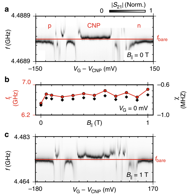
Fig. 3 Dispersive shift as a function of V_G and B_{||} . a At B_{||} = 0 T, |S_{21}| (Norm.) versus f and V_G (with V_{CNP} = 300 mV subtracted) shows the symmetric band dispersion of graphene with additional fluctuations we attribute to UCF. b f_t (red circles) extracted from \chi (black diamonds) versus B_{||} at V_G = 0 V, showing f_t is not significantly affected. c Repeating a at B_{||} = 1 T with V_{CNP} = 430 mV subtracted confirms the graphene JJ behaves equivalently to B_{||} = 0 T. The variation observable in b and shift in V_{CNP} between a and c we attribute to slow gate drift
