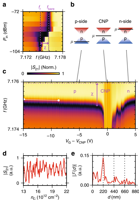
Fig. 2 Resonator spectroscopy as a function of P_{in} and V_G . a |S_{21}| (Norm.) as a function of input frequency f and input power P_{in} . At single photon occupancy the resonator experiences a frequency shift \chi due to repulsion from an energy level above the resonator (device A). b Diagram of the Dirac cone band structure of graphene. Changing V_G to tune \mu allows the dominant charge carriers to be varied between hole, charge neutral and electron-like regimes. c At single photon occupancy, |S_{21}| (Norm.) is measured as f and V_G are varied, with the voltage at CNP ( V_{CNP} = 7.8 V) subtracted. In the p-regime, \chi oscillates as V_G is varied. We extract the charge carrier density n_C d from the white linecut to generate a Fourier transform e that is consistent with Fabry-Perot oscillations in a cavity of d = 220 nm
