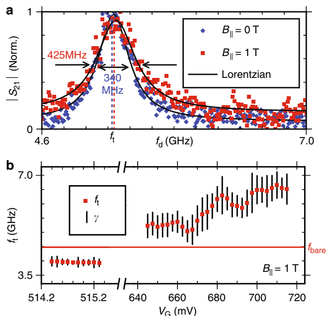
Fig. 4 Two tone spectroscopy a Normalised |S_{21}| at f_r as f_d is varied can be fitted to extract f_t and \gamma at V_G = 0 V. At B_{||} = 1 T, \gamma shows a 25% increase compared to B_{||} = 0 T. b At B_{||} = 1 T, f_t and \gamma are extracted as V_G is varied, demonstrating f_t can be swept over a wide frequency range. Lines bisecting each f_t are not error bars, but represent the extracted \gamma at each f_t
