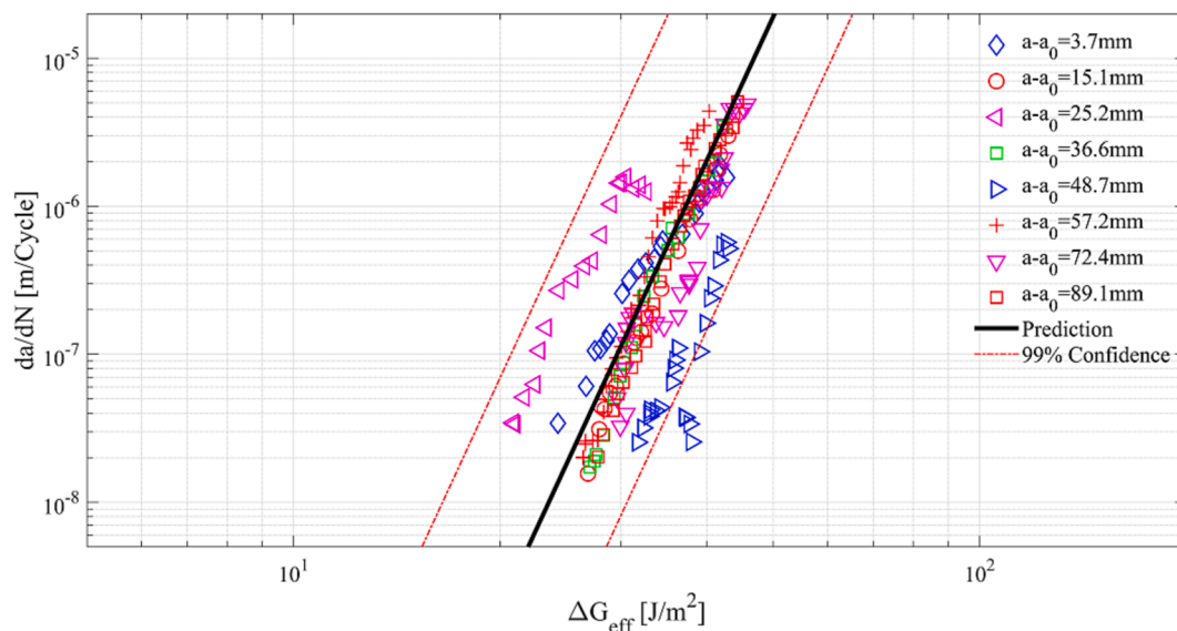
Fig. 18. FDG behavior predictions of 50°C.
