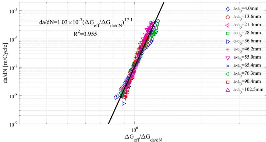
Fig. 14. FDG interpretations of -40^{\circ}\text{C} via the semi-empirical fatigue model.
