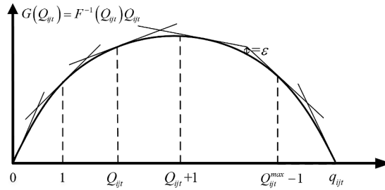
Fig. 2. Outer-approximation procedure.
