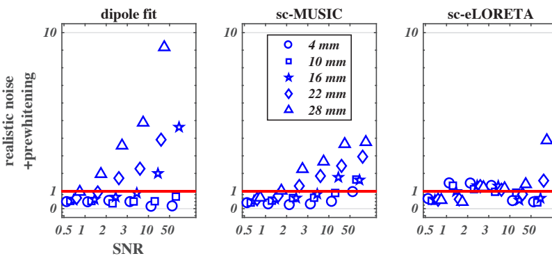
Fig. 3.3. Separability as a function of SNR. Values lower than one imply that the dipoles were not separable due to the large standard deviation. The different symbols represent the different spatial distances between the simulated dipoles. The rows show the results for the tested algorithms: stationary dipole fit, sc-MUSIC, sc-eLORETA when spatial pre-whitening is applied on the realistic noise case. The temporal distance of \Delta=30 ms is shown.
