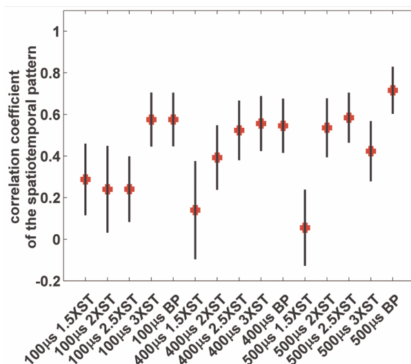
Fig. A2.1 Correlation coefficient of the spatiotemporal patterns for the time window 25 to 65 ms post stimulus and for different stimulation protocols. Mean and standard deviation over the bootstrapped based correlations are shown.
