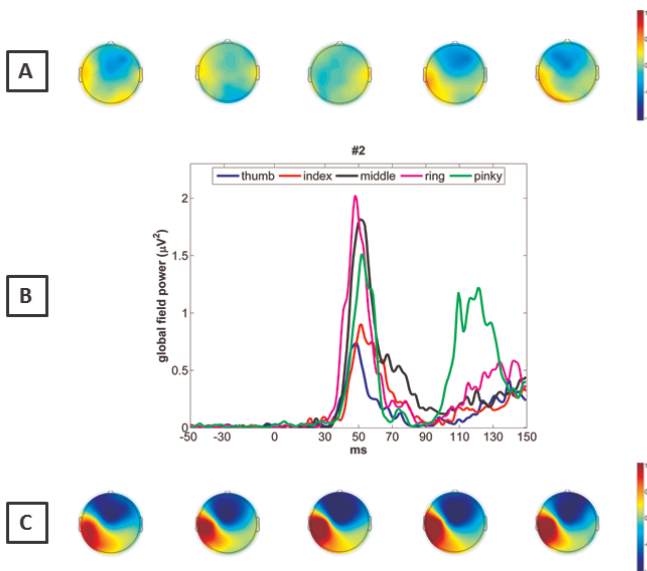
Fig. A2.3 (A) topographical distribution of the P30 peak. (B) GFPs of SEP responses after stimulation of the individual fingers of subject 2. Different colors represent different fingers. (C) topographical distribution of the P50 peak.
