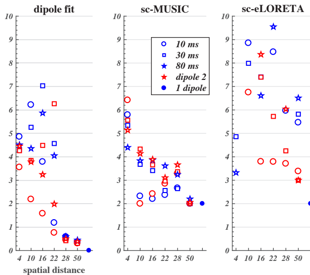
Fig. S3.1 Mean distance from simulated dipole(s). Comparison of one dipole simulation versus two dipoles simulation for the ideal case of added white noise and SNR = 50 . The black line depicts the grid size (3 mm). The different symbols represent the different temporal distances of the sources time-series peaks.
