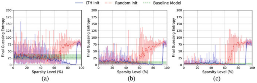
Fig. 16 CHES CTF 2018, MLP8. (a) 20,000 profiling traces. (b) 30,000 profiling traces. (c) 40,000 profiling traces
