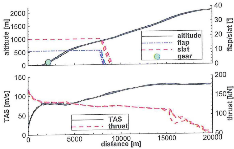
(a) Standard departure flights.
