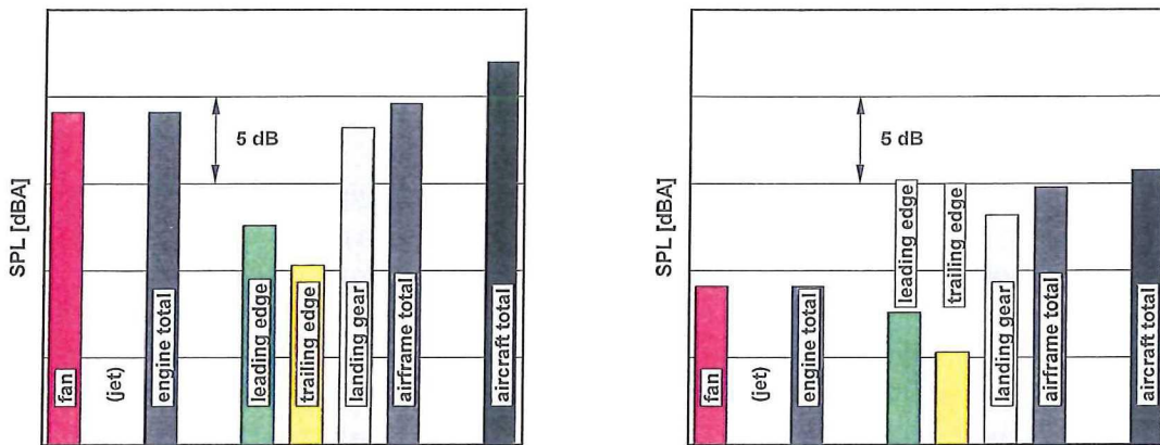
(a) Reference vehicle.
