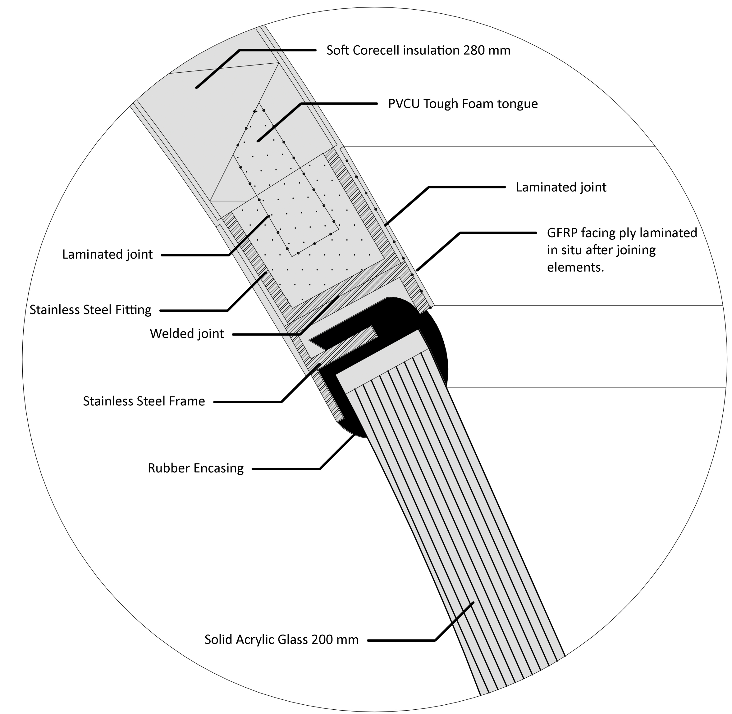
Detail B
