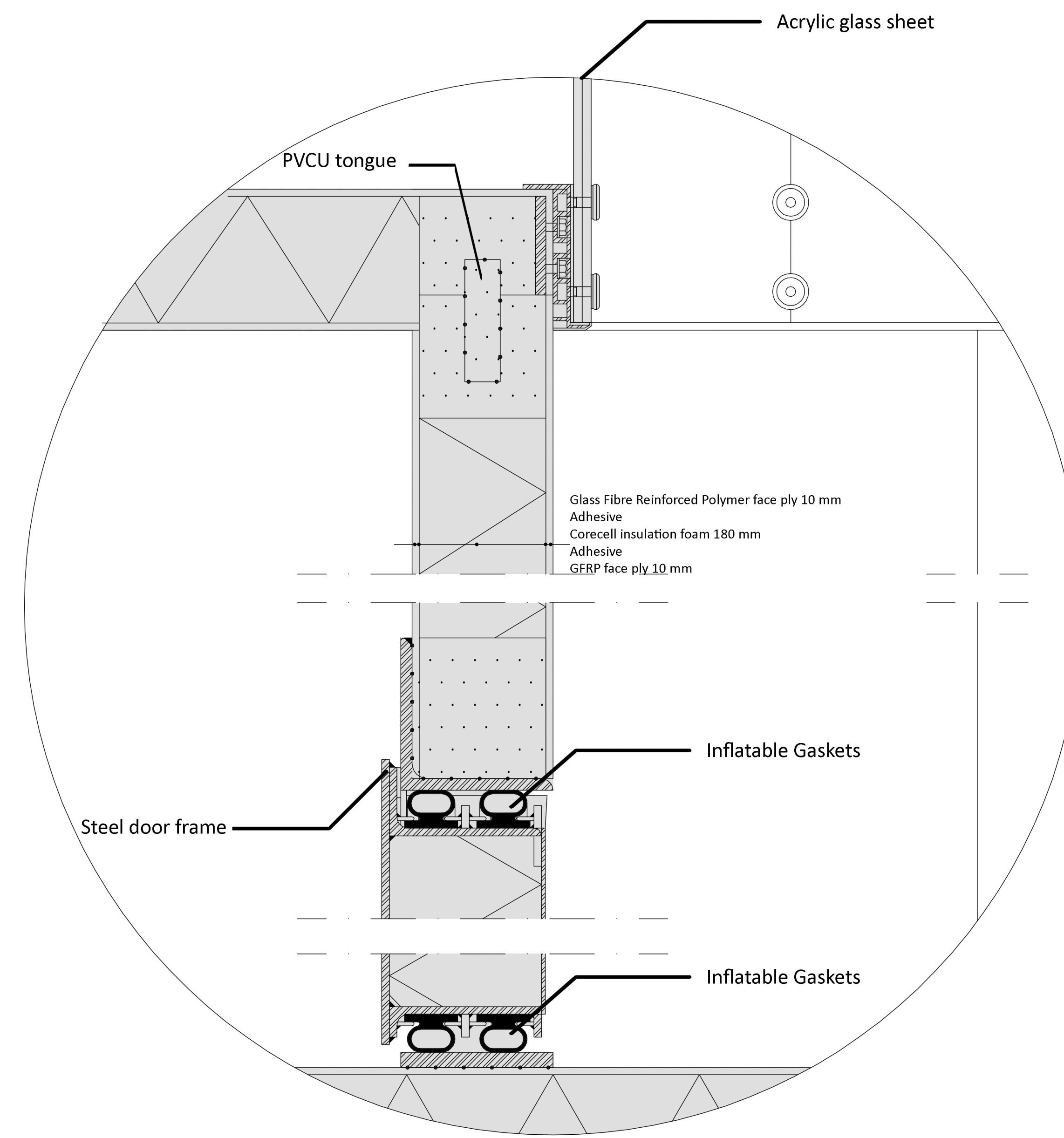
Detail A
