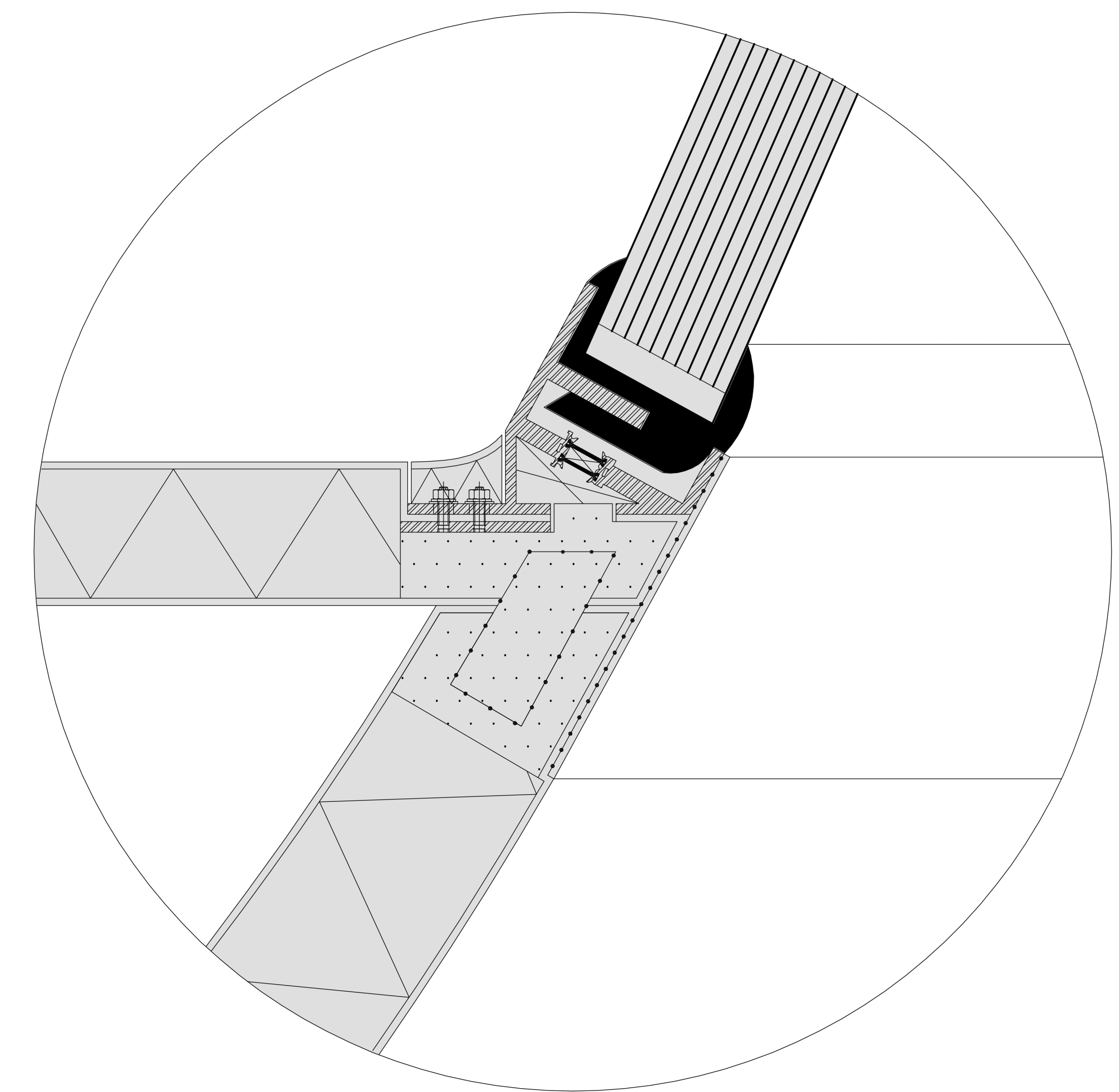
Detail D
