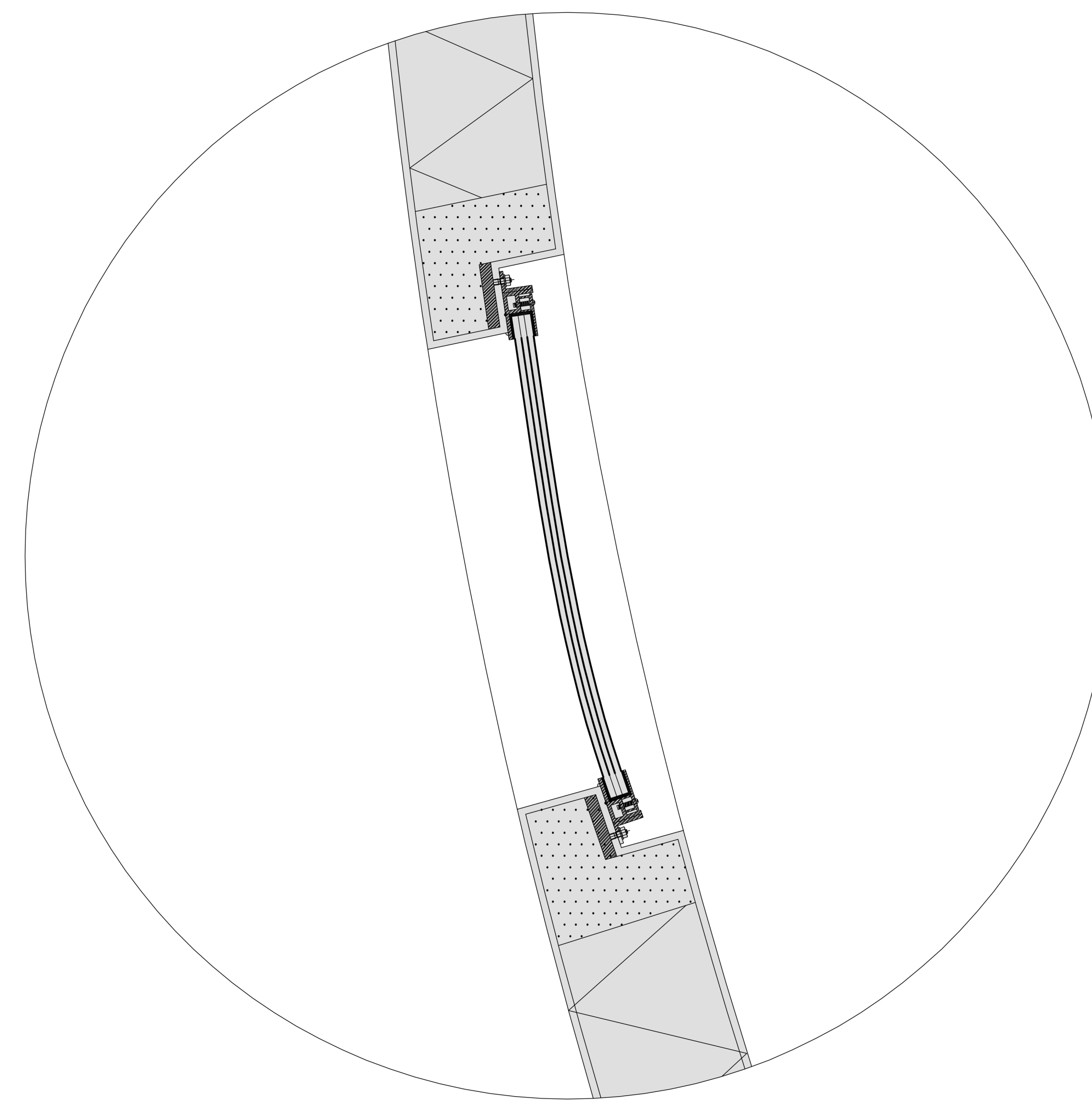
Detail C
