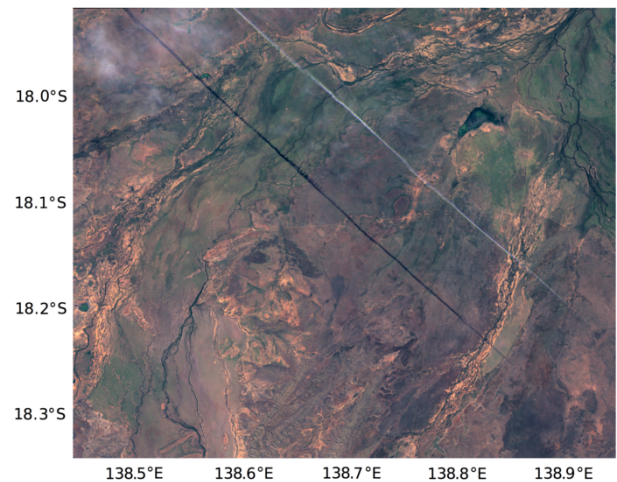
Figure 1. LANDSAT 8 True Colour RGB on April 4 th 2017, West Queensland in Australia, with contrail visible as white diagonal stripe and the shadow it casts above to the South.
