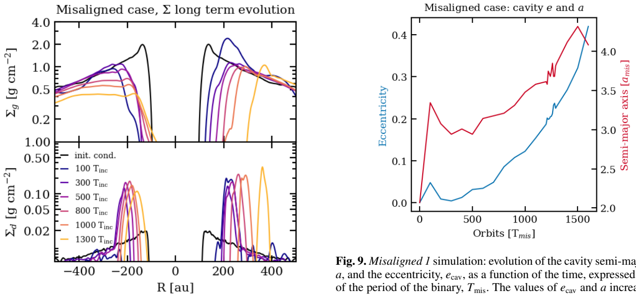
Fig. 8. Misaligned I case: radial cut along the major axis of the surface density profile of the gas (top, \Sigma_g ) and dust (bottom, \Sigma_d ) as a function of the distance of the star, R (au), for different time-steps. Initially, a low-eccentric ( e_{\text{cav}} \lesssim 0.03 ) cavity and dust ring form. Later on, the simulation shows a larger and more eccentric cavity and dust ring.
