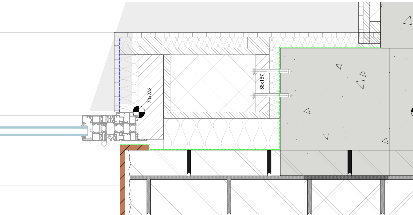
DT-H02 - French balcony horizontal cut
