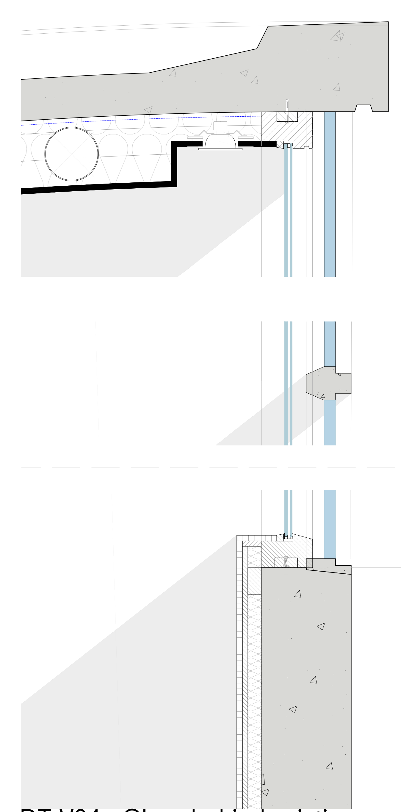
DT-V04 - Glass behind existing window frame, curved insulation
