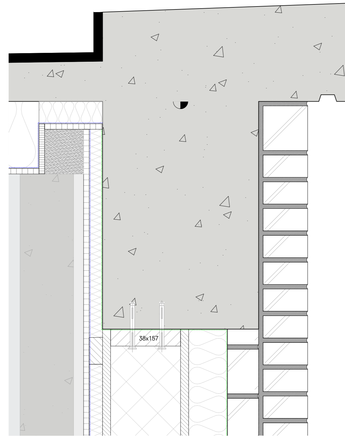
DT-V03 - Ceiling bay to hide lighting fixtures
