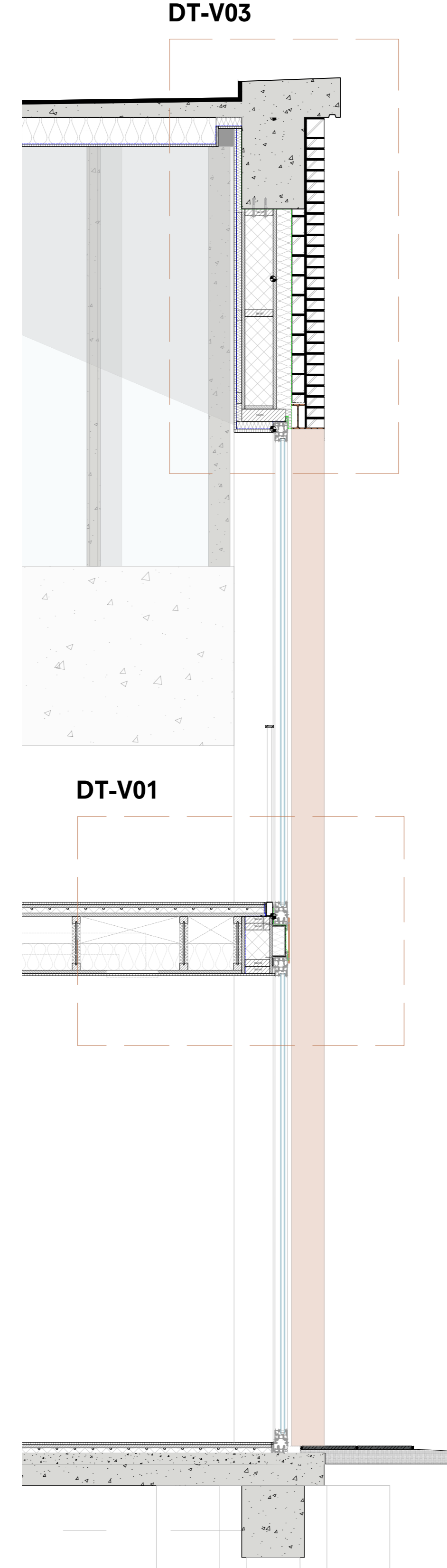
Eastern façade cut
