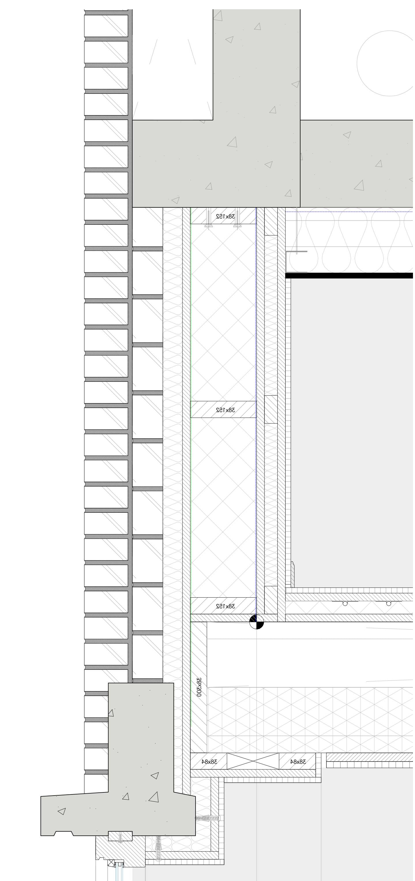
DT-V05 - Timber framing and finjoists
