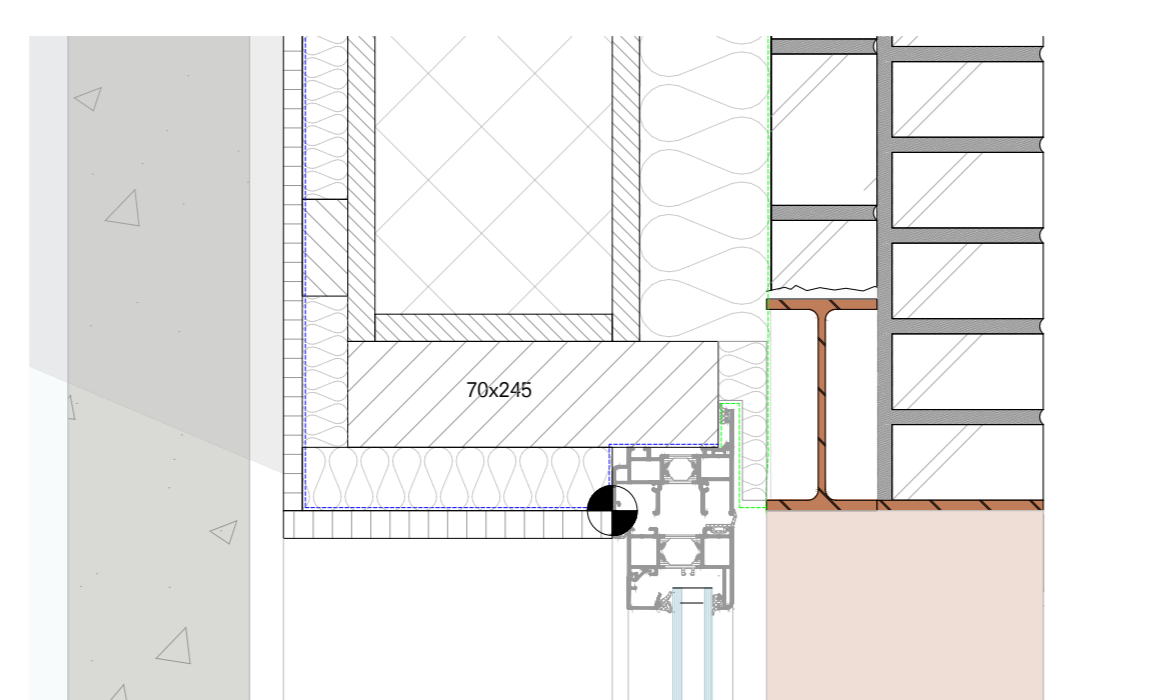
DT-V03 - IPE-beam welded flange
