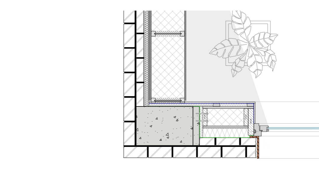
Ground floor horizontal section
