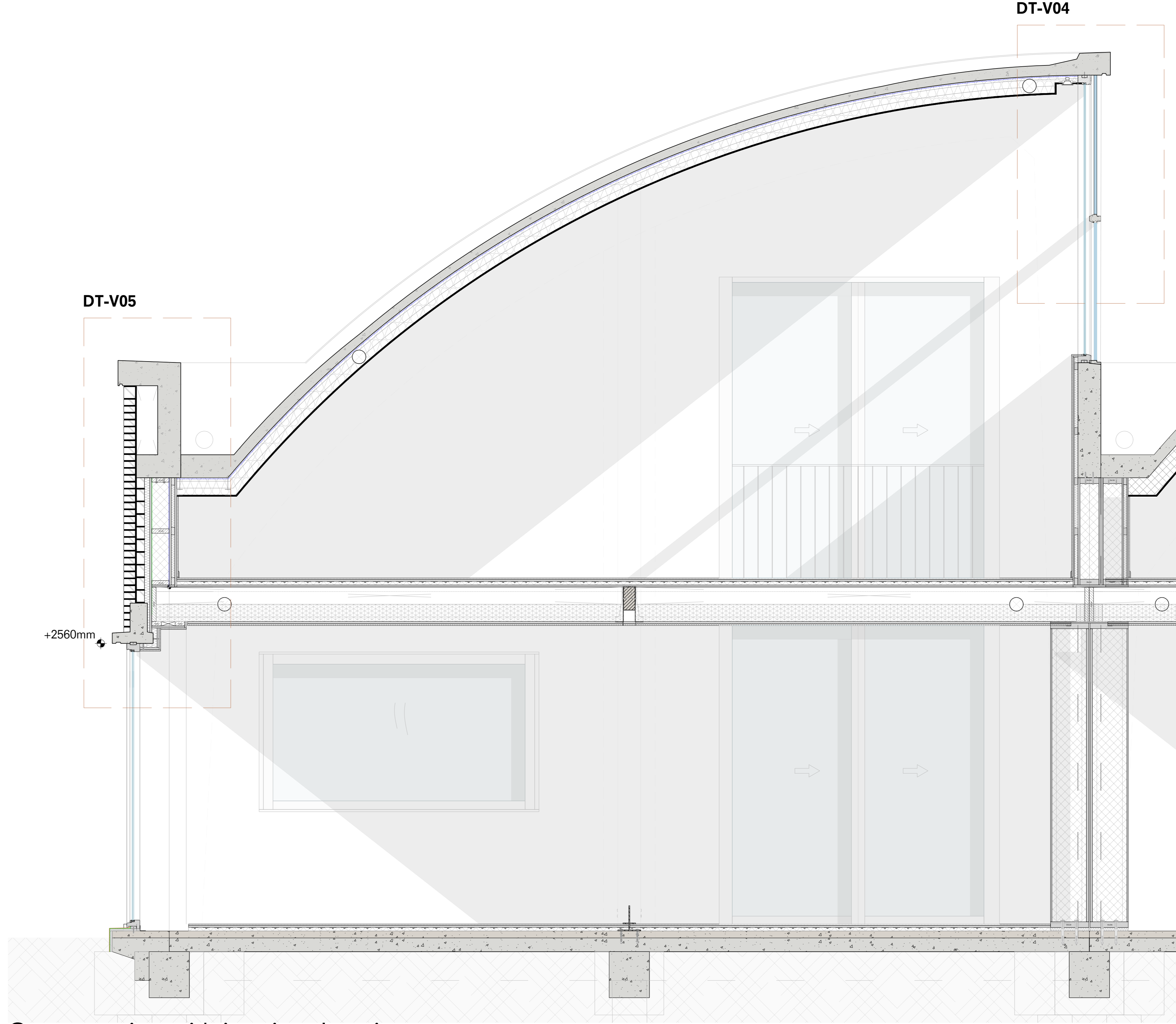
Cross section with interior elevation
