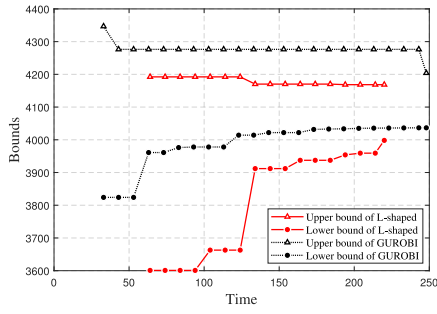
(a) Instance with (|I|, |K|, |T|) = (10, 15, 140)
