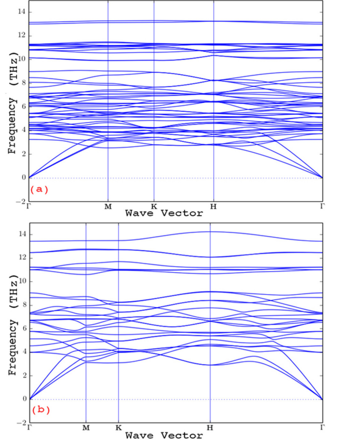
FIG. 2. Phonon band structure of \text{MnFeSi}_{0.33}\text{P}_{0.66} in (a) AFM and (b) FM states.
