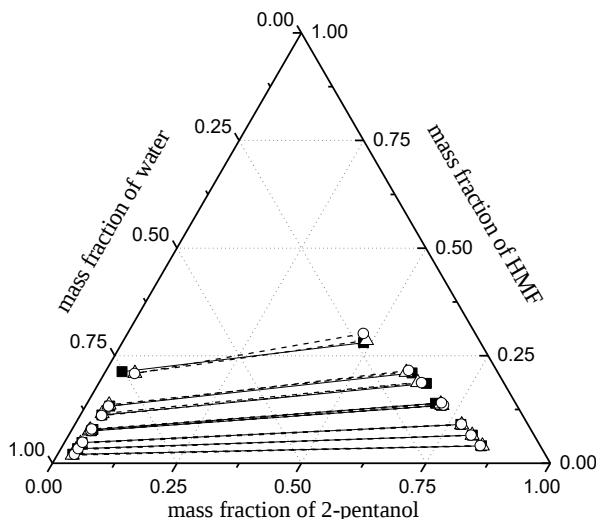
Figure 2.2 Phase diagram of the experimental and calculated LLE tie-line data for the ternary system 2-pentanol-HMF-water at T = 313.15 K and atmospheric pressure using NRTL and UNIQUAC models; (—■—) experimental data; (---△---) NRTL model; (---○---) UNIQUAC model.
