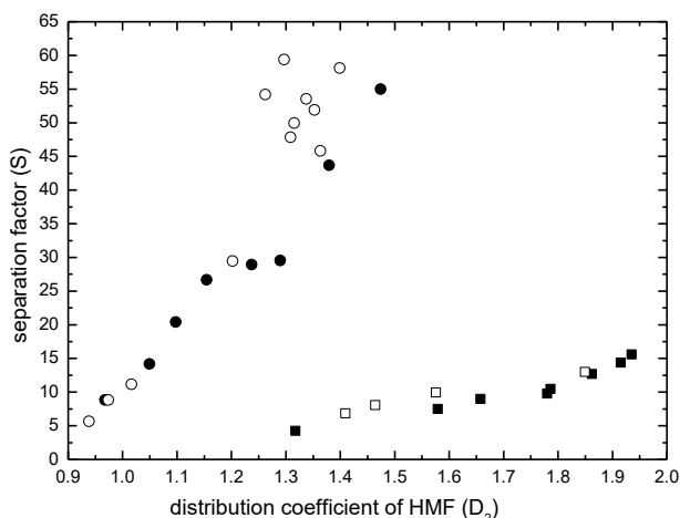
Figure 2.3 Relationship between separation factor (S) and distribution coefficient of HMF ( D_2 ) for the organic solvent-HMF-water systems at T = 313.15 K and 298.15 K, and atmospheric pressure; (●) MIBK-HMF-water at 313.15 K (this study); (○) MIBK-HMF-water at 298.15 K [19]; (■) 2-pentanol-HMF-water at 313.15 K (this study); (□) 2-pentanol-HMF-water at 298.15 K [23].
