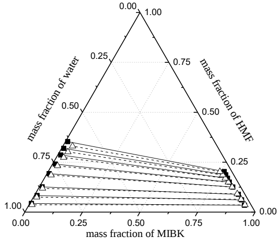
Figure 4.1 Phase diagram of the experimental and calculated LLE tie-line data for MIBK-HMF-water and MIBK-HMF-water-DES (ChCl-urea) systems on DES-free basis at T=313.15 K and atmospheric pressure (0.1 MPa) using NRTL model; (a) 0 wt% DES [22]; (b) 10 wt% DES; (c) 20 wt% DES; (d) 30 wt% DES; —■— : experimental data; --△-- : NRTL model.
