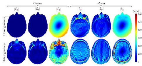
Figure 2: Magnitude of the electric field strength component at two positions in the birdcage coil (for the midplane, (a-c) and five centimeters above the midplane (d-f)) and for a longitudinal homogeneous head (model B, top row) and heterogeneous head (model A, bottom row).
