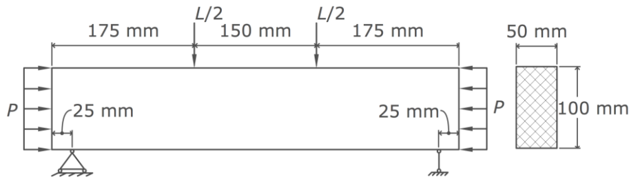
Figure 8. Test model dimension and load combination
