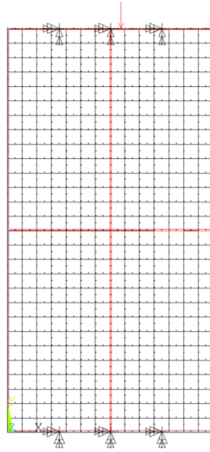
Figure 27 FEM model
