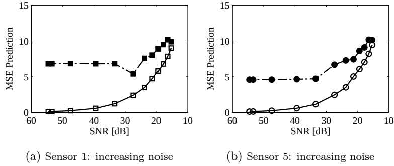
Figure 8: One-step ahead prediction error of sensors 1 and 5 for the increasing noise variance. The solid lines correspond to the full models and the dashed lines to the reduced models.
