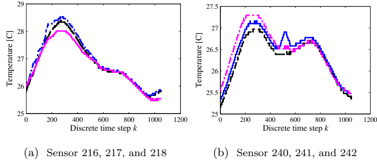
Figure 20: Validation data plot from sensor: (a) 216 in black, 217 in blue), 218 in magenta (b) 240 in black, 241 in blue, and 242 in magenta.
