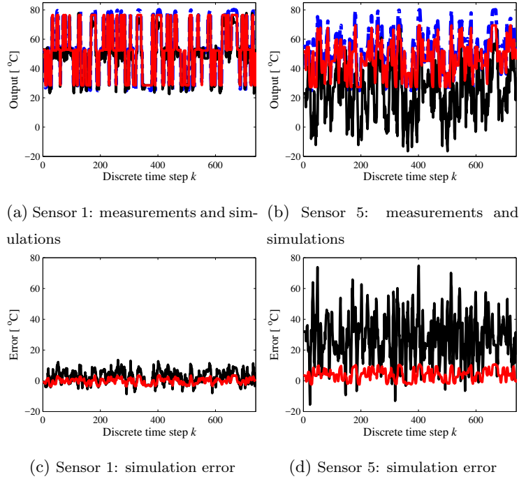
Figure 6: Measurements (blue) and free-run simulation predictions for the models with full inputs (black) and the ones with reduced inputs (red) using the validation data set for the two-dimensional heat conduction example. Note that the output error of the full and the reduced input models are overlapping.
