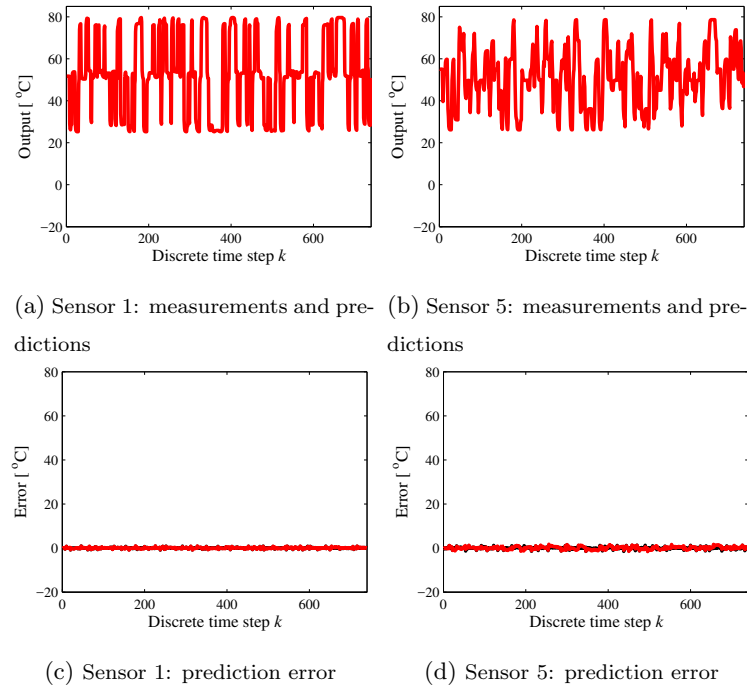
Figure 5: Measurements (blue, invisible due to the overlap) and one-step ahead prediction for the models with full inputs (black curves) and the ones with reduced inputs (red curves) using the validation data set for the two-dimensional heat conduction example. Note that the prediction error of the full and the reduced input models are overlapping.
