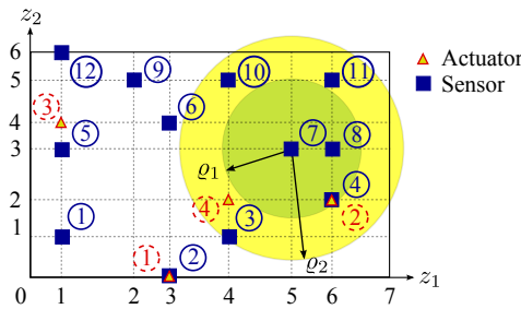
Figure 1: An illustration of the neighboring measurements and the inputs set with two possible neighborhoods of sensor 7 using a Euclidean distance criterion. The first set of neighbors is defined using distance \varrho_1 from sensor 7 and the second set using distance \varrho_2 .
