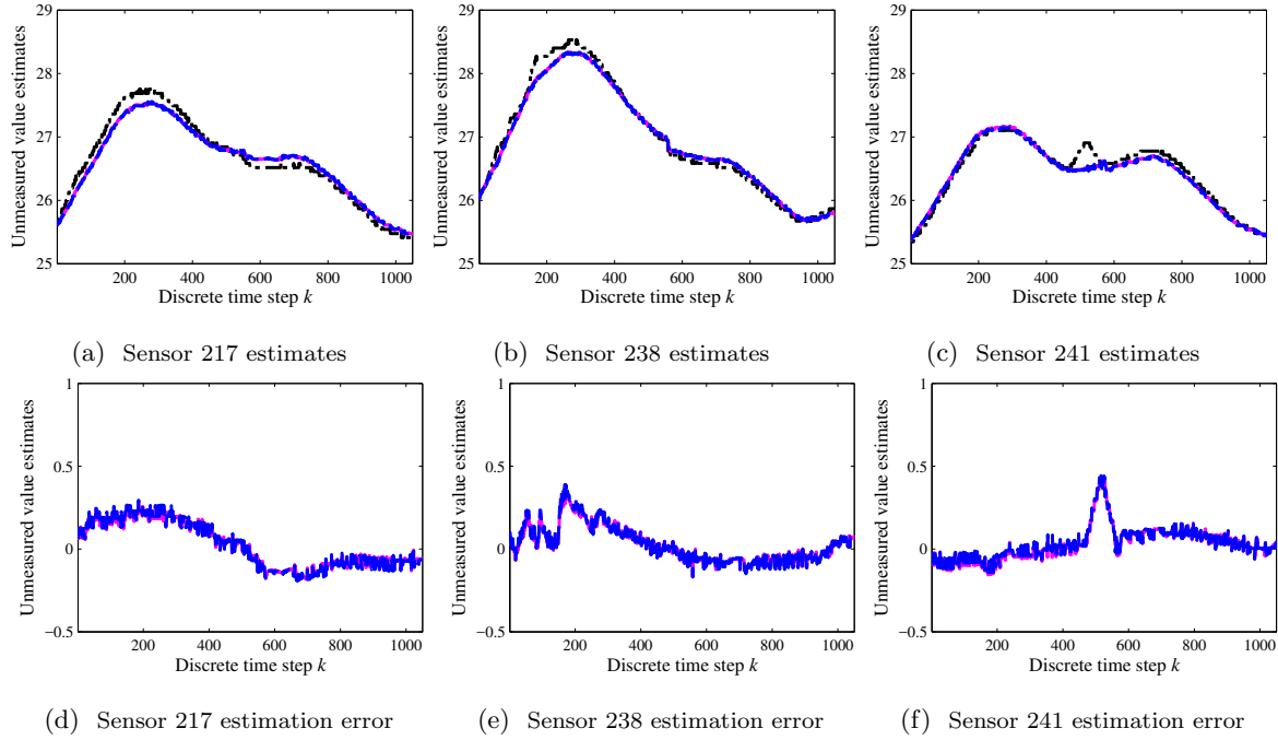
Figure 17: Validation data estimates for sensor 217, 238, and 241 by using ordinary kriging and their corresponding error. For (a), (b), and (c), black lines are the validation data, magenta lines are estimates from the full models, and blue lines are estimates from the reduced models. For (d), (e), and (f), magenta lines are errors from the full models and blue lines are errors from the reduced models.
