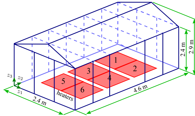
Figure 11: A schematic representation of the greenhouse with its physical dimensions.
