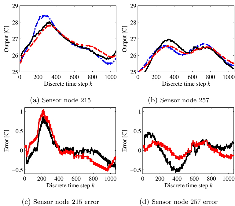
Figure 15: Greenhouse setup measurements (blue) and 20-step-ahead predictions for the model with the full set of inputs (black) and for the model with the reduced set of inputs (red) using the centered validation data set and their corresponding prediction error, i.e., error for the full model (black) and for the reduced model (red). Note that the measurement, the prediction of the full and the reduced input models are very close one to another.
