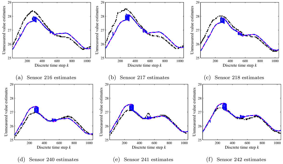
Figure 18: Validation data estimates for sensor 216, 217, 218, 240, 241, and 242 by using ordinary kriging. Black lines are the validation data, magenta lines are estimates from the full models, and blue lines are estimates from the reduced models.
