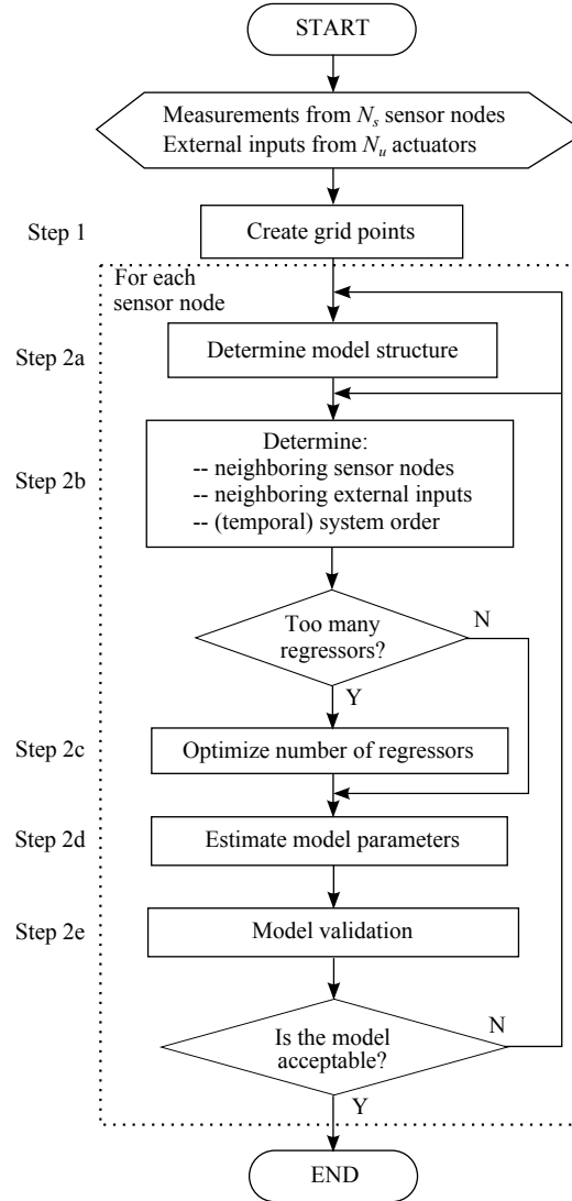
Figure 3: Flow chart of the proposed method.
