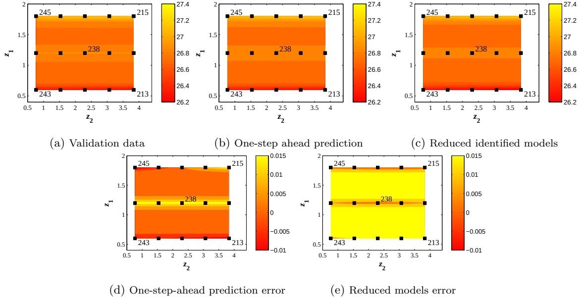
Figure 21: Contours of the greenhouse temperature model at discrete-time step k = 400 of the validation data for 0.6 \geq z_1 \geq 1.8 , 0.767 \geq z_2 \geq 3.833 and fixed z_3 = 1.1 . The black square markers are the sensor locations and the labeled sensors are used to build the kriging model.
