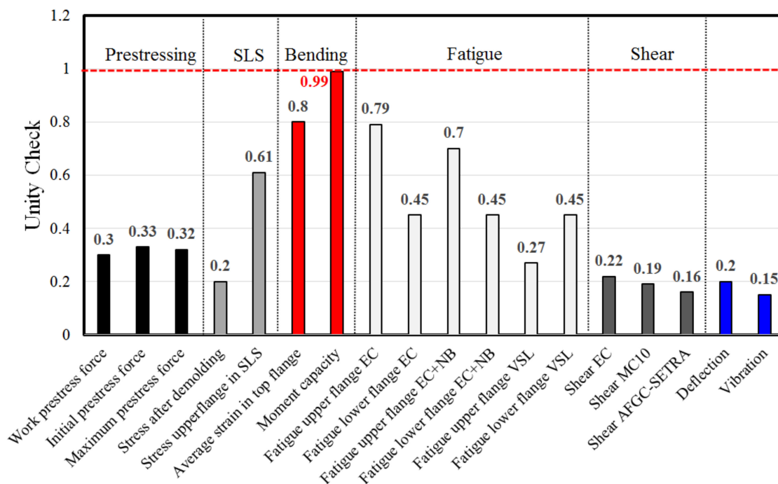
Figure 9. Outcome of the calculation with BoDeTo (ULS bending criteria is reached).
