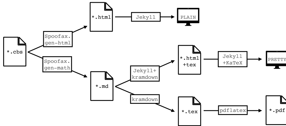
■ Figure 2 Generation of hyperlinked twins using Spoofax and external tools.
