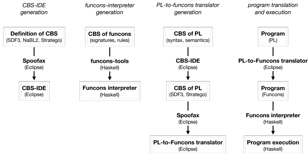
■ Figure 1 Generation and use of a CBS-IDE based on Spoofax and external tools [16].
