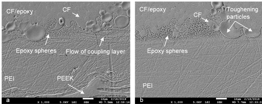
Fig. 4. Representative SEM cross-sectional micrographs of epoxy-PEEK 250 samples welded at a displacement of a) 0.38 mm and b) 0.30 mm. The epoxy-PEI interphase seems intact when samples are welded at d_{\text{opt}} whereas flow of the coupling layer close to the epoxy resin, leading to alteration of the original interphase morphology is observed when the samples are welded above d_{\text{high}} .
