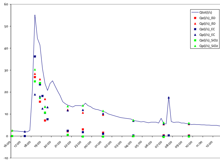
Fig. 3. Hydrograph separation between event ( Q_e ) and pre-event ( Q_p ) discharge of the 27 March 2008 event based on \delta D , EC and SiO_2 in Mataini catchment.
