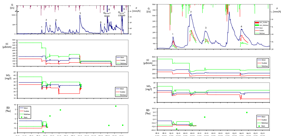
Fig. 4. Time series of precipitation [ mm\ h^{-1} ], discharge [ l\ s^{-1} ], EC [ \mu S\ cm^{-1} ], SiO_2 [ mg\ l^{-1} ] concentration and \delta D [%] content at the weir site in Bangalala and Vudae and Ndolwa catchments for the Vuli '07 season and 18–25 November 2007 events.
