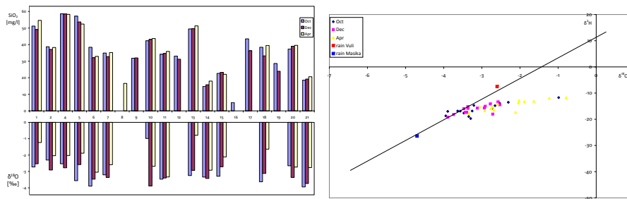
Fig. 8. Inter-seasonal variations of \text{SiO}_2 [ \text{mg l}^{-1} ] concentrations and \delta^{18}\text{O} [‰] content in selected springs (see Fig. 1 for locations).
