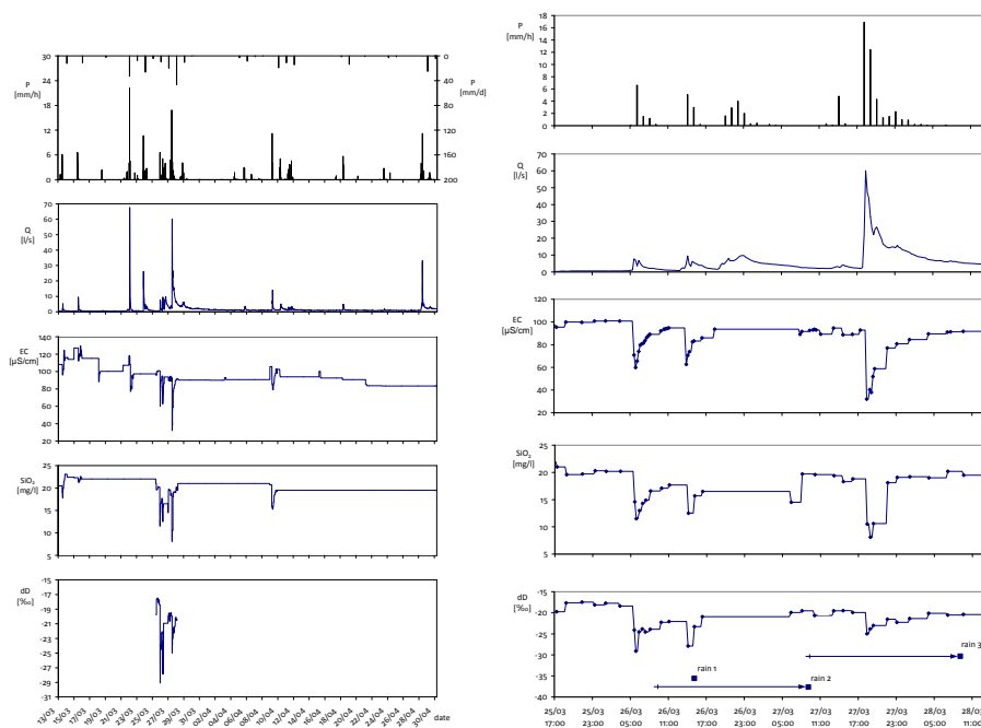
Fig. 2. Time series of precipitation [ \text{mm h}^{-1} and \text{mm d}^{-1} ], discharge [ \text{l s}^{-1} ], EC [ \mu\text{S cm}^{-1} ] and \text{SiO}_2 [ \text{mg l}^{-1} ] concentration and \delta D [%] content in runoff for Mataini catchment, 12 March–30 April 2008 and 25–28 March 2008.
