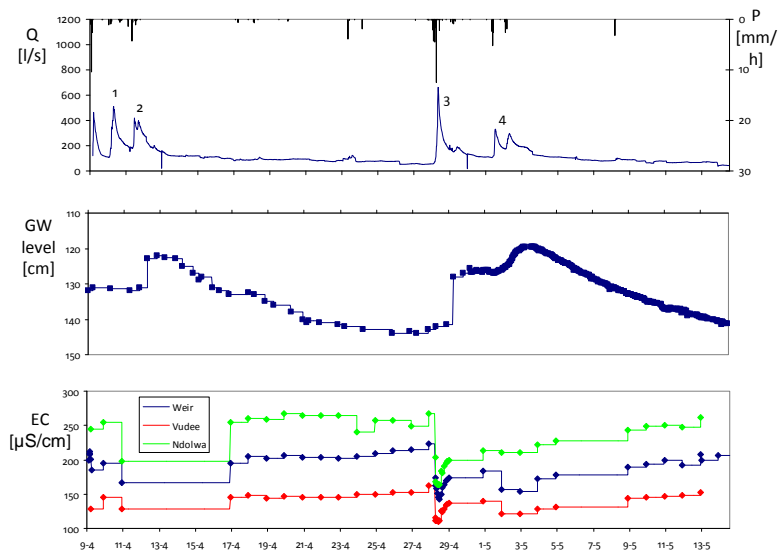
Fig. 5. Time series of precipitation [ \text{mm h}^{-1} ], discharge [ \text{l s}^{-1} ], EC [ \mu\text{S cm}^{-1} ], \text{SiO}_2 [ \text{mg l}^{-1} ] concentration and \delta D [‰] content at the weir site in Bangalala and Vudee and Ndolwa catchments for the Masika '08 season.
