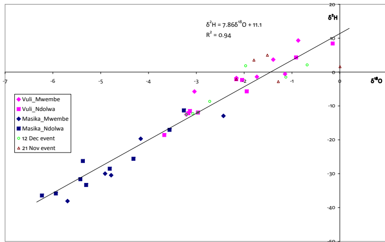
Fig. 7. Seasonal variation in isotopic composition of rainfall, based on measurements at 2 stations and during two events (21 November and 12 December 2007).
