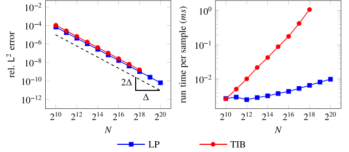
FIG. 3. The figure shows a comparison of the algorithms LP and TIB for the secant-hyperbolic potential ( A_R = 0.4 ) with respect to convergence rate (left) and run time per sample (right).
