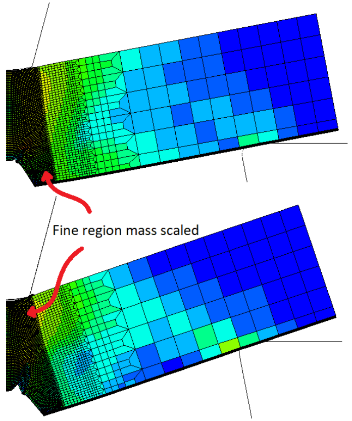
FIGURE 6: CONTOURS OF MISES STRESS SHOWING THE LOAD PATH CHANGING ITS COURSE TO PREDOMINANTLY PASS THROUGH A DIFFERENT NODE THAN BEFORE, SHORTENING THE SPAN.
