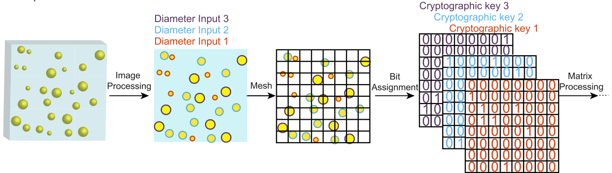
Fig. 2. Schematic illustration of working algorithm. Cryptographic keys are generated from a diameter-based PUF authentication system using (a) single diameter and (b) multiple diameters as input. Following proper mesh and bit assignment, the cryptographic key, i.e. the output response matrix is further processed depending on the bit uniformity.
