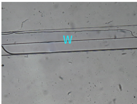
Figure 5.2: A mixed regime is observed in a step channel when initialized at a high flow rate. The dyed fluid is water (the regions corresponding to the letter W within the interface) and the colourless fluid is Novec.
