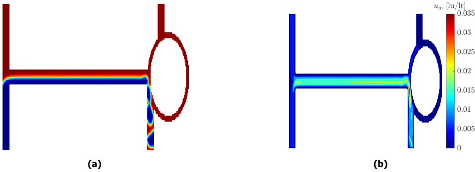
Figure 4.23: a) Droplets were observed in the toluene outlet in the circular reservoir design ( 600 \mu m diameter) with a concentric pillar of 500 \mu m diameter. The Capillary number of toluene is 10^{-3} and \phi = 1 . The blue fluid is toluene and the red fluid is water. b) Velocity magnitude for the same simulation with the units in lattice unit/lattice time ( lu/lt ).
