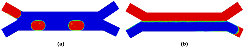
Figure 5.10: VOF simulations for Water-Novec mixture in channel 2 at Ca_n = 1.5 \times 10^{-5} , Ca_w = 3 \times 10^{-5} with a) Hydrophobic surface. b) Hydrophilic surface. The blue fluid is Novec and the red fluid is water, with Novec being located in the deeper section at the bottom half of the channel.
