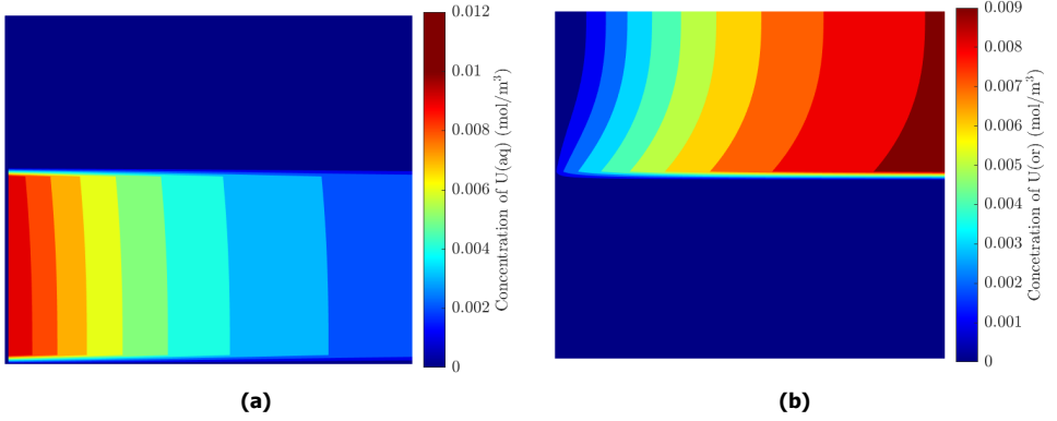
Figure 6.2: Simulated concentration profiles using the data from Helle et al [9] at Q_{aq} = 1.56 \mu\text{L/min} and Q_{org} = 1.38 \mu\text{L/min} . a) Aqueous Concentration Profile b) Organic Concentration Profile
