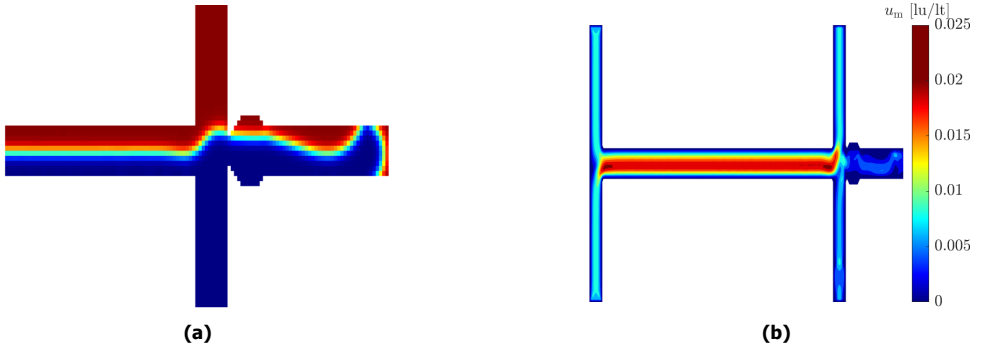
Figure 4.7: a) Simulations of a T-T channel with D_1 = 70 \mu\text{m} , D_2 = 140 \mu\text{m} and D_3 = 100 \mu\text{m} . The Capillary number of toluene is 10^{-3} and \phi=1 . The blue fluid is toluene and the red fluid is water. b) Velocity magnitude contour for the same simulation in \text{lu/lt} .
