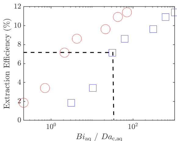
Figure 6.13: Influence of the Biot number (blue squares) on the Gallium extraction efficiency in the step channel. The Biot number is varied by changing K_1 (ranging from 3 \times 10^{-6} to 10^{-3} m/s) at a flow rate of 10 \mu\text{L/min} . The Da_c (red circles) is also plotted for the same Biot numbers.
