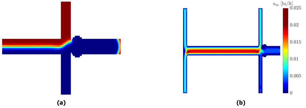
Figure 4.8: a) Simulations of a T-T channel with D_1 = 90 \mu\text{m} , D_2 = 140 \mu\text{m} and D_3 = 100 \mu\text{m} . The Capillary number of toluene is 10^{-3} and \phi=1 . The blue fluid is toluene and the red fluid is water. b) Velocity magnitude contour for the same simulation in \text{lu/lt} .
