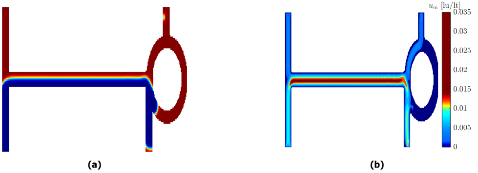
Figure 4.22: a) Stable parallel flow in the circular reservoir design (600 \mu\text{m} diameter) with a concentric pillar of 400 \mu\text{m} diameter. The Capillary number of toluene is 10^{-3} and \phi = 0.45 . The blue fluid is toluene and the red fluid is water. b) Velocity magnitude for the same simulation with the units in lattice unit/lattice time (lu/lt).
