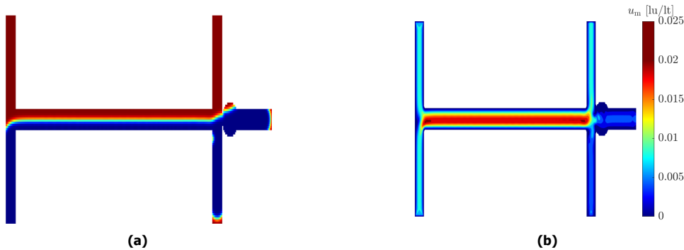
Figure 4.9: a) Simulations of a T-T channel with D_1 = 70 \mu\text{m} , D_2 = 160 \mu\text{m} and D_3 = 100 \mu\text{m} . The Capillary number of toluene is 10^{-3} and \phi=1 . The blue fluid is toluene and the red fluid is water. b) Velocity magnitude contour for the same simulation in \text{lu/lt} .
