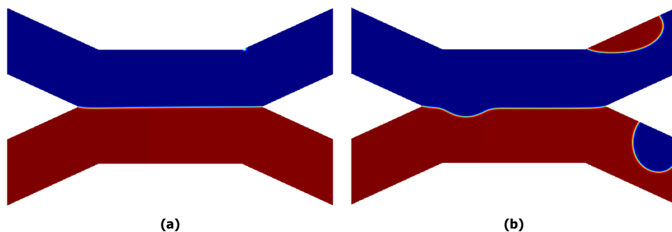
Figure 6.12: RK simulations of Zinc Nitrate solution and chloroform in a step channel at Q = 20 \mu\text{L/min} . a) Phase Contour at t=3.7 ms. b) t= 0.26 s
