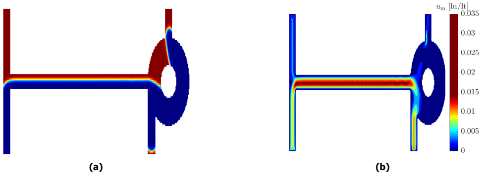
Figure 4.21: a) Leakage in the circular reservoir design (600 \mu\text{m} diameter) with a concentric pillar of 200 \mu\text{m} diameter. The Capillary number of toluene is 10^{-3} and \phi = 0.45 . The blue fluid is toluene and the red fluid is water. b) Velocity magnitude for the same simulation with the units in lattice unit/lattice time (lu/lt).
