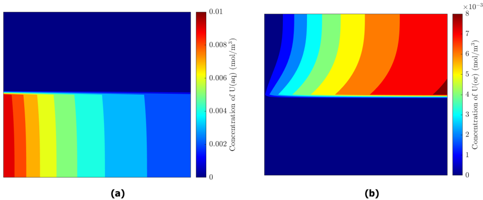
Figure 6.3: Simulated concentration profiles using the data from Helle et al [9] and the analytical flow profile defined in Equation 6.13. Q_{aq} = 1.56 \mu\text{L}/\text{min} , h = H/2 , Bi_{aq} = 0.16 , Bi_{or} = 1.6 , Pe_{aq} = 0.081 , Pe_{or} = 0.78 . a) Aqueous Concentration Profile b) Organic Concentration Profile
