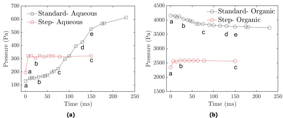
Figure 5.14: Evolution of the pressure in the a) Aqueous phase b) Organic phase in both the channels. The letters in the plot correspond to the times shown in Figures 5.12 and 5.13.
