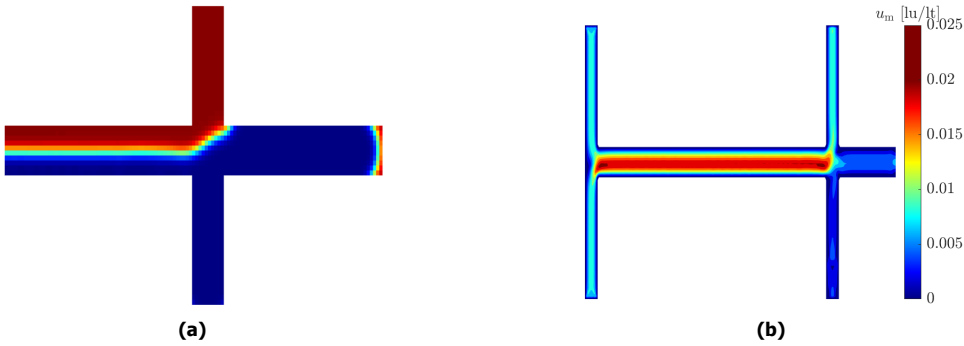
Figure 4.12: a) Simulations of a T-T channel with a third outlet similar to the design shown in Figure 4.2a [5]. The Capillary number of toluene is 10^{-3} and \phi=1 . The blue fluid is toluene and the red fluid is water. b) Velocity magnitude contour for the same simulation in lu/lt.
