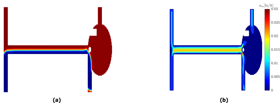
Figure 4.16: a) Stable parallel flow in the T-T channel at \phi = 1.2 when the circular reservoir contains two pillars. The blue fluid is toluene and the red fluid is water, with the Capillary number of toluene being 10^{-3} . b) Velocity magnitude for the same simulation with the units in lattice unit/lattice time (lu/lt).
