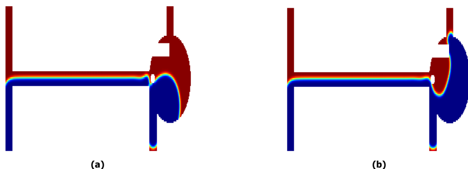
Figure 4.15: Stages of accumulation leakage in a circular reservoir with two pillars at a) t = 7 ms and b) t = 20 ms. The blue fluid is toluene and the red fluid is water, with the Capillary number of toluene being 10^{-3} and \phi = 0.6 .
