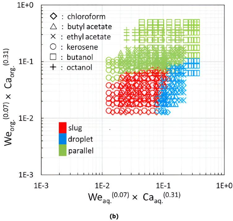
Figure 1.5: a) Flow Maps showing Re_c/Ca_c as a function of Re_d d_h / \epsilon_d for different studies [24] b) Flow patterns observed by Asadi-Sanghadi et al. [61] for various fluids using a combination of Ca and We
