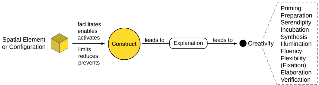
Figure 50. Abstracted “formula” that describes the causal relationship between space and creativity.
