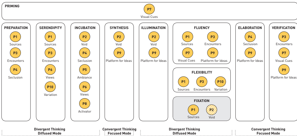
Figure 62. Propositions relevant to the creativity concepts.
