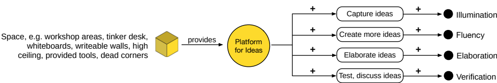
Figure 59. Components of Proposition 9: “Platform for Ideas”.
