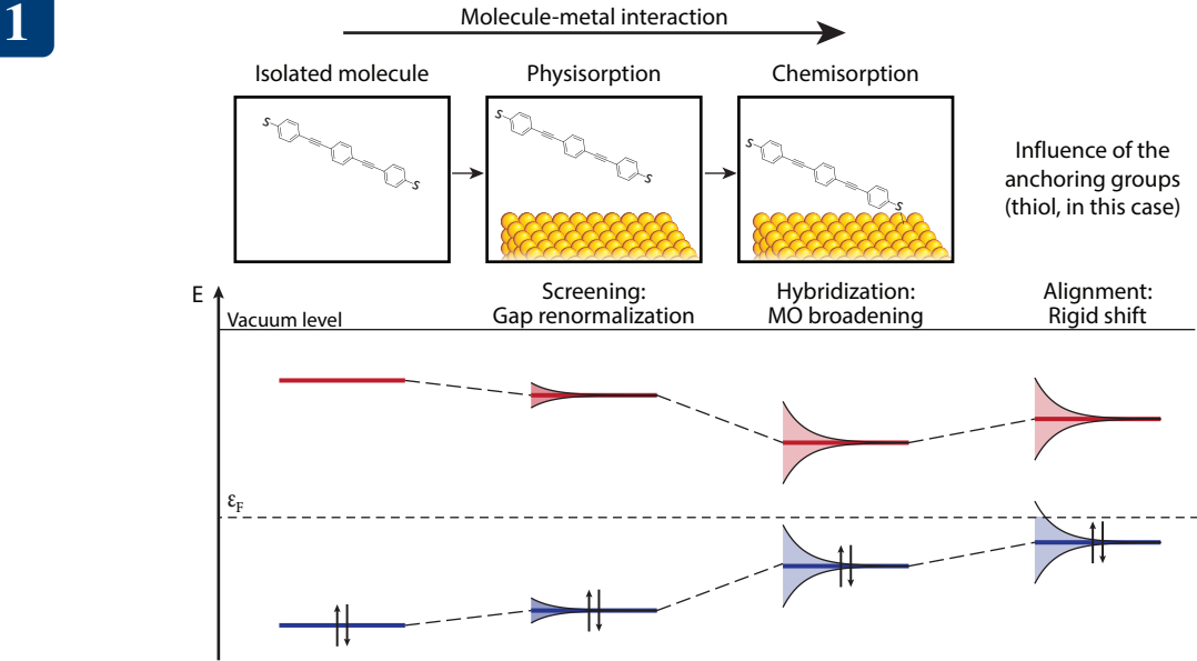
Figure 1.2: Schematic drawing of the effect of the interaction between a molecule and a metal on the frontier molecular orbitals in respect to the Fermi energy ( \epsilon_F ) of the metallic surface. The isolated molecule (left) initially interacts with the metal surface only via long-range interactions (middle, physisorption) and subsequently also with a chemical bonds (right, chemisorption). The screening of the metal surface causes the energy gap to reduce, the formation of the chemical bond induces the broadening of the MOs and their hybridization with the wavefunction of the metal. The formation of a surface dipole causes the levels to rigidly shift towards higher or lower energies, depending on the electronegativity of the anchoring groups.
