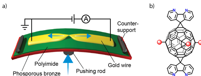
Figure 3.1: a) Schematics of the MCBJ devices used in the experiment [165]. b) Chemical structure of the trans -1-bis-diazafluorene adduct of C_{60} -tetramalonate ( C_{60} -daf). Malonates are designated with red balls representing the C(COOC_2H_5)_2 groups.
