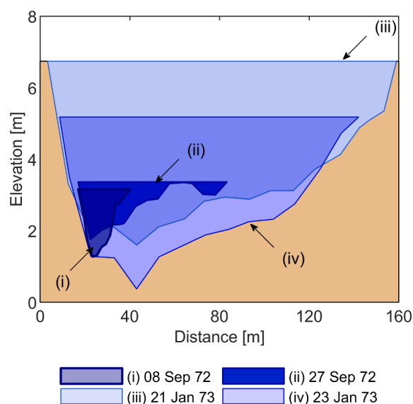
Fig. 2. Channel cross-section A, looking in the downstream direction, at Misiones La Paz measured in the period 1972–1973 showing strong and quick morphological variations in time. The corresponding discharges are: (i) 12 \text{ m}^3/\text{s} ; (ii) 25 \text{ m}^3/\text{s} ; (iii) 1,330 \text{ m}^3/\text{s} ; and (iv) 550 \text{ m}^3/\text{s} . Discharge and cross section geometries data were obtained from the Tri-national Committee for the Development of the Pilcomayo River basin ( www.pilcomayo.net ). Their measuring technique is well described in Martín-Vide et al. (2019).
