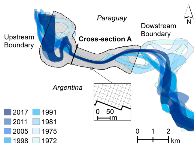
Fig. 3. Changes of river course in 45 years (1972–2017), as manually derived from selected Landsat images (see section 3.2 for further details on used Landsat images). The Cross-Section A (black line) is located at the gauging station of Misiones La Paz ( 22^{\circ}22'38''\text{S} , 62^{\circ}31'24''\text{W} ). The black polygon represents the numerical model domain, which contains the river channels in the period 1972–2019 for an extension of 8 km. The rectangular grid cells are shown in the small square.
