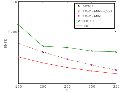
(b) RMSE vs. L with SNR=5dB
