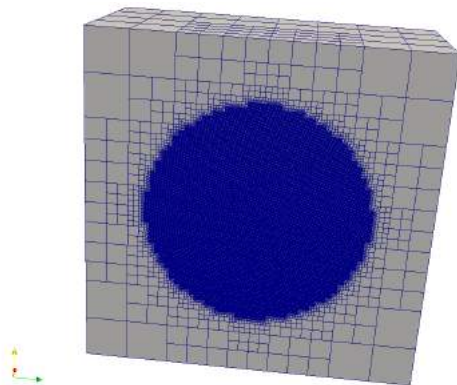
Figure 7: Spherical Refinement
