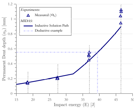
(a) Permanent indentation as function of energy
