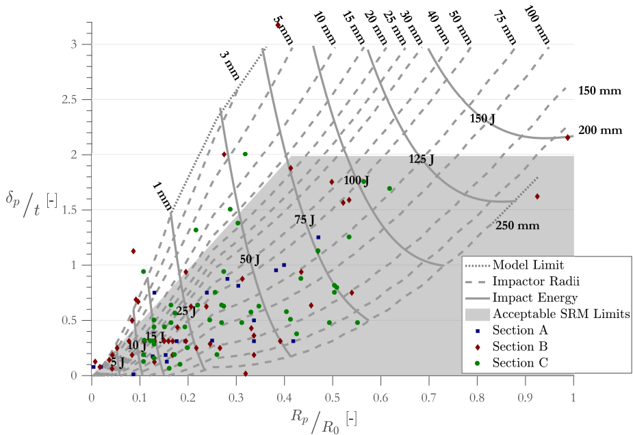
Figure 2.8: Reference damage data superimposed on impact threat map
