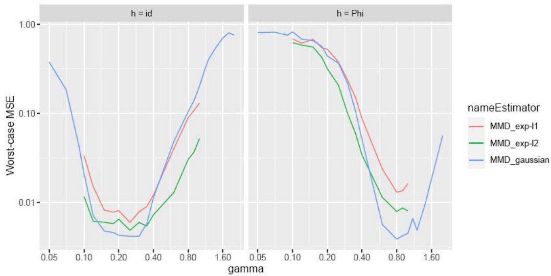
Figure 1. MSE of \hat{\theta}_n based on the Gaussian kernel k_U(U, V) = \exp(-\|h(U) - h(V)\|_2^2/\gamma^2) , the exp-L 2 kernel k_U(U, V) = \exp(-\|h(U) - h(V)\|_2/\gamma) and the exp-L 1 kernel k_U(U, V) = \exp(-\|h(U) - h(V)\|_1/\gamma) , as functions of \gamma .
