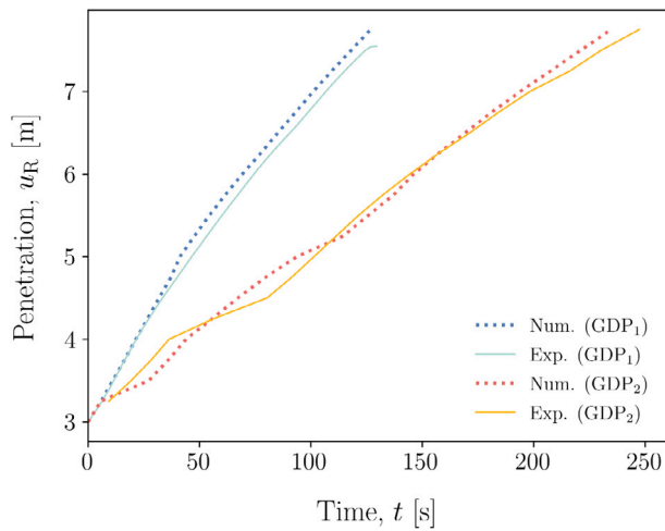
Fig. 8. Comparison of pile penetration ( u_R ) between numerical model predictions and experimental data for the piles GDP 1 and GDP 2 .
