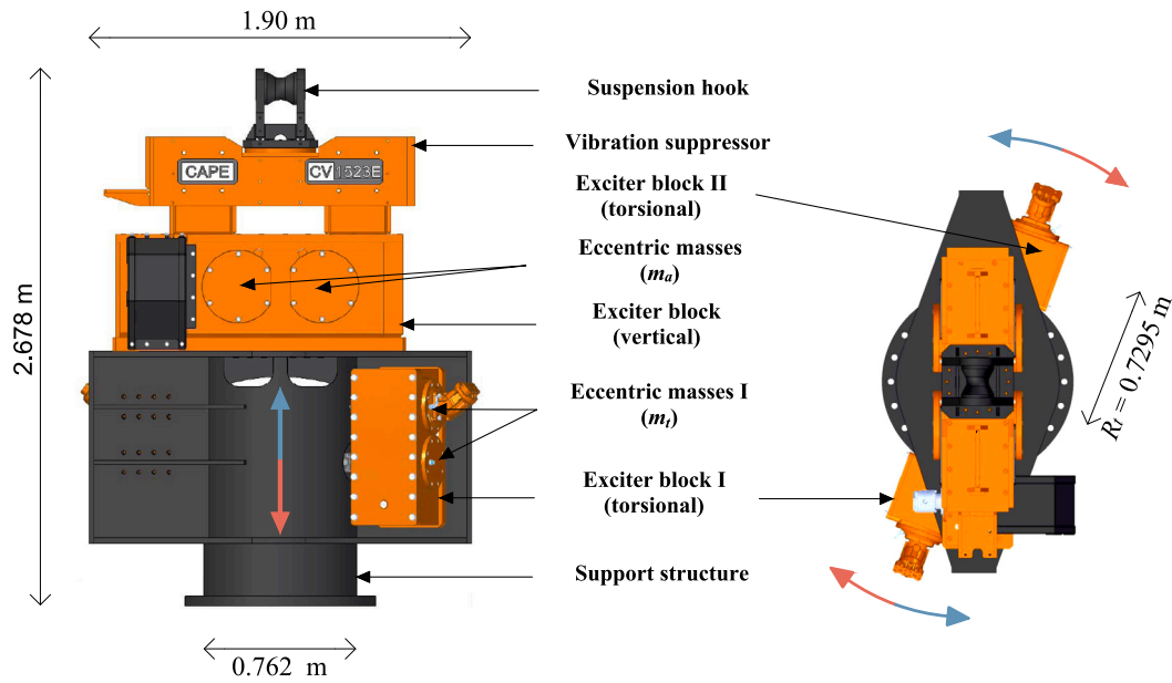
Fig. 2. Detailed design of the GDP shaker.
