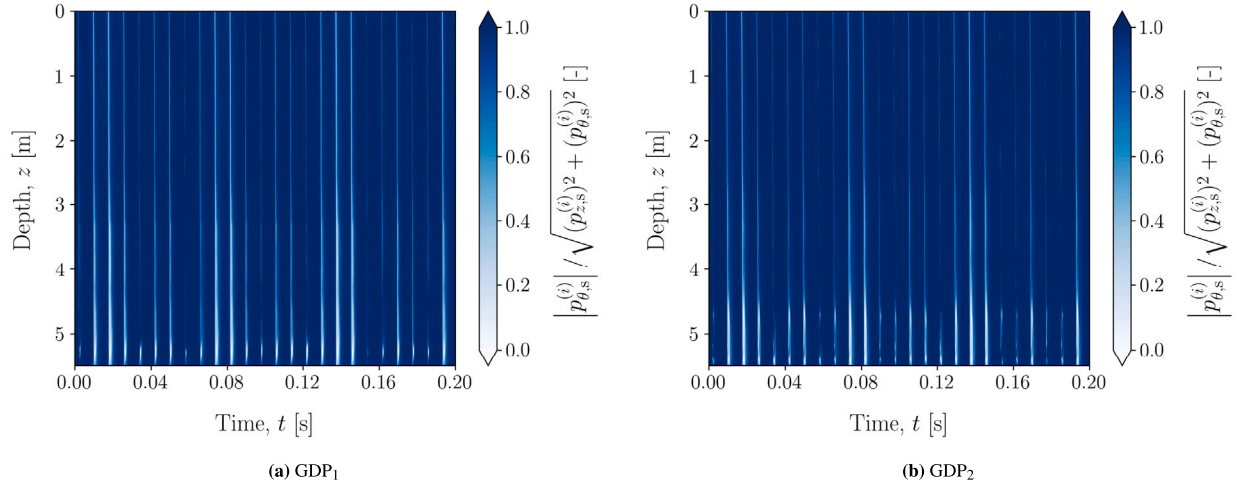
Fig. 12. Ratio of circumferential to total friction force \frac{|p_{\theta,s}^{(i)}|}{\sqrt{(p_{z,s}^{(i)})^2 + (p_{\theta,s}^{(i)})^2}} at u_R = 5.5 m.
