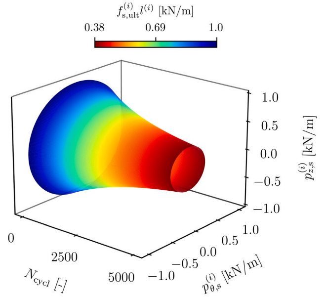
Fig. 6. History-dependent friction force at the i -th soil interface as a function of the number of loading cycles N_{cycl} , for f_{s,0}^{(i)} l^{(i)} = 1 kN/m, \beta_{\infty} = 0.2 , c_N = 0.0003 .
