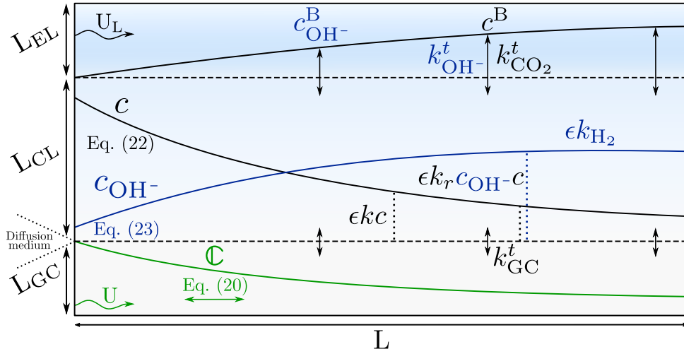
Fig. 5. Diagram of the numerical system (not to scale). Explicit variation in the flow-wise direction only occurs in the development of \bar{c} , through (20), and in the development of the boundary layer dependent mass transfer coefficients, k^t_{OH^-} and k^t_{CO_2} . The concentrations c and c_{OH^-} , governed by (22) and (23) respectively, depend on these parallel streams, as well as each other and \theta .
