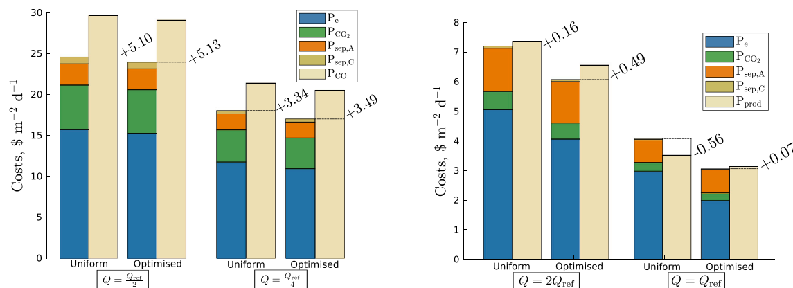
(a) Breakdown of the costs associated with electrolyser operation and value of produced CO for reduction on Ag in KOH for the systems in Fig. 6. The net profits are labeled above the dashed lines.
