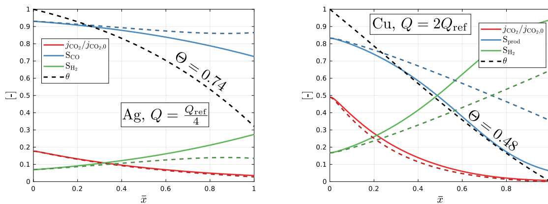
(a) Normalised partial CO 2 current densities and product and H 2 selectivities before and after optimisation for the case of reduction on Ag depicted in Fig. 6a
