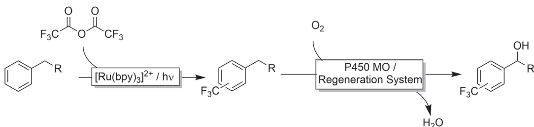
Scheme 9.14: Cascade of photocatalytic trifluoromethylation of arenes followed by P450 monooxygenase-catalyzed hydroxylation.
