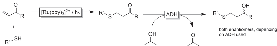
Scheme 9.13: Photoenzymatic cascade combining photoaccelerated thio-Michael addition and stereoselective, ADH-catalyzed ketoreduction.
