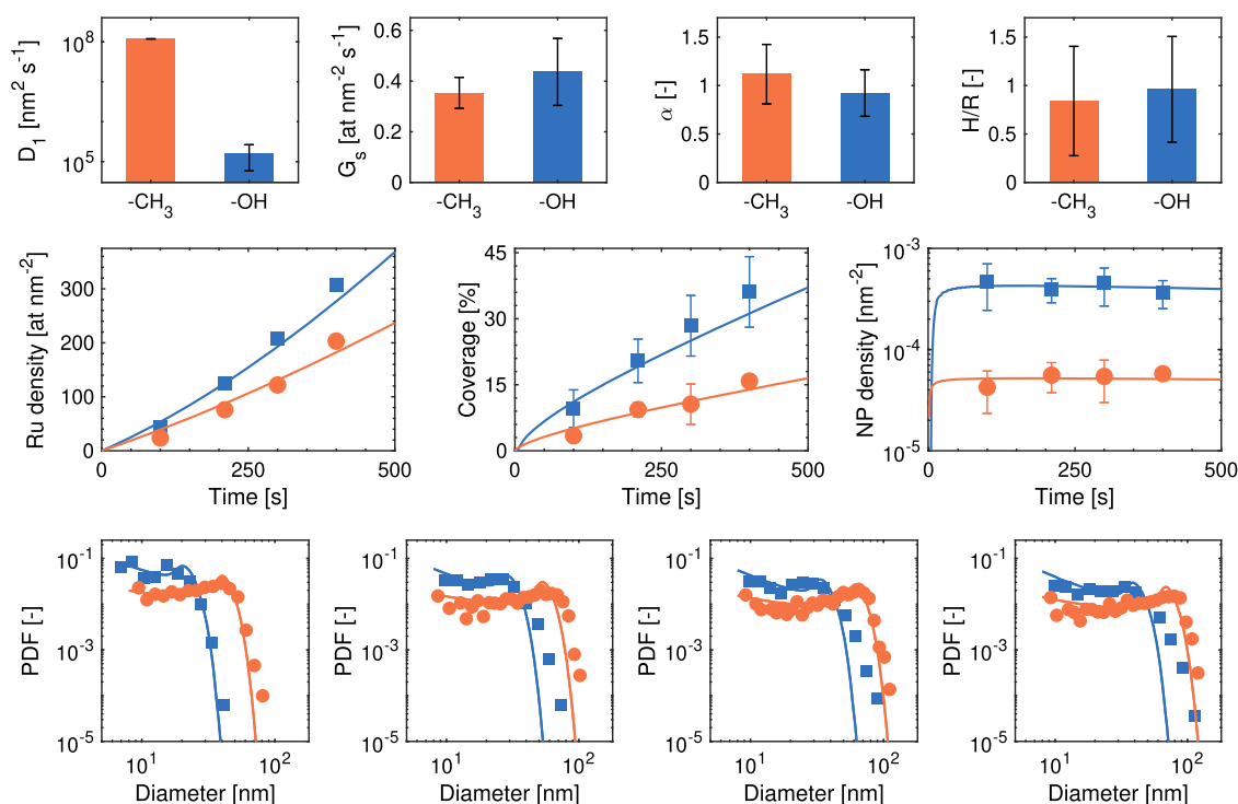
Figure 3. Comparison between simulation and experiments for Ru CVD at 250 °C on \text{--OH} -terminated (blue) and \text{--CH}_3 -terminated (red) \text{SiO}_2 . (a) Fitted parameters D_1 , \alpha , G_s , and H/R and their respective 95% confidence intervals for the two surface terminations. (b) Ru areal density as measured by RBS. (c) Areal coverage. (d) Nanoparticle density. (e) Size distribution of the nanoparticles expressed in terms of the probability density function (PDF) at different times: 100, 210, 300, and 400 s, from left to right. Lines and symbols indicate simulated and experimental data, respectively. Size distributions, coverages, and number densities are obtained by SEM. The simulated observables are rescaled to account for the fact that nanoparticles smaller than a certain threshold ( \sim 5 nm) could not be imaged or counted.
