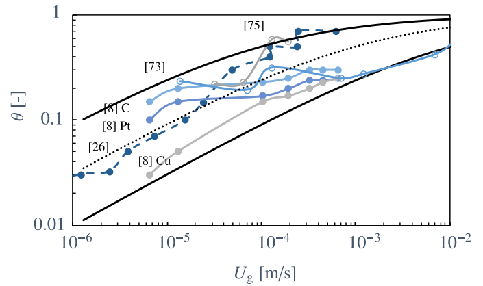
Fig. 7. The surface coverage \theta of hydrogen bubbles in \text{H}_2\text{SO}_4 (solid circles) on vertical electrodes (solid lines) and horizontal electrodes (dashed lines). The open circles indicate alkaline electrolytes NaOH and KOH. The black lines indicate Eq. (10) with r = 0.5 and j_c = 10^{-4} (top solid line), 10^{-3} (middle, dotted) and 10^{-2} \text{A/m}^2 (bottom, solid), respectively. The top and line of Ref. [8] used a carbon electrode and platinum electrode, respectively and would fit better with a still lower power r \approx 0.15 and r = 0.2 , respectively [73].
