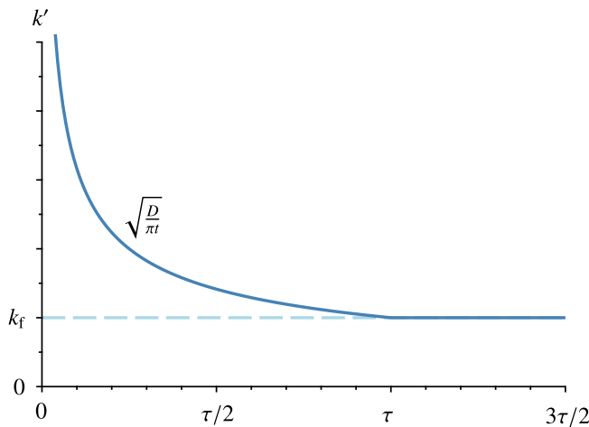
Fig. 6. The local mass transfer coefficient k' as a function of time after the departure of a bubble, modelled using the one-dimensional diffusion equation analytical solution. After a time \tau this equals the background flow mass transfer coefficient k_f , which is then assumed to take over.
