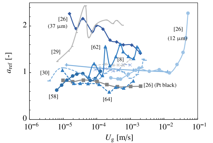
Fig. 3. For hydrogen bubbles in sulphuric acid ( \text{H}_2\text{SO}_4 ) the parameter a_{\text{ref}} , defined by Eq. (3), does not depend on gas flux U_g = j \eta_m'/2F for most of the data obtained from the literature. Solid and dashed lines concern experiments with horizontal and vertical electrodes, respectively. The line colour and marker type only differ to be able to distinguish the different sources better. For Ref. [57] the grain size of the sanding paper used for treating the platinum electrodes is indicated.
