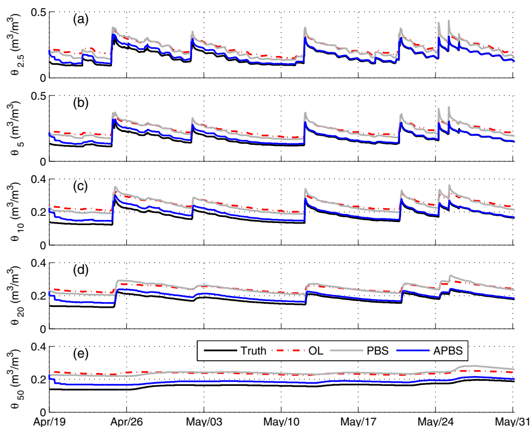
Figure 5. Comparison of the soil moisture estimated using PBS and APBS at 5 depths.
