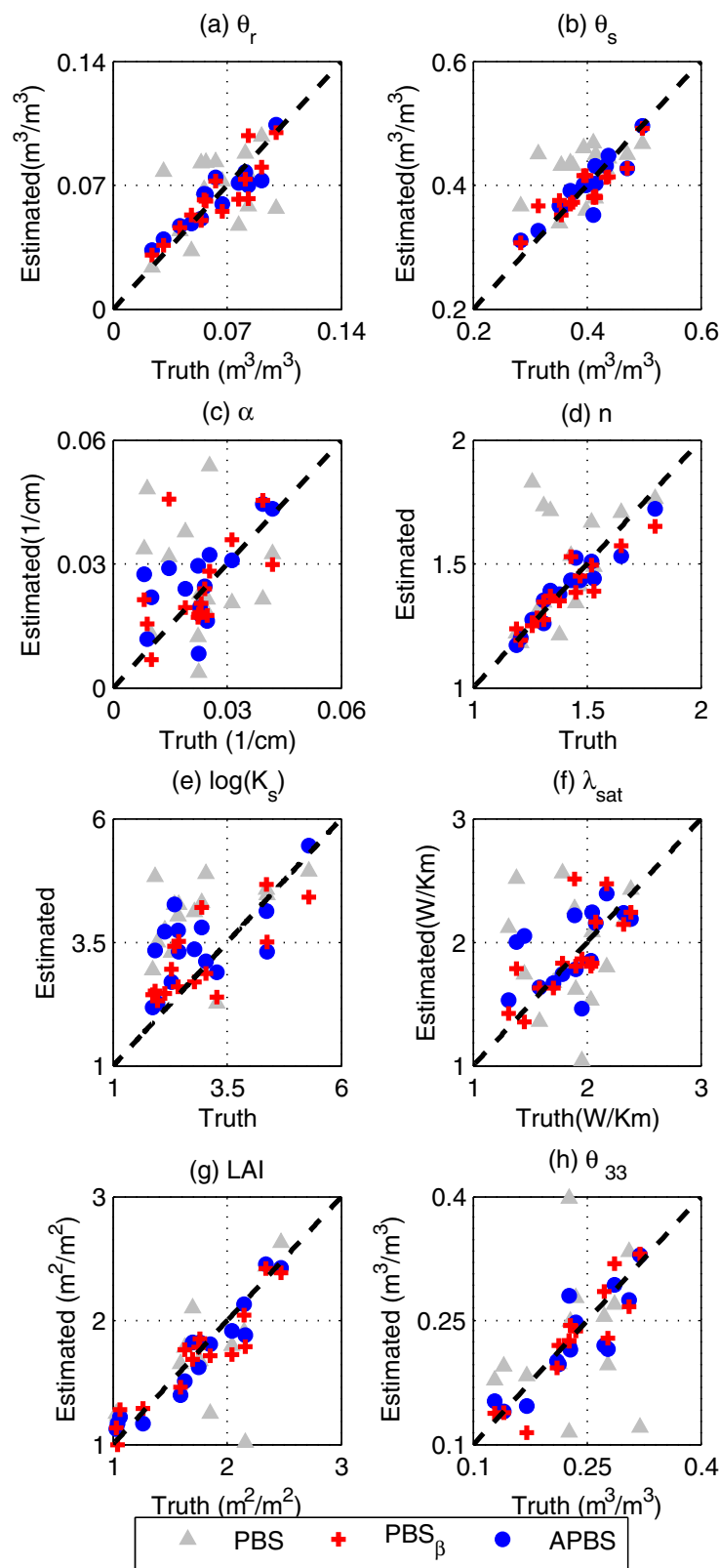
Figure 7. (a–g) Comparison of the true and the estimated model parameters and (h) the \theta_{33} calculated using the estimated soil hydraulic properties.
