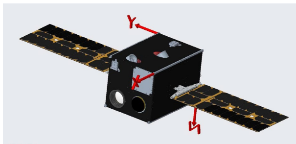
Fig. 4. Rendering of the LUMIO spacecraft configuration at the end of the Phase A study.
