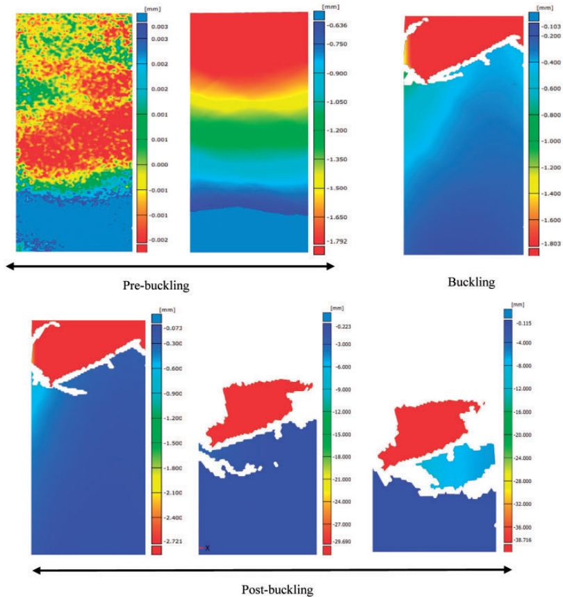
Figure 7. In-plane displacements contours of DIC method.
