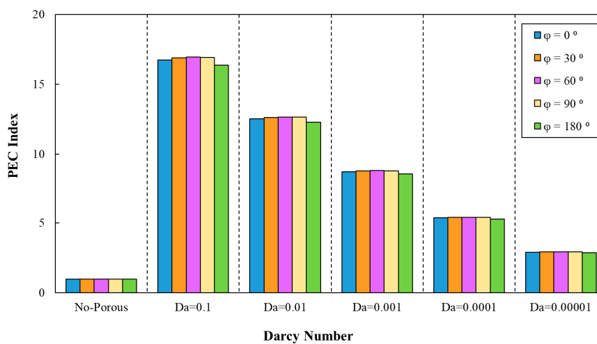
Figure 18. The variation of PEC index against different Darcy numbers for various phase shifts, ( a = 0.5 mm, \lambda = 10 mm).
