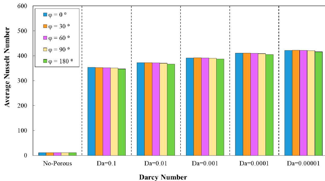
Figure 8. Comparison of average Nusselt number for diverse Darcy numbers with various phase shifts and wavelength of ( a = 0.5 mm, \lambda = 10 mm).
