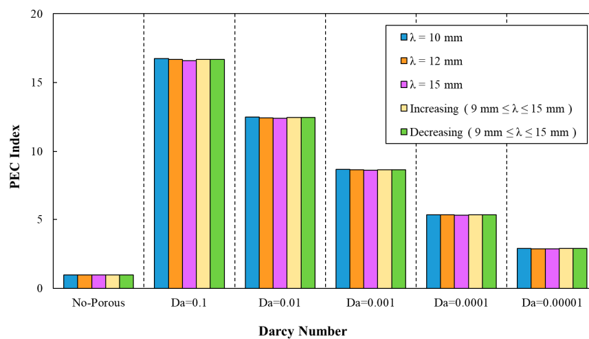
Figure 16. The variation of PEC index against different Darcy numbers for various wavelengths, ( a = 0.5 mm, \varphi = 0^\circ ).
