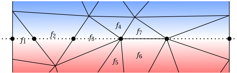
Figure 3.23: Possible situations of triangles intersecting an isocurve (the dashed line). Among three vertices of a triangle, there may be zero ( f_{1,2} ), one ( f_{3,4,5} ), or two ( f_{6,7} ) vertices located on the isocurve.
