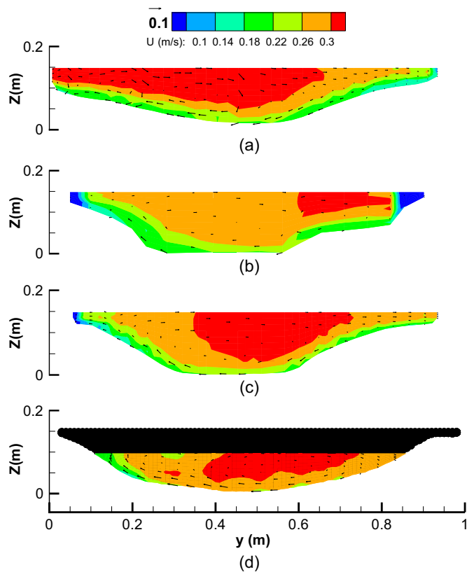
Fig. 6. Cross-stream velocity vectors overlaid on streamwise velocity (contour form) at 90° cross section obtained from (a) angle of repose; (b) standard Delft3D; (c) developed bank erosion models; and (d) experimental observations. Black zone shows unmeasured area during ADV measurements.
