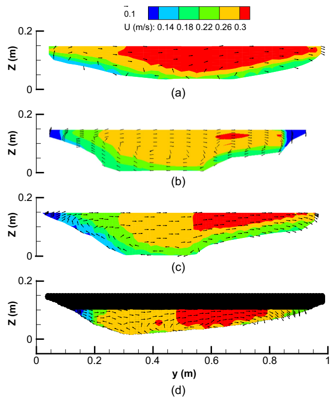
Fig. 7. Cross-stream velocity vectors overlaid on streamwise velocity (contour form) at 135° cross section obtained from (a) angle of repose; (b) standard Delft3D; (c) developed bank erosion models; and (d) experimental observations. Black zone shows unmeasured area during the ADV measurements.
