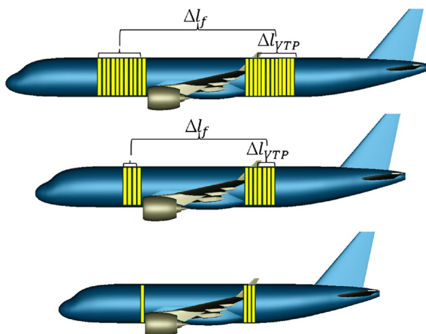
Fig. 4 Example of the change in fuselage length and wing position for an aircraft family
