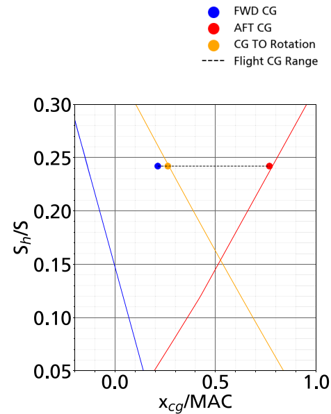
Fig. 17 Scissors plot for the D250-LH2 concept (Point design)
