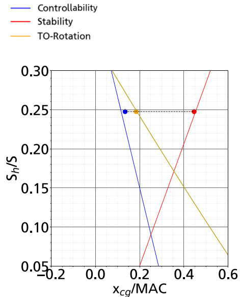
Fig. 7 D239-S (Point design) scissors
