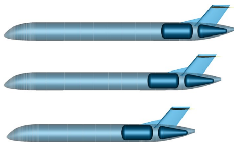
Fig. 15 D250-LH2 family concept with constant fuel capacity and varying payload
