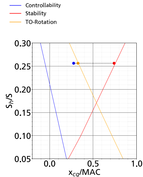
Fig. 18 Scissors plot for the D250-LH2-short (Point design)
