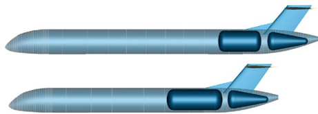
Fig. 23 LH2 family concept with varying fuel capacity and payload. D250-LH2 (top) and D250-LH2-ER-short (bottom)
