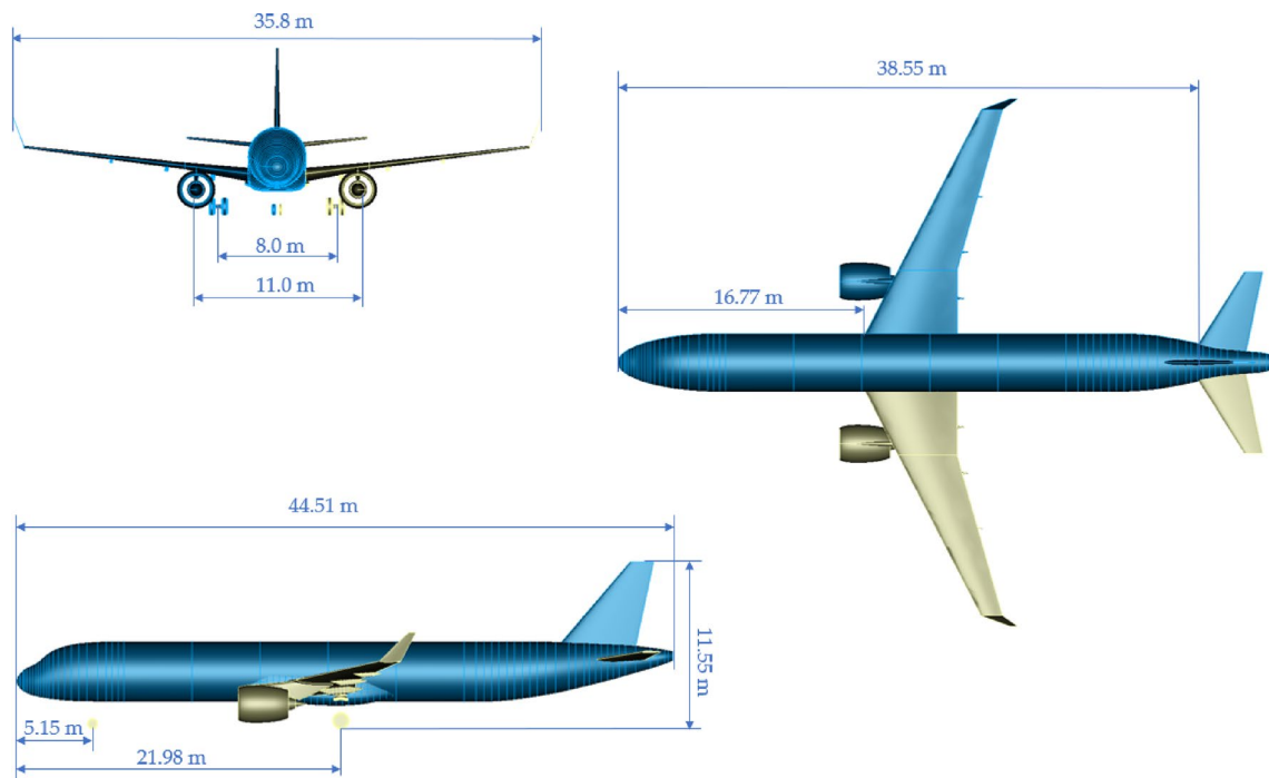
Fig. 25 Three standard views for the D239 final concept
