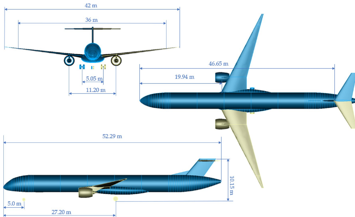
Fig. 28 Three standard views for the D250-LH2 final concept
