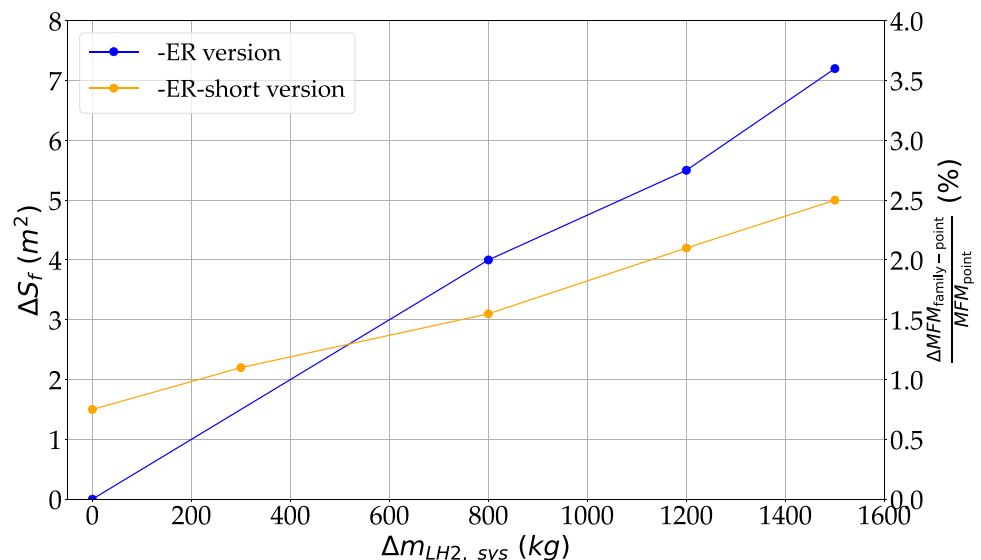
Fig. 24 Effect of tank mass increase on HTP area and empennage commonality block fuel penalty for D250-LH2-ER and ER-short variants
