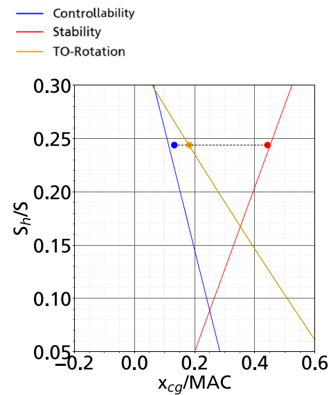
Fig. 3 Example of minimum HTP area for stability and TO rotation
