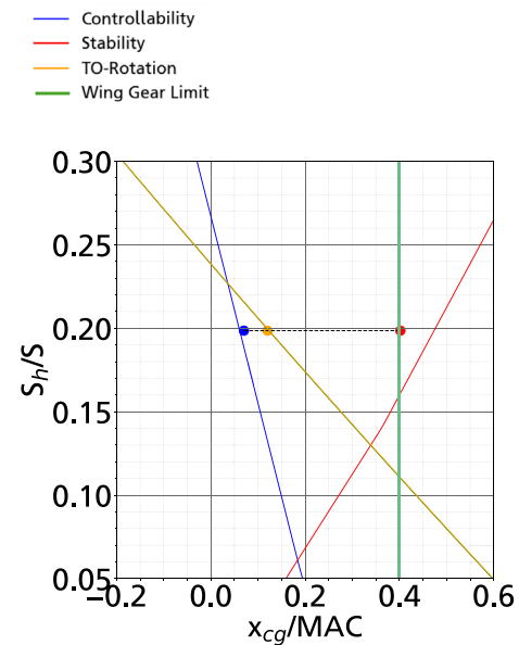
Fig. 14 Scissors plot for the D250 with wing integrated landing gear (Point design)
