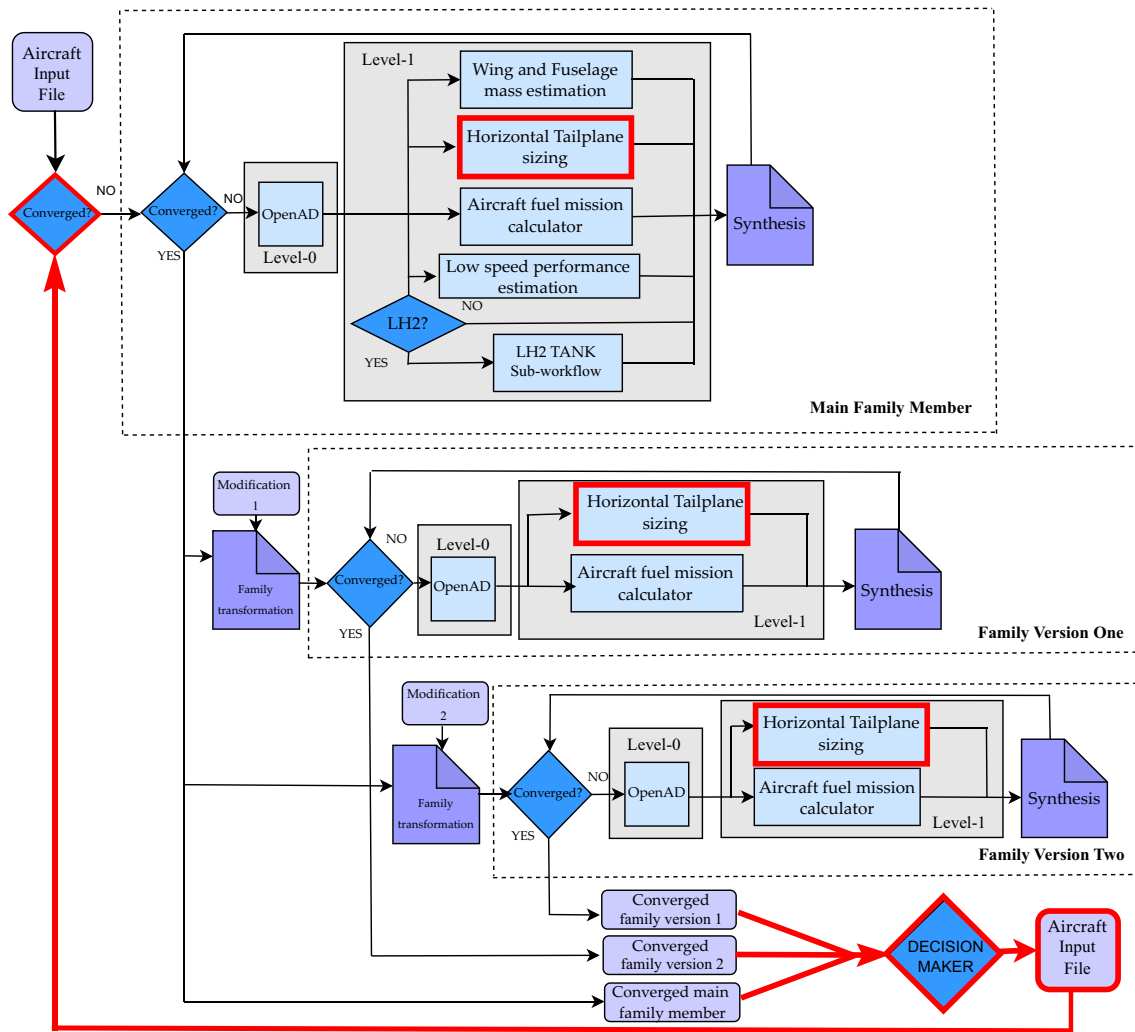
Fig. 1 Modified EXACT workflow schematic
