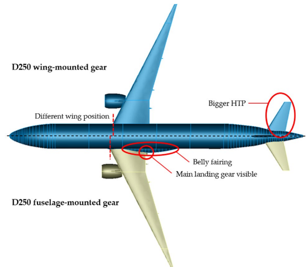
Fig. 12 Plan view of the D250 concept (point design) with fuselage-mounted (bottom) and wing-mounted landing gear (top)
