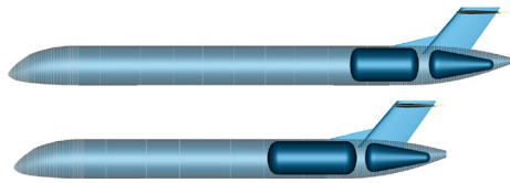
Fig. 22 LH2 family concept with constant payload and varying fuel capacity. D250-LH2 (top) and D250-LH2-ER (bottom)
