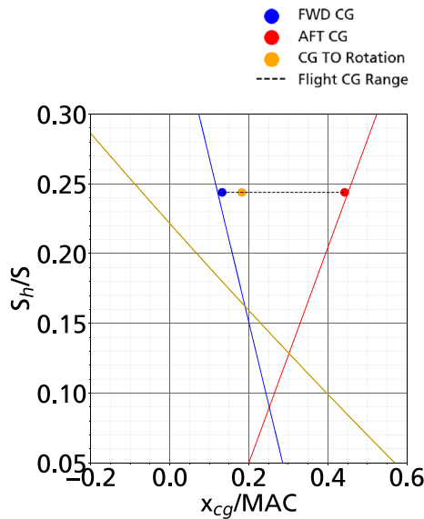
Fig. 2 Example of minimum HTP area for trim and stability
