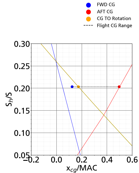
Fig. 13 Scissors plot for the D250 with fuselage integrated landing gear (Point design)
