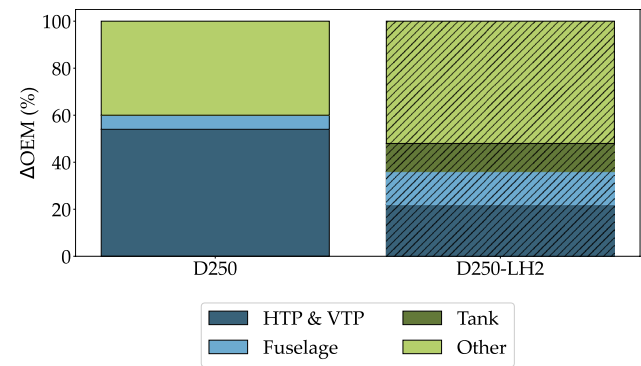
Fig. 19 OEM-breakdown by component increment due to tailplane commonality for the D250 and D250-LH2
