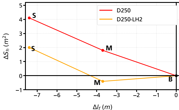
Fig. 16 Point design results for the required HTP area as a function of the change in fuselage length for both D250 and D250-LH2 family concepts. Results are shown for all base (or long) (B) mid (M) and short (S) family variants
