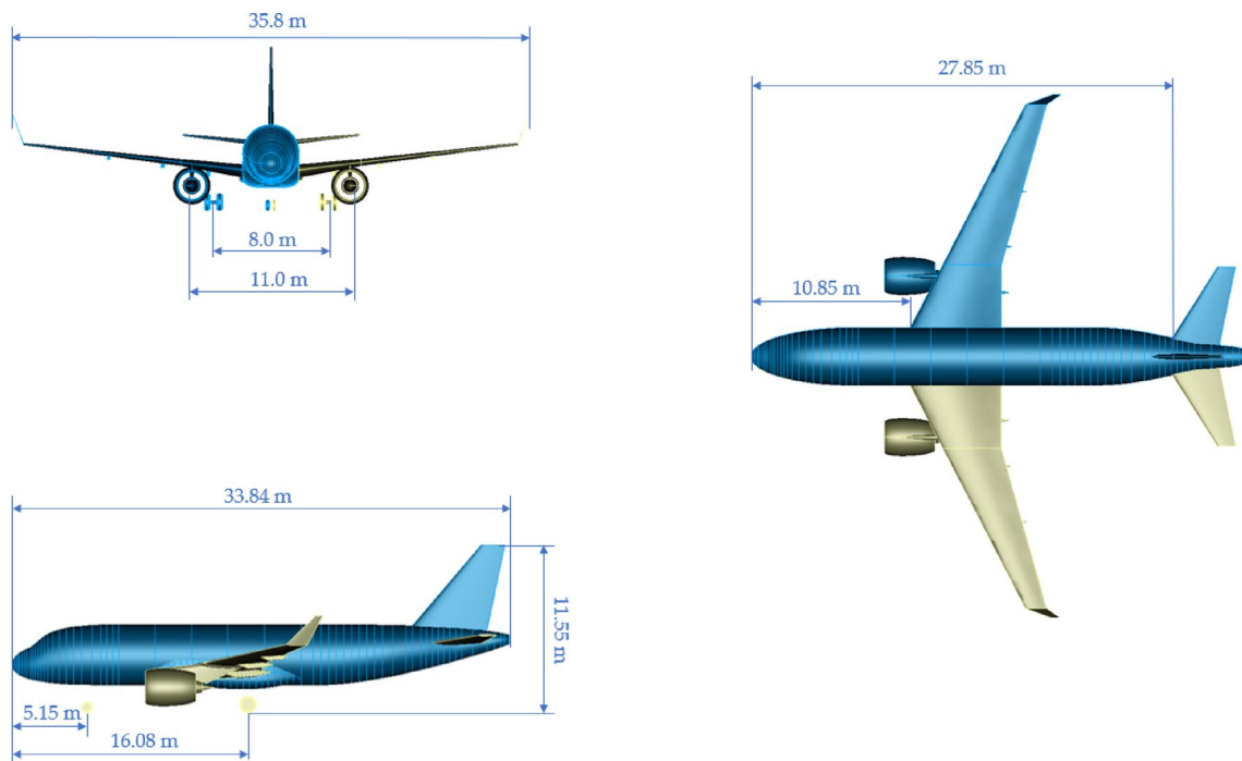
Fig. 26 Three standard views for the D239-short final concept
