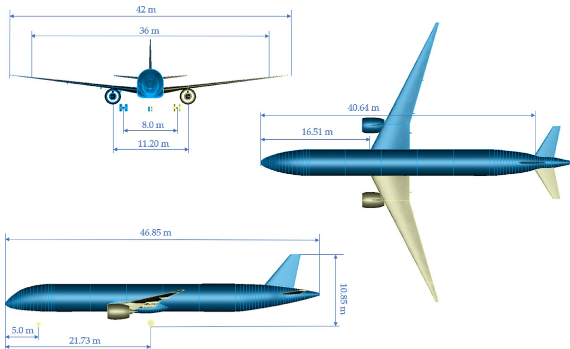
Fig. 27 Three standard views for the D250 final concept
