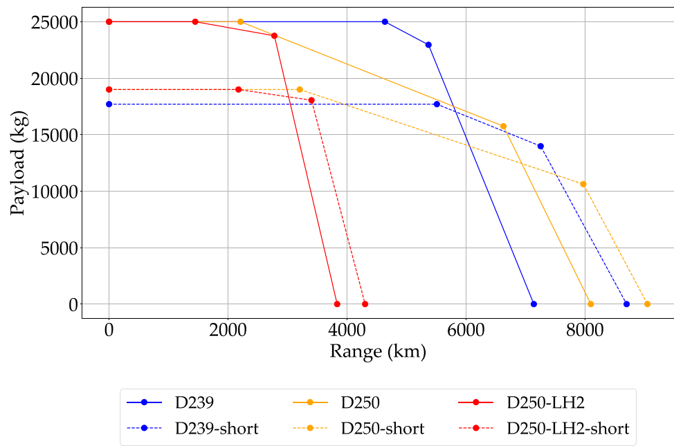
Fig. 21 Payload-range diagram comparison for the -long and -short members from the D239, D250, and D250-LH2 families
