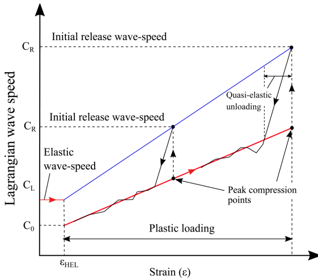
FIG. 20. Schematic Lagrangian wave speed vs strain diagram for a typical ductile material subject to shock compression and release. The uniaxial strain is computed as \left(1 - \frac{\rho_0}{\rho}\right) . The red line shows the evolution of the Lagrangian wave speed as the material undergoes compression (loading). For strains lower than the elastic limit ( \epsilon_{HEL} ), the wave speed corresponds to the longitudinal elastic wave speed ( C_L ). For strains higher than \epsilon_{HEL} , the plastic loading wave speeds evolves as shown in the figure, with C_0 obtained from the material's linear U_S - u_p relation: U_S = C_0 + Su_p . After reaching peak compression, at initial release (unloading), the material wave speed abruptly increases to a point on the "initial release velocity" line (shown in blue). With further release, the material wave speed proceeds along the quasi-elastic path (shown in black) and eventually merges with the plastic loading path. For SLG, it is observed that the release wave speeds always remain significantly higher than the loading wave speeds and never merges with the plastic loading path (see Figs. 12 and 19).
