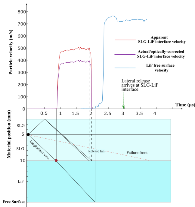
FIG. 7. Velocimetry data from experiment No. SSL-3 for the SLG–LiF interface and the LiF-free surface. A failure wave velocity of 1.3 km/s was assumed in the material position–time ( X – t ) diagram. Impact velocity is 879.6 m/s.
