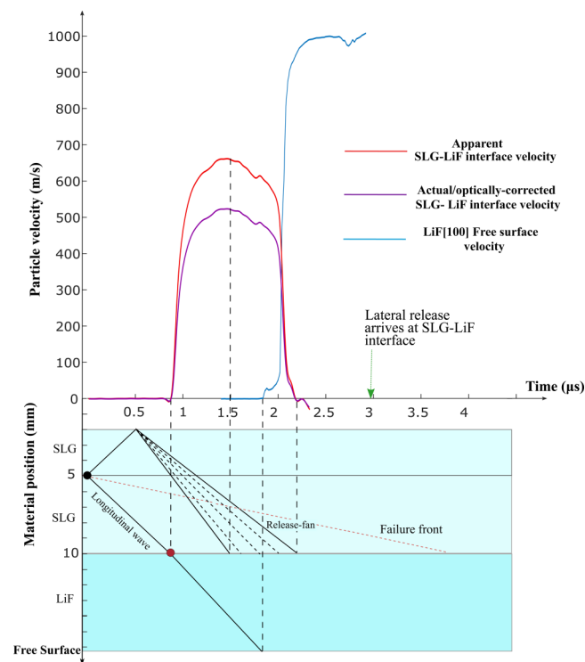
FIG. 5. Velocimetry data of experiment No. SSL-2 for SLG–LiF interface and LiF-free surface. A failure wave velocity of 1.3 km/s was assumed in the material position–time ( X-t ) diagram.
