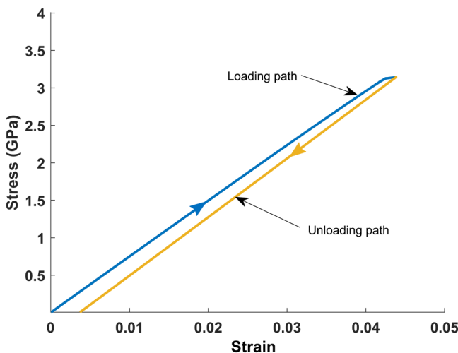
FIG. 10. Stress-strain plot for experiment No. SSL-4. The uniaxial strain is also identical to the volumetric strain \left(1 - \frac{\rho_0}{\rho}\right) .
