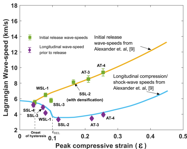
FIG. 12. Plot of Lagrangian wave speeds of compression and release waves in SLG. The data for experiments AT-3 and AT-4 are taken from Alexander et al. 28 The compression (blue line) and release (yellow line) wave speeds for SLG provided as a function of peak particle velocity in Alexander et al. 11 are plotted here as functions of strains (refer to the Appendix in Joshi et al. 17 for the procedure). The onset of hysteresis is the strain (0.04) at which the release and compression wave speeds start to differ significantly. The strain ( \epsilon ) is computed as (1 - \frac{\rho_0}{\rho}) .
