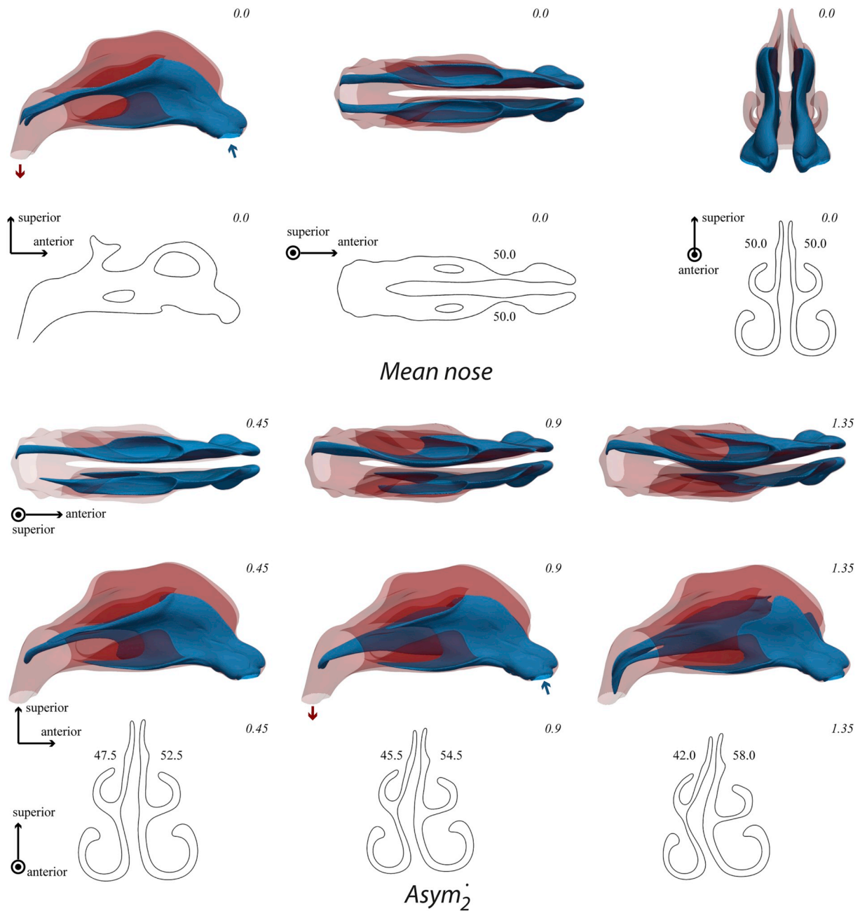
Fig. 6. Qualitative volumetric temperature-threshold maps for the mean nose (top) and the second asymmetrical PC (bottom). Cold air (5 °C) is inhaled. Inhaled air with a temperature above 27 °C is rendered completely transparent. Air with a temperature below 27 °C is shown in blue and opaque. The nasal wall, with its constant temperature of 32.6 °C, is depicted with a lower opacity in red. The numbers in the right top corners for each map provide the scaling factors of the standard deviations. The numbers located at the different coronal, sagittal and transversal slices represent the percentages of the total flow rates passing through the nose. For example, for the mean nose, the 50.0 at both channels indicates that exactly half of the overall flow rate passes through each of both channels, as expected. A coronal slice, located at the plane in which the inferior meatus reaches its maximum height, is shown to clarify the effect of each specific PC.
