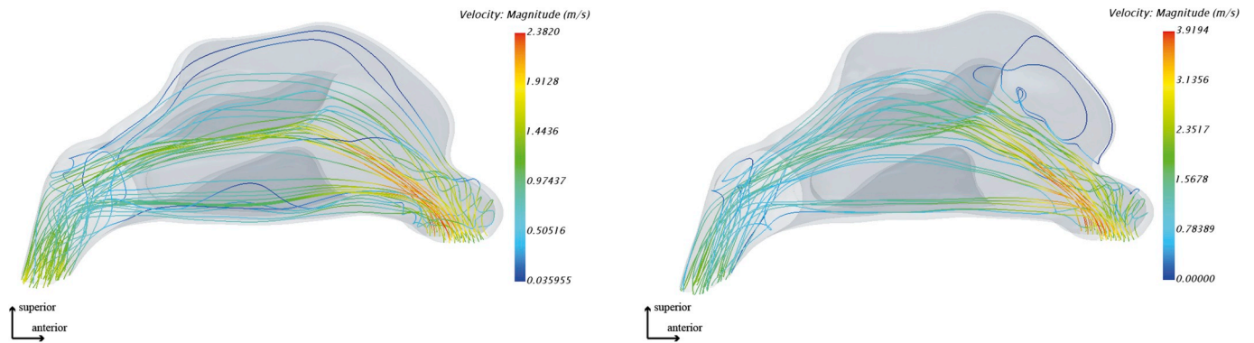
Fig. 5. Two examples of a converged result: (left) for the mean nasal geometry and (right) for the first symmetrical mode. The streamlines, representing the path that massless particles will follow are color-coded with the velocity magnitude. These results will be further discussed in Section 4.
