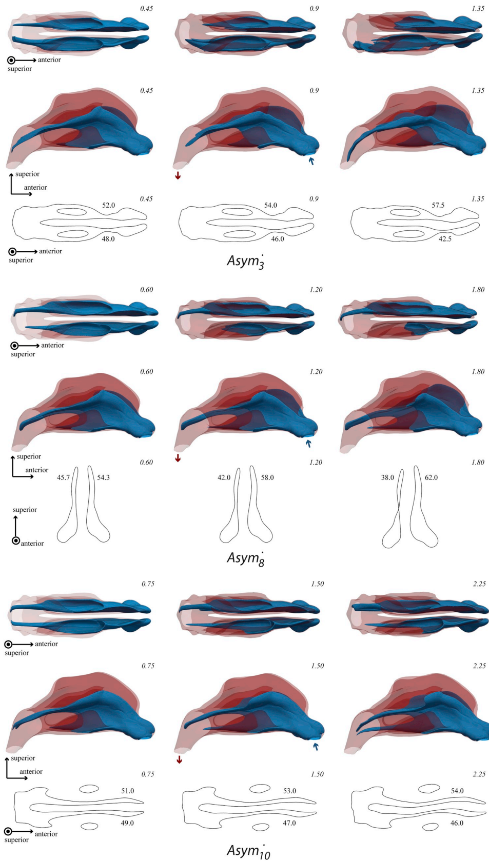
Fig. 7. Qualitative volumetric temperature-threshold maps for asymmetrical PC 3 (top), PC 8 (middle), and PC 10 (bottom). The reader is referred to Fig. 6 for detailed information on the maps.
