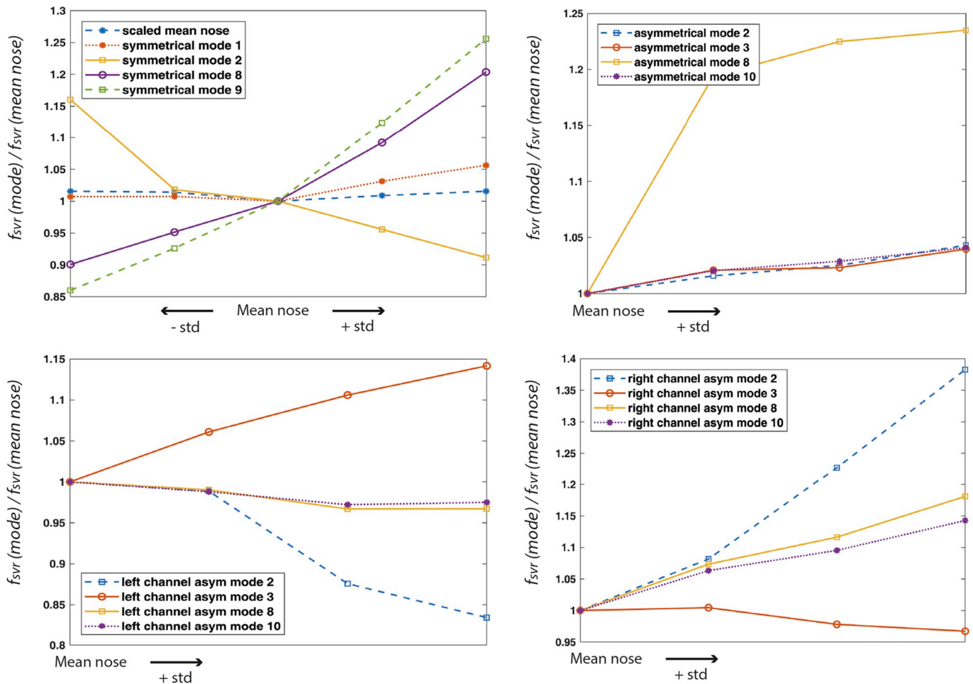
Fig. 10. Normalized unitless surface-to-volume ratio (SVR) on the vertical axis, defined as the square root of S^3 and divided by the volume times the unitless SVR of the mean nose. Moving along the horizontal axis changes the scaling factor of the shape modes. (Top left) SVR for the symmetrical modes. Each line in a graph corresponds with a shape mode, and each data point with one of the shape instances presented in the previous results. Starting from the center (mean nose), the scale factor of the standard deviation (std) decreases or increases respectively. (Top right) SVR for the asymmetrical modes. Only one side on the horizontal axis is shown because of the symmetry for positive and negative std. (Bottom left) SVR for the left nasal channel of the asymmetrical modes. (Bottom right) SVR for the right nasal channel of the asymmetrical modes.
