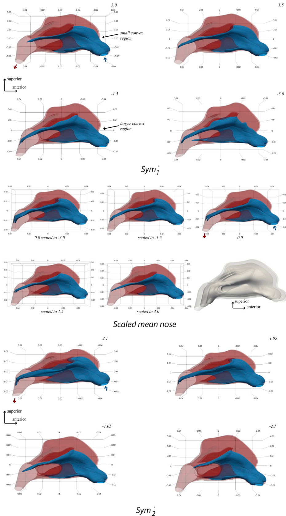
Fig. 8. Qualitative volumetric temperature-threshold maps for symmetrical PC 1 (top), PC 2 (bottom), and the scaled mean nose (middle). See Fig. 6 for detailed information on the maps. Nasal channel flow fraction percentages are no longer shown here because we are dealing with symmetrical shapes. On the right of Fig. 8 (middle), the difference in size for the scaling of the average nose is shown by overlaying the shapes.
