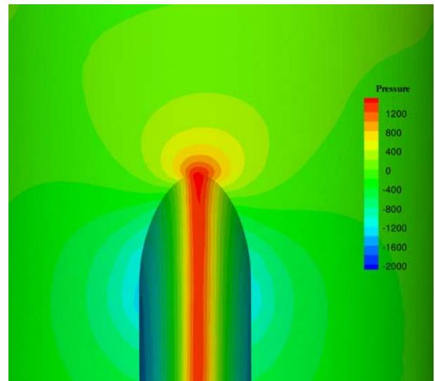
Fig. 7. Effect of the propeller slipstream on the local pressure distribution at the model sting and fuselage. The viewpoint is from upstream looking downstream at the leading edge of the sting at the bottom of the aircraft fuselage. Contours of relative pressure level ([Pa]) are plotted. The pressure is taken relative to a free-stream reference of 0 [Pa]
