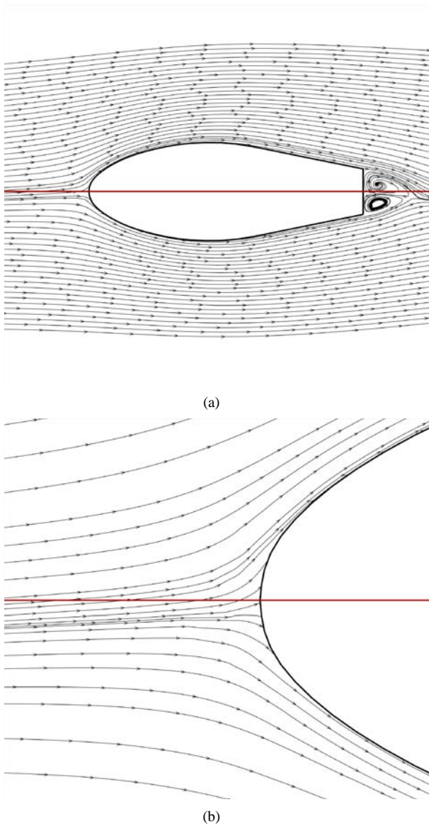
Fig. 6. Effect of the propeller slipstream on the local angle of sideslip at the model sting (a) A top view of a cross sectional plane of the model sting very close to the fuselage showing the local streamlines. As a reference the symmetry line of the sting is shown (b) The same as (a) but focused near the nose of the model sting
