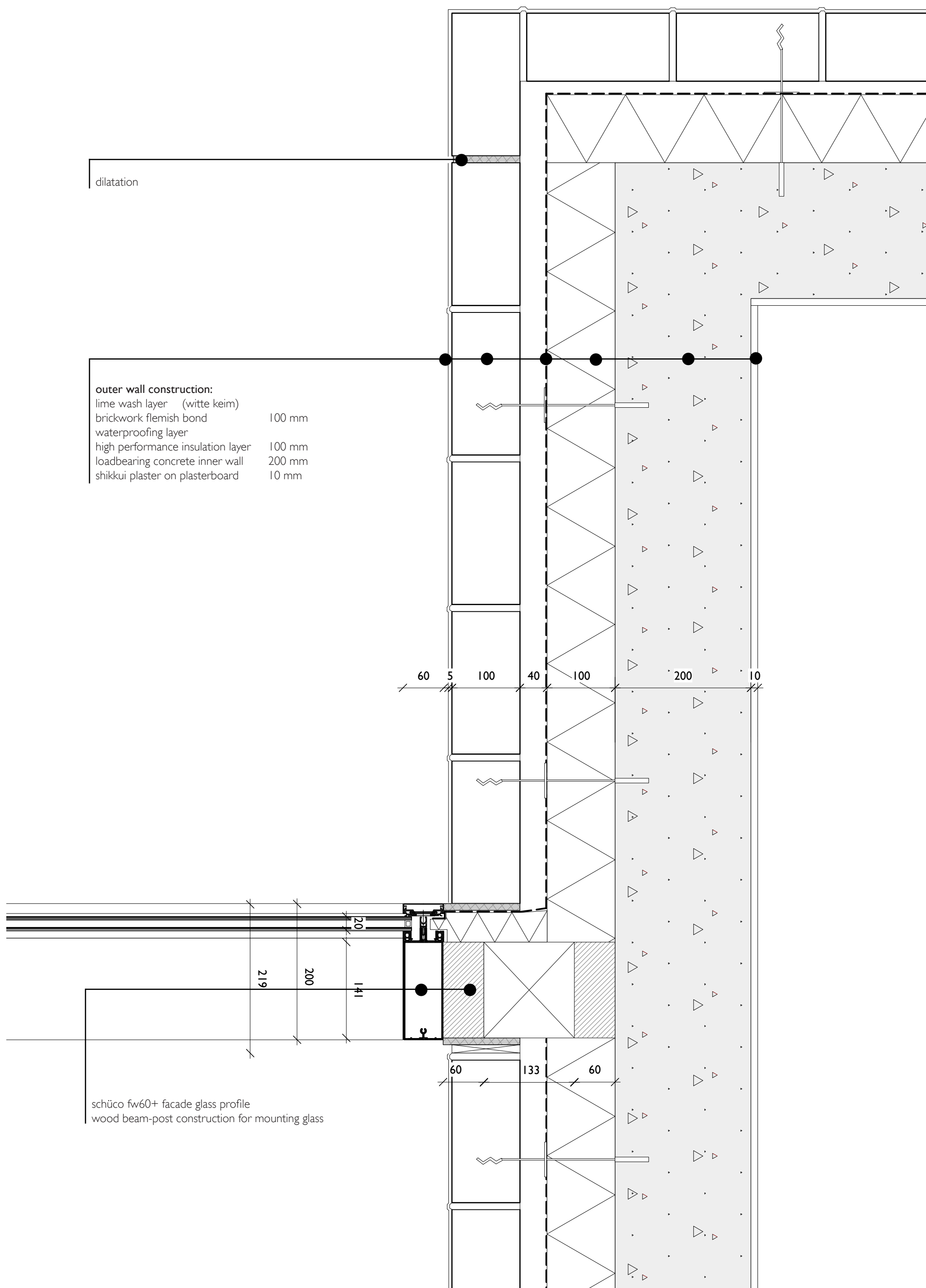
H02 - Horizontal detail brick facade with connection with intermediate facade
