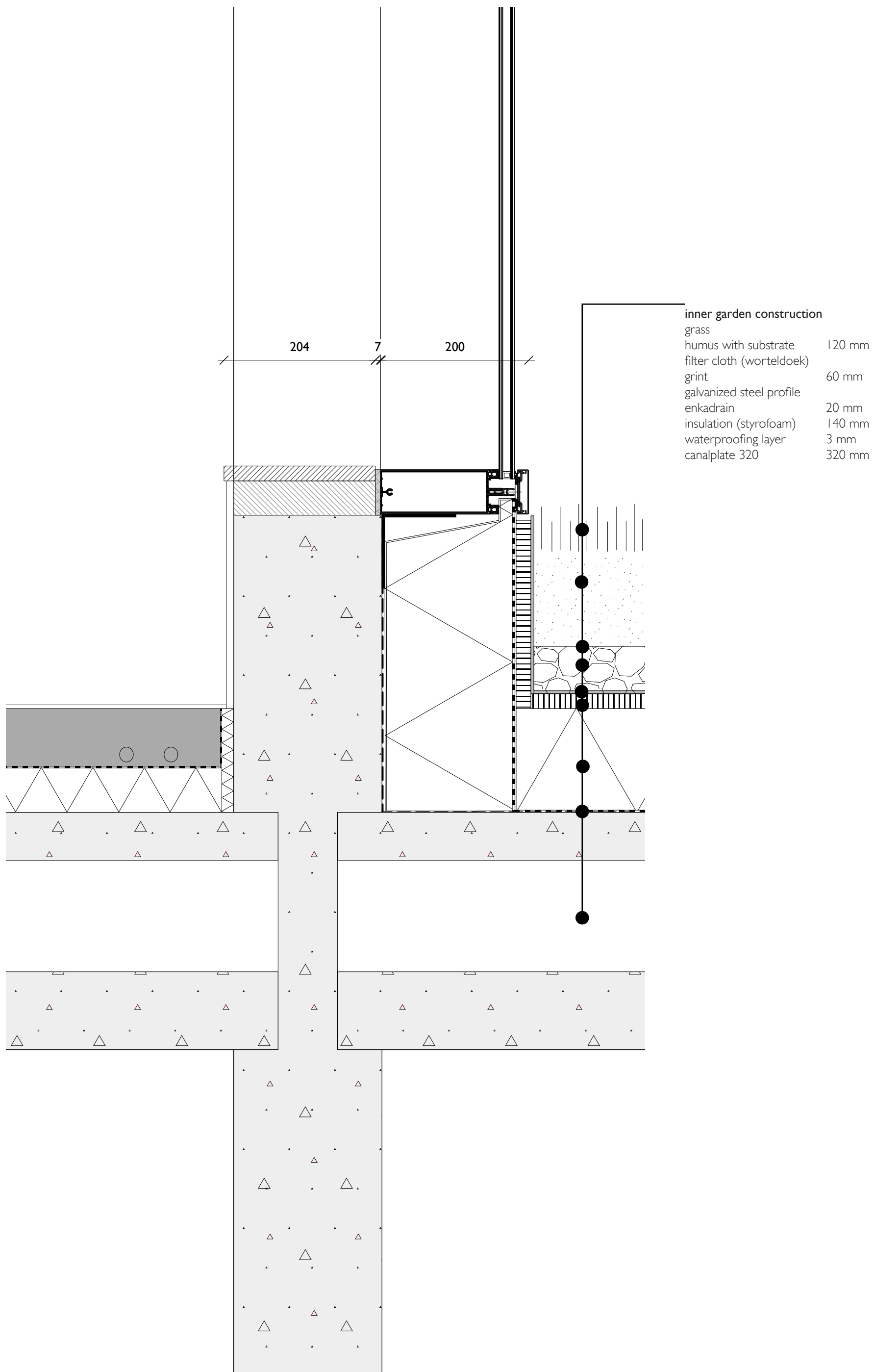
V07 - ICU inner patio with bottom connection detail
