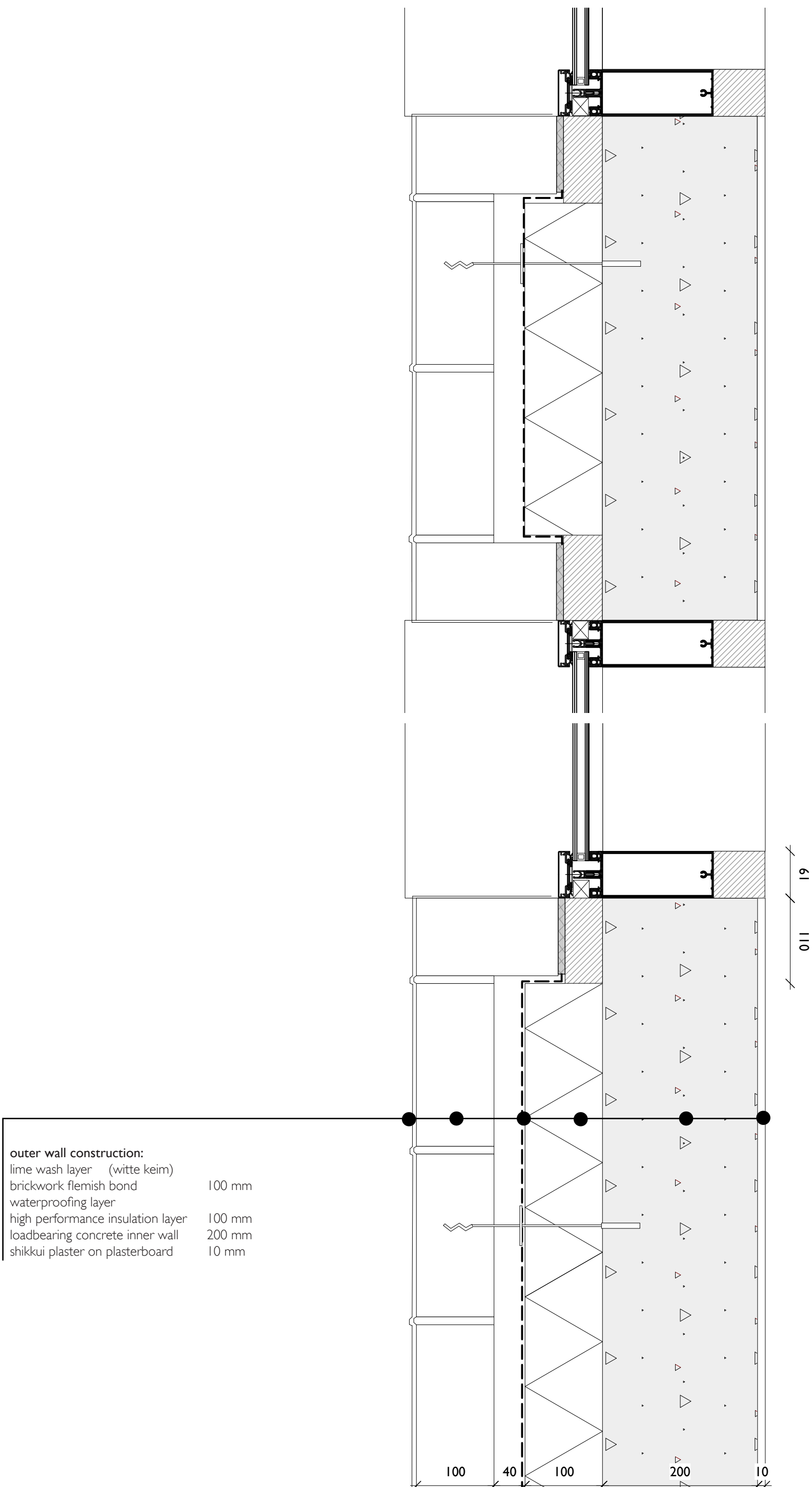
H01 - Horizontal detail brick facade
