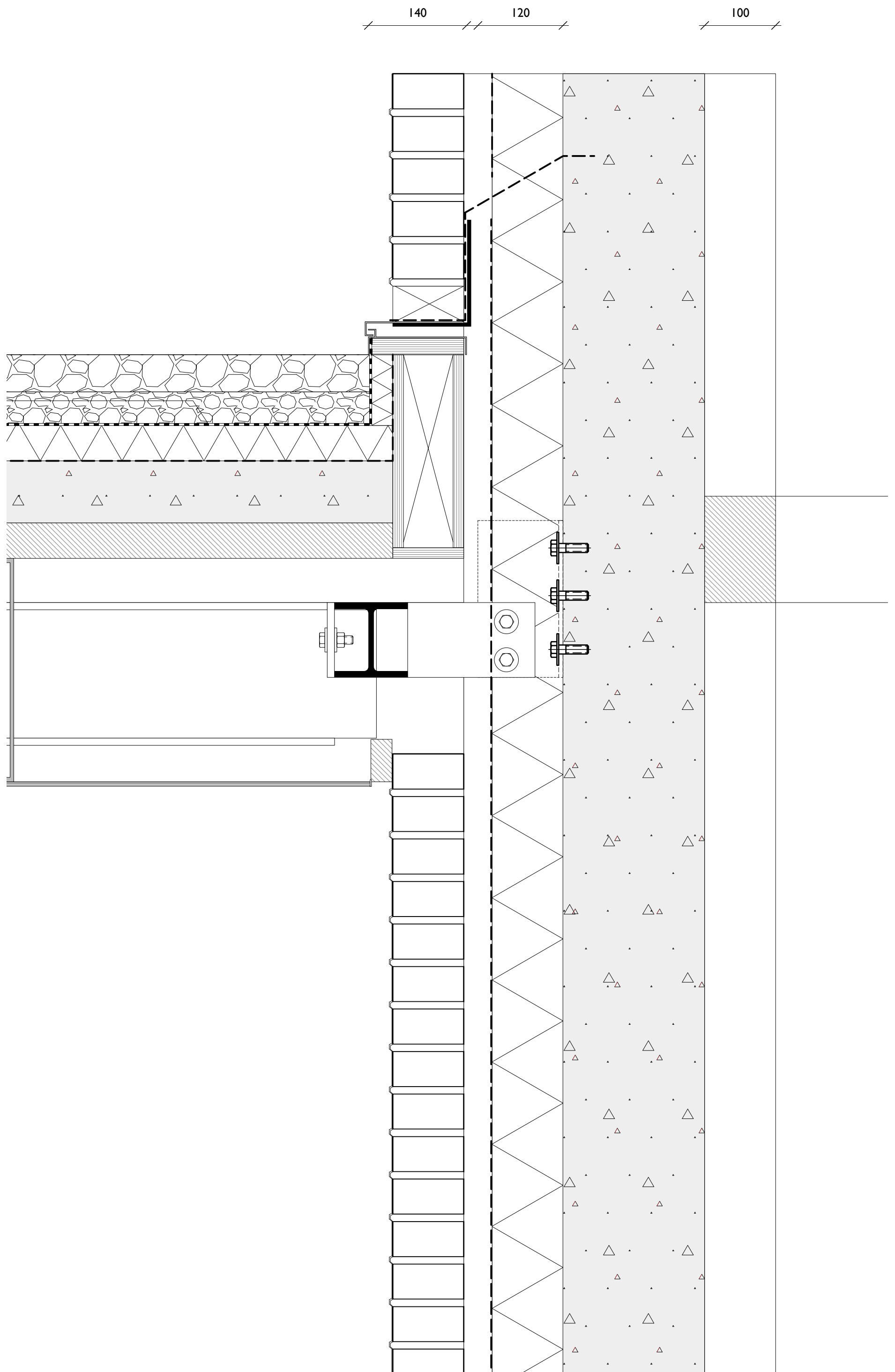
V09 - Stability connection between roof of Intermediate with brick facade
