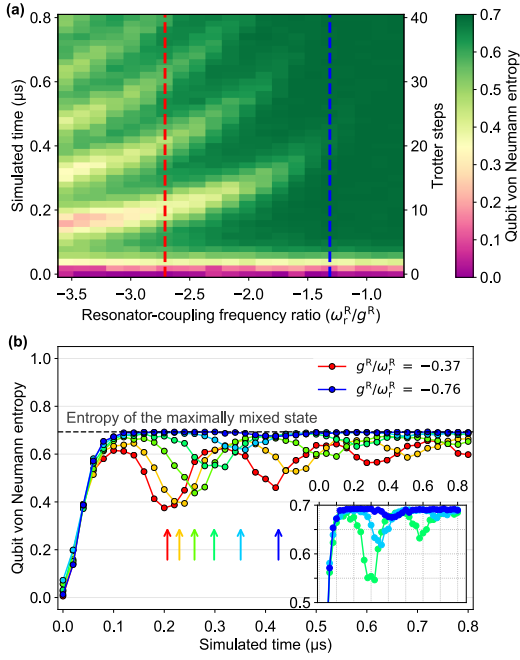
Figure 3.17: Tomography of the reduced state of qubit Q_R as a function of simulation time and relative resonator-coupling frequency. (a) Image plot showing the dynamics of qubit quantum von Neumann entropy over different ultrastrong-coupling regimes. (b) Line slices are plotted at evenly spaced frequencies between the blue and red dashed lines. Inset: Zoom showing revivals.
