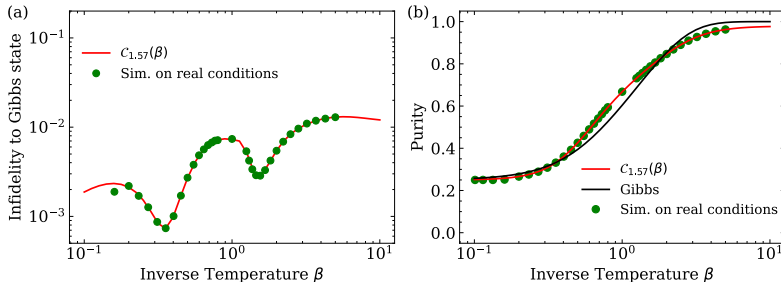
Figure 5.17: Test of the classical optimizer. By feeding simulated readout data for an ideal processor (instead of actual measurements) into the software stack used to control our experiment [153], we verify the limitations of the optimizer under the exact configuration and conditions used in the experiment. Both figures include the curves from Fig. S3 (red) as reference. (a) Simulated infidelity (green) of the reduced state of system A to the Gibbs state after optimization. (b) Corresponding purity of the reduced state (green). The purity of the Gibbs state is also shown for comparison (black).
