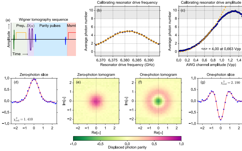
Figure 3.12: Calibration of Wigner tomography. (a) Pulse sequence used to make the displaced photon parity measurement which provides a direct measurement of the Wigner function at a particular position in phase space. (b) This plot shows the response of R_R to the drive pulse as a function of drive frequency, as recorded by the Q_W photon meter, centred at 6.3814 GHz, with a FWHM of \sim 21 MHz, in reasonable agreement with the 18 MHz expected for a 50 ns square pulse. (c) The pulse displacement amplitude is also calibrated using a low-dynamic-range photon meter with a linear range of 0–8 photons. We fit the data in the centre of the linear range, where the photon meter mapping is most accurate, with a function of the form \langle n \rangle = k_A A^2 , finding k_A = 9.10 . (e, f) Measured direct Wigner tomograms of zero-photon (e) and one-photon (f) states (one-photon state prepared using a calibrated SWAP pulse between Q_R and R_R ). (d, g) Direct Wigner tomogram slices of zero-photon (d) and one-photon (g) states measured using the full parity meter calibrations.
