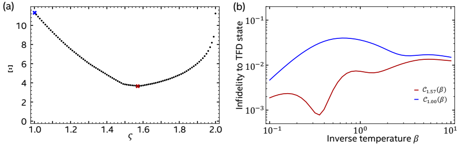
Figure 5.1: Optimization of the cost function. (a) Plot of \Xi versus \varsigma . The minimum of \Xi is found near \varsigma = 1.57 , indicating the closest match between optimized states and ideal TFD states across the range of \beta considered. (b) Simulated infidelity to the ideal TFD state of states optimized using the cost function \mathcal{C}_{1.00} (blue) and the optimized cost function \mathcal{C}_{1.57} (red).
