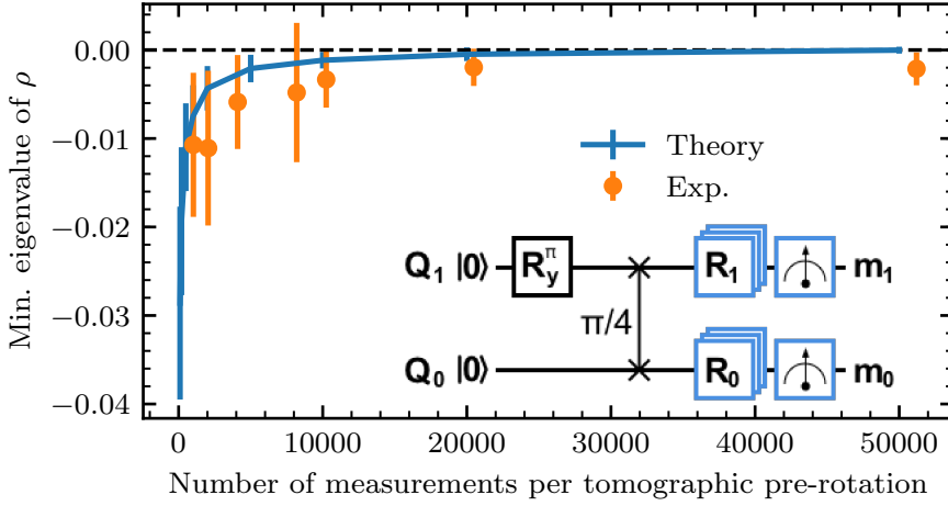
Figure 4.9: Minimal eigenvalue of density matrices obtained from linear tomographic reconstruction with different N_{\text{meas}} . Here, the state preparation targets a Bell state using our variational ansatz (inset) with \theta = \pi/4 (producing a \sqrt{\text{iSWAP}} gate). Physicality constraints on density matrices restrict their eigenvalues to be non-negative. We observe negative minimum eigenvalues over the entire range of N_{\text{meas}} . A quantumsim simulation produces a similar trend, asymptoting to a physical state by N_{\text{meas}} \sim 50,000 .
