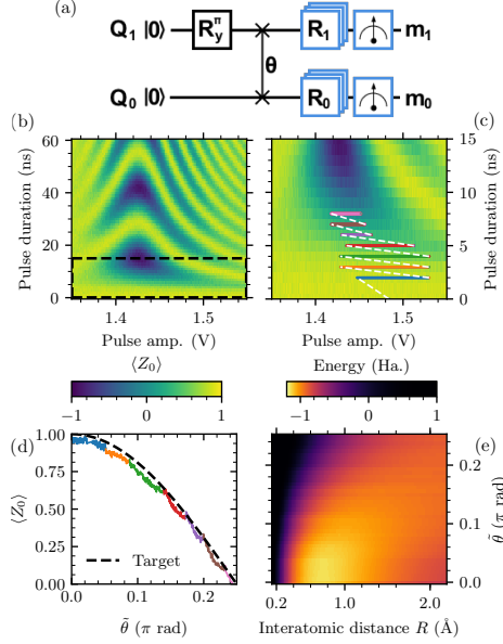
Figure 4.1: Quantum circuit and energy landscape of the variational eigensolver. (a) Quantum circuit for generating and measuring the variational ansatz state. (b) Coherent excitation exchange, produced as Q_0 is fluxed into resonance with Q_1 by a square flux pulse of fixed amplitude ( x axis) and duration ( y axis). The amplitude controls the frequency to which Q_0 is pulsed ( \sim 1.428 V bringing it on resonance with Q_1 ). (c) Zoom-in of (b) into the region used in the experiment to control the exchange of population between Q_0 and Q_1 . Colored lines illustrate the combinations of square-pulse amplitudes and duration used to achieve fine adjustment of \tilde{\theta} . (d) Excitation of Q_0 for the combinations of pulse amplitudes and duration marked by colored lines in (c), showing the matching of the experimentally-defined \tilde{\theta} to the target \theta defined in Eq. (4.7) (black dashed curve). Colors [matching (c)] correspond to pulse duration. (e) Landscape of energies E^{(raw)}(\tilde{\theta}, R) as a function of the experimentally-defined \tilde{\theta} angle and the interatomic distance R .
