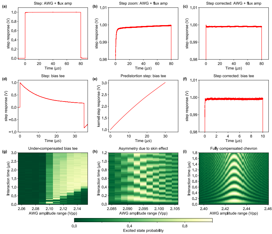
Figure 3.10: Calibration of the flux distortions. (a,b) Step response of the amplified AWG flux channel output with a zoom in (b), measured using a fast oscilloscope. (c) Corrected step response achieved using one linear response correction and three exponential decay corrections with parameters (\tau, \alpha) : (5.1\mu\text{s}, 0.0012) , (670\text{ns}, 0.015) and (520\text{ns}, -0.00037) (see text for details). (d, e) Measured step response (d) and numerically calculated predistortion step response (e) after the bias-tee. (f) Corrected step response achieved using a quadratic bias tee correction (see text for details). (g) Distorted flux “chevron” measured with the corrections applied in (e). (h) Dramatically improved chevron obtained after sweeping one parameter in the bias-tee correction (that corresponding to the standard RC time constant). The asymmetric signature observed here is characteristic of the low-pass filtering effect produced by the skin effect in the coaxial cables. (i) A well-compensated chevron obtained after applying a correction for the skin effect and several more exponential decay corrections with (\tau, \alpha) : (350\text{ns}, -0.0063) , (600\text{ns}, -0.0037) , (1500\text{ns}, -0.002) , (100\text{ns}, -0.0017) and (30\text{ns}, 0.0036) .
