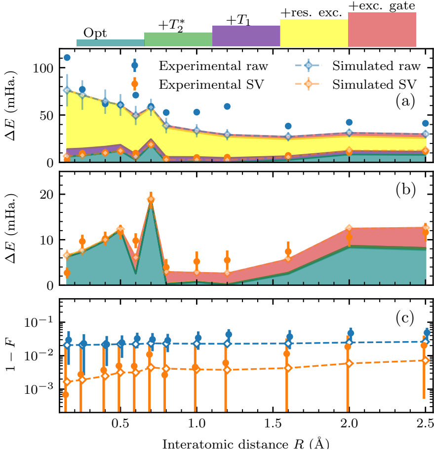
Figure 4.3: Impact of SV in ground-state energy and state fidelity, and dissected error budget. (a) Experimental (solid circles) energy error \Delta E without and with SV compared to the result (empty circles and dashed line) of a full density-matrix simulation using the full error model. The contributions from optimizer inaccuracy, qubit dephasing, qubit relaxation, residual qubit excitations and increased Q_0 dephasing during the exchange gate are shown as shaded regions for the case of no SV applied. Without SV, \Delta E is clearly dominated by residual qubit excitation. (b) Zoom-in on experimental and simulated \Delta E with SV and corresponding error budget. With SV, the effects of residual excitation and qubit relaxation are successfully mitigated, as predicted in Ref. [57]. The remaining energy error is dominated by optimizer inaccuracy. Simulation error bars are obtained by modelling measured fluctuations of T_1 , T_2^* , and residual excitation. (c) Experimental (solid circles with error bars) infidelity to the true ground state without and with SV compared to simulation using the full error model (empty circles and dashed line). Error bars are propagated through the linear inversion procedure for experiment and calculated from sampling noise for simulations. For simulations, error bars are smaller than the markers.
