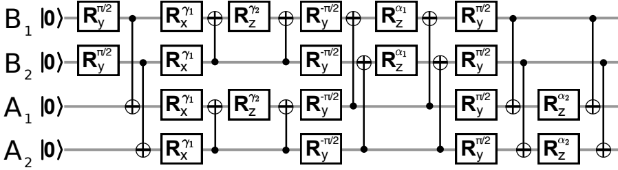
Figure 5.4: Compilation step 1. Depth-14 circuit obtained by replacing the ZZ and XX exponentiation steps in Fig. 1(b) with the circuits of Figure 5.3.
