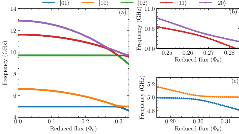
Figure 2.4: Two Qubit gates. (a) Spectrum for two transmons at typical frequencies (5 GHz and 6.6 GHz), with E_C = 300 MHz, connected to a common bus with qubit-qubit coupling J_1 = 30 MHz. (b) Zoom in on the avoided crossing of levels |20\rangle and |11\rangle , working area of the CZ gate. (c) Zoom in on the avoided crossing of levels |01\rangle and |10\rangle , working area of the \sqrt{i} SWAP gate.
