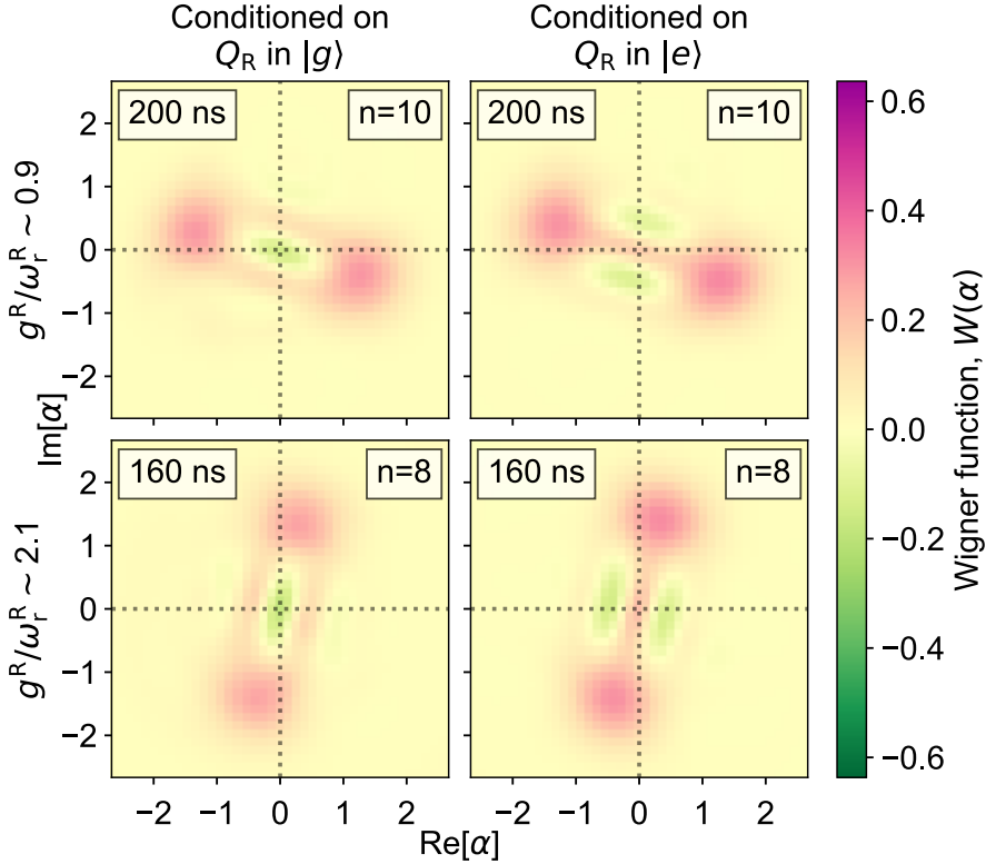
Figure 3.5: Nonclassical resonator cat states from conditioned DSC-driven entanglement (degenerate-qubit case). The plots show Wigner functions of nonclassical Schrödinger cat states in the Rabi resonator, reconstructed from maximum-likelihood state tomography for two different DSC coupling strengths with g^R/\omega_r^R \sim 0.9 (top, n = 10 Trotter steps) and g^R/\omega_r^R \sim 2.1 (bottom, n = 8 Trotter steps), conditioned on measuring Q_R in |0\rangle (left) and |1\rangle (right). The regions of negativity and visibility of several fringes between the well-resolved coherent state peaks are clear signatures of nonclassicality in the Rabi field mode and demonstrates the coherence and entanglement of the underlying qubit-resonator state. Combined with the qubit conditioning shown in Fig. 3.4, observing clear cat states for both outcomes of the Q_R measurement is a clear signature of coherent DSC dynamics.
