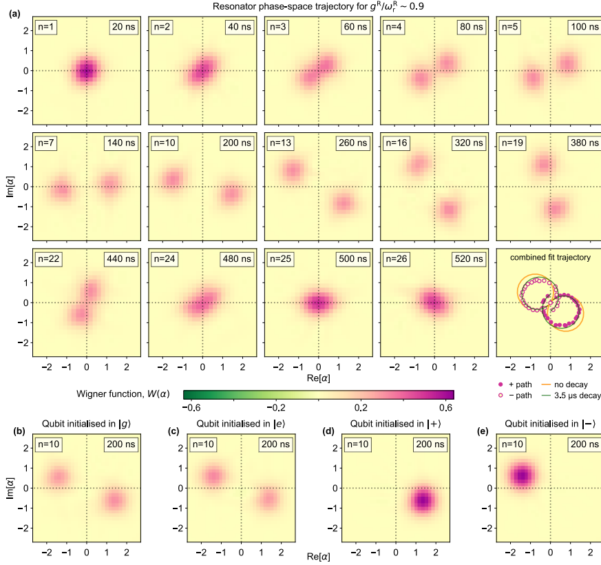
Figure 3.4: Photon dynamics in phase space in the DSC regime (degenerate-qubit case) from maximum-likelihood Wigner tomography. (a) Selected frames from a “movie” (measured over \sim 40 hours) showing the phase-space evolution of the resonator reduced state for r \sim 0.9 (frames labelled by Trotter step n and simulated time), with the final panel showing the full trajectories determined from 2D double-Gaussian fits to the raw data [the full movie is provided in the Supplementary Movie 1 of the published work]. Plotted tomograms are maximum-likelihood reconstructions of direct Wigner tomography measured data with a systematic phase correction [see Methods]. When the effective drive on the intracavity field created by the Rabi interaction has a strength comparable to the resonator’s natural frequency (i.e., g^R \sim \omega_f^R ), this drive is able to create a significant displacement of the cavity field before the phase-space rotation caused by \omega_f^R brings the field back towards the origin. This effect is observed clearly here in the creation of two well-resolved, rotating peaks and subsequent re-coalescence which are characteristic signatures of DSC dynamics. Deviation from the ideal circular trajectories (orange curves) arises from photon decay. The measured trajectory shows excellent agreement with a numerical Trotter simulation at g^R/2\pi = 1.79 MHz which includes resonator T_1, r = 3.5 \mu\text{s} (green curves). From the fits, we calculate an estimated Wigner function width \sigma = 0.526 \pm 0.003 , instead of the predicted 0.5, indicating a displacement calibration error of \sim 5\% [Supplementary Note 6]. Background noise arises from phase instability of microwave sources and frequency stability of the Wigner qubit over the long measurement. (b-e) Conditional phase-space evolution illustrated by the resonator Wigner function for different initial states of Q_R : (b) |0\rangle , (c) |1\rangle , (d) |+\rangle and (e) |-\rangle . The phase-space trajectory of R_R depends on the qubit state in the \sigma_x basis, consistent with creation of Bell-
