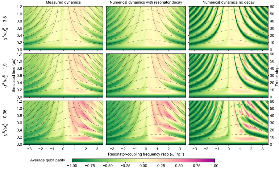
Figure 3.6: Measured and numerical quantum Rabi model qubit dynamics for nondegenerate qubit frequency. The cases implemented are g^R/\omega_q^R \sim 4 (top), \sim 2 (middle) and \sim 1 (bottom), with the plots showing measured qubit dynamics (left), numerically simulated dynamics of a Trotterised QRM with the measured T_{1,r} \sim 3.5 \mu\text{s} included (centre), and ideal Rabi dynamics (right). The results illustrate that the nondegenerate-qubit dynamics do not deviate significantly from the degenerate-qubit case in the regime where \omega_r^R \gg \omega_q^R . The measured dynamics exhibit many qualitative features in good agreement with the ideal QRM and show excellent agreement with the numerical Trotter simulation with decay, indicating that the fidelity of the measured results to the ideal case is limited primarily by resonator decay.
