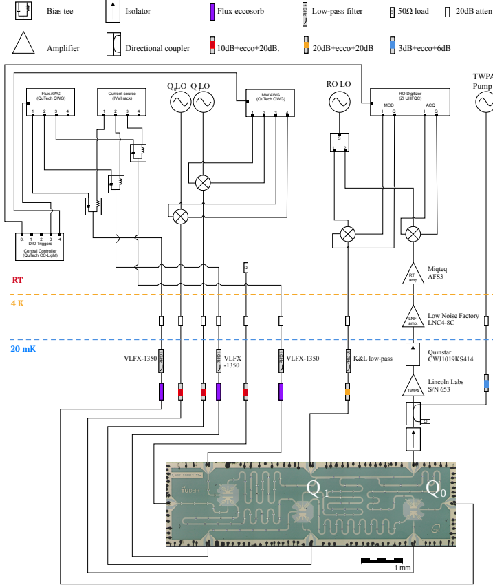
Figure 4.5: Device and wiring schematic. The 2\text{ mm} \times 7\text{ mm} chip contains three Starmon [46] qubits. Qubit pairs Q_0 - Q_1 and Q_1 - Q_2 are coupled by bus resonators. Qubits have dedicated microwave drive lines, flux bias lines, and dispersively-coupled readout resonators. Readout resonators are coupled to a common feedline allowing independent qubit readout by frequency multiplexing. See text for details of cryogenic system and wiring. In this experiment, we only make use of Q_0 and Q_1 . The unused leftmost qubit, Q_2 , is parked at its sweetspot frequency (4.128 GHz) throughout.
