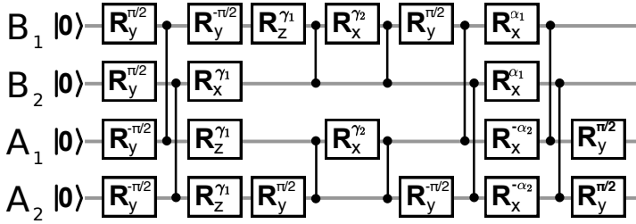
Figure 5.8: Compilation step 3. Depth-12 circuit obtained by applying the commutation rule in Figure 5.7 and simple identities to the circuit of Figure 5.6.
