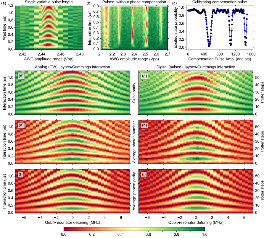
Figure 3.13: Comparison of analog and digital versions of a Jaynes-Cummings interaction. (a) Standard analog JC chevron showing the resonant excitation swapping between qubit and resonator after the qubit is initialised in the excited state as a function of flux-pulse amplitude ( x axis) and duration ( y axis) (qubit-resonator detuning and interaction time, respectively). The x -axis location of the chevron ( \sim 2.445 Vpp) therefore defines the qubit-resonator on-resonance condition. (b) Digital JC chevron (measured under otherwise identical conditions) using a pulse duration of 20 ns showing a series of equally spaced resonances with different apparent interaction strengths. (c) We scan amplitude of a 5 ns compensation flux pulse to identify the value which enforces that the digital chevron is centred around the natural resonance position. (d-f) Standard analog and (g-i) digital JC chevrons measured by probing: (d, g) the excited state probability for Q_R , (e, h) the average photon number in R_R (linear range 0–2 photons), and (f, i) the photon parity of R_R .
