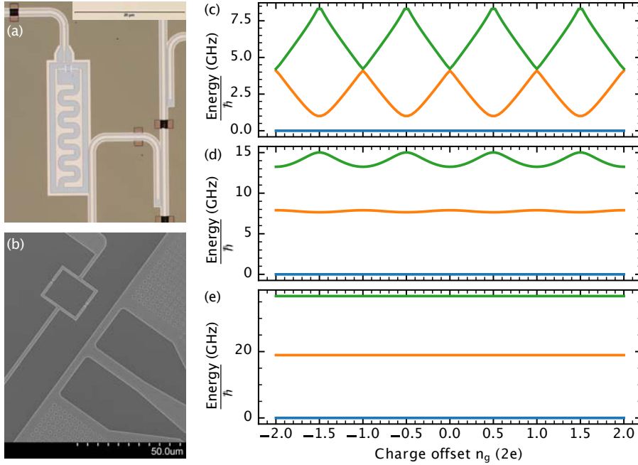
Figure 2.1: The Transmon qubit. (a) Optical micrograph of a Transmon qubit, defined by a shunting interdigitated capacitor and a SQUID loop (top of the capacitor). The qubit couples capacitively to a CPW resonator on its bottom-right end. A flux-bias line couples inductively to the SQUID loop on the top. All the surfaces are made of NbTiN on top of a Si substrate, except for the JJs and airbridges (stitch-like structures on top of CPW lines), which are made of Al. (b) SEM picture of a similar device centered on the SQUID loop. The JJs are evaporated on top of the square pattern defining the SQUID. The flux-bias line is placed assymmetrically, in order for its current to affect the magnetic flux threading inside the SQUID loop. (c-d) The first three energy levels of a transmon qubit for \frac{E_C}{\hbar} = 1 GHz and (c) \frac{E_J}{\hbar} = 1 GHz, (d) \frac{E_J}{\hbar} = 10 GHz and (e) \frac{E_J}{\hbar} = 50 GHz. As E_J/E_C increases, the spectrum dependence on n_g decreases exponentially. The qubit transitions frequencies are set by the difference between these energy levels.
