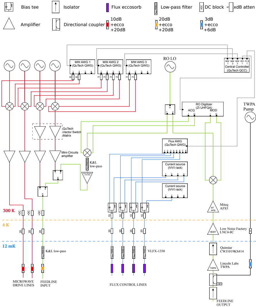
Figure 5.11: Fridge wiring and electronic setup.
