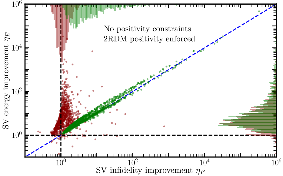
Figure 4.4: Constraining positivity with symmetry verification to mitigate the effect of sampling noise. The experimental data from Fig. 4.3 is split into 100 sample simulations for each R , increasing the sampling noise by a factor of 10 and making it comparable to other sources of experimental error. For each sample, we plot (red) the relative energy error and infidelity [Eq. (4.9)]. Values below 1 (dashed lines) indicate that SV has not provided an improvement, as may be the case when the density matrix has negative eigenvalues. We restore the improvement from SV by constraining the positivity of the 2-reduced density matrix [148] (green). Histograms on the top and right axes show the marginal distribution of the two scatter plots. When the density matrices are constrained to be positive, we observe the points fall along the line y = x (blue dashed line), indicating that SV improves both metrics by the same amount.
