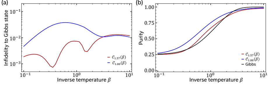
Figure 5.2: Cost function performance comparison. (a) Simulated infidelity of the reduced state of system A to the Gibbs state for states optimized using the cost function C_{1.00} (blue) and the optimized cost function C_{1.57} (red). (b) Corresponding purity of the reduced state. The purity of the Gibbs state is also shown for comparison (black).
