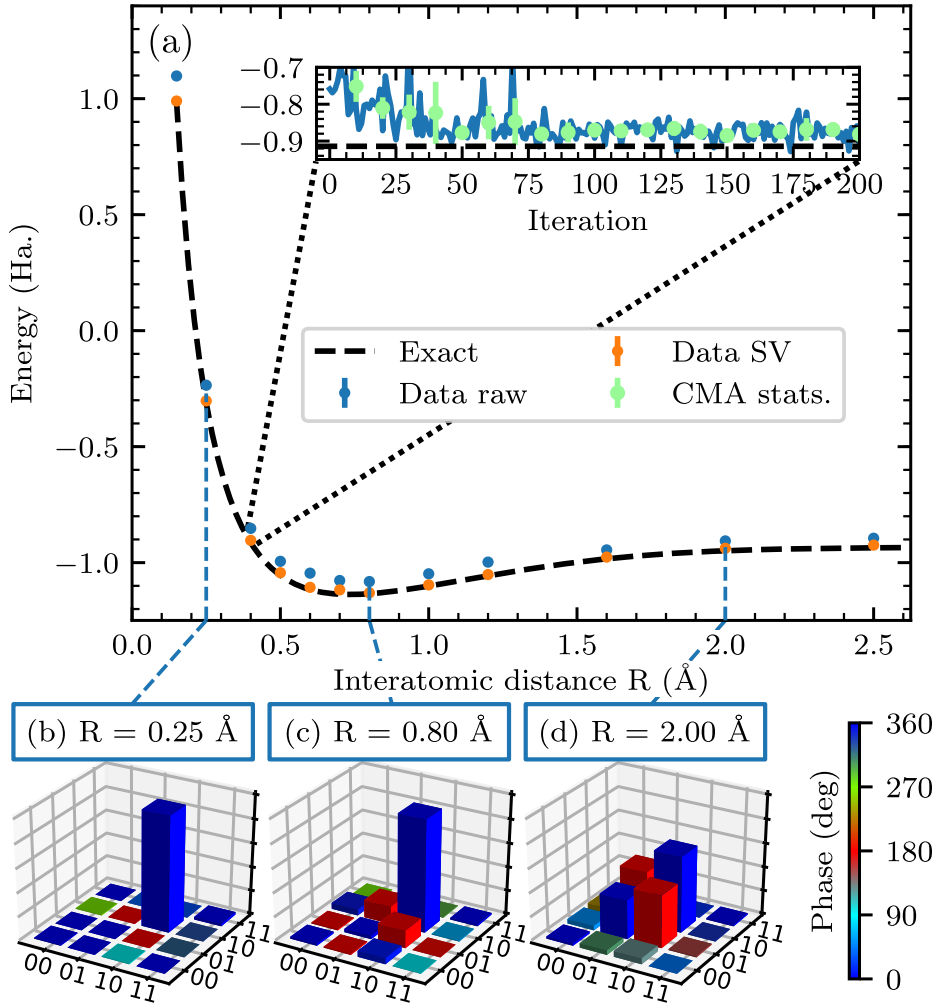
Figure 4.2: Convergence of the VQE algorithm. (a) Experimental VQE estimate of H_2 ground-state energy as a function of interatomic distance R . At each chosen R , we minimize the raw energy E^{(raw)} (blue data points) over the variational parameter \tilde{\theta} using the CMA-ES evolutionary algorithm [145]. Applying SV to the converged solution (orange data points) lowers the energy estimate towards the exact solution (dashed curve). Inset: A typical optimization trace for the convergence of the energy estimate. (b-d) The reconstructed density matrices of the converged states at (b) R = 0.25 Å, (c) R = 0.80 Å, and (d) R = 2.00 Å, showing that the converged states lie mostly in the single-excitation subspace, and that entanglement increases with the interatomic distance R .
