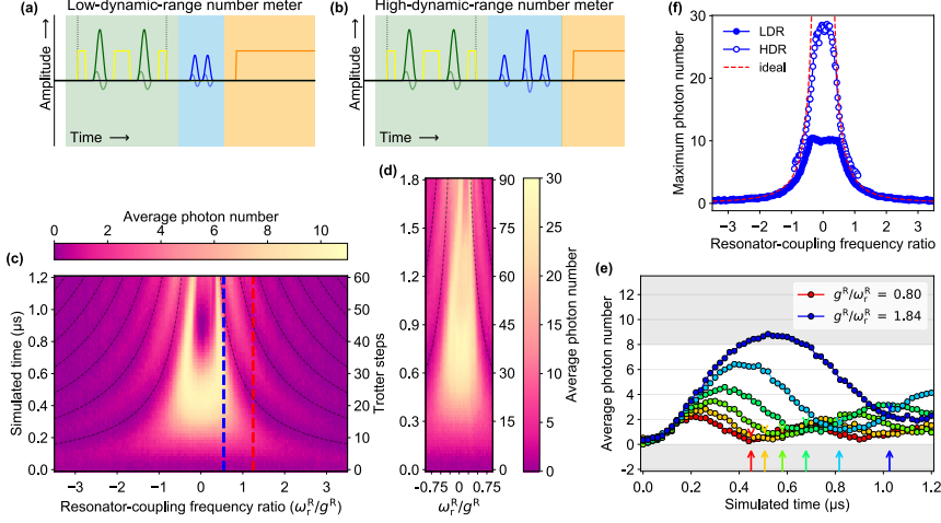
Figure 3.3: Photon number dynamics of the quantum Rabi model in the degenerate-qubit case. (a, b) Average photon number is probed by applying Ramsey and echo-like pulses to Q_W . The effective Ramsey pulse separation \tau determines the photon dynamic range. Because of finite pulse widths, reaching the small \tau needed for high dynamic ranges (b) requires an unbalanced “echo”-like sequence. (c, e) Measured photon number dynamics up to 60 Trotter steps using a low-dynamic-range (LDR) photon number meter ( \tau \sim 18.7 ns) with a linear range of \sim 0 –8 photons [indicated by grey regions in (e)]. Large photon populations in the resonator highlight the non-conservation of excitation number in the quantum Rabi model. The resonator displays clear oscillations up to r > 1.8 in good agreement with the expected qubit revival times (dashed curves). The red feature in the middle reflects the upper limit on the number meter’s dynamic range set by Q_W “population wrapping” at high photon numbers. (d) Measured photon dynamics up to 90 Trotter steps using a high-dynamic-range (HDR) number meter with \tau \sim 6.5 ns and a linear range of \sim 0 –20 photons, allowing observation of photon oscillations beyond 1.5 \mu s of simulated time (more than 75 Trotter steps). This data shows the effect of a residual Kerr nonlinearity at high values of r . (e) Line slices are plotted for evenly spaced resonator-coupling frequency ratios between the red and blue dashed lines shown in (c). Grey regions delineate the linear range of the number meter. (f) Maximum measured average photon number for each value of r for both LDR and HDR number meters.
