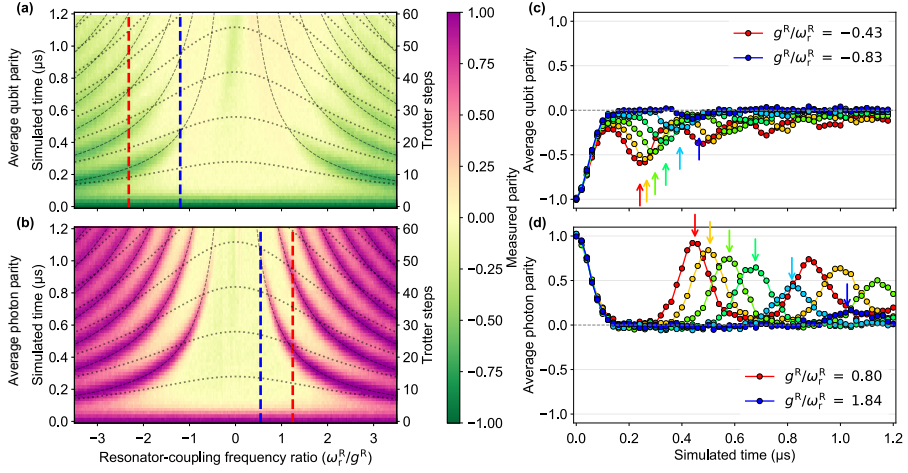
Figure 3.2: Qubit and resonator parity dynamics of the quantum Rabi model in the degenerate-qubit case. Measured dynamical landscapes for (a) qubit and (b) photon parity dynamics for a broad range of parameters up to 60 Trotter steps, with the extreme DSC regime in the centre decreasing to weaker USC near the edges. The data show clear Gaussian-shaped collapses for all r , along with the characteristic plateaus of DSC. Qubit revivals are observed up to r \sim 0.8 , while photon parity shows clear revivals up to r \sim 1.8 . Vertical line cuts for (c) qubit and (d) photon parity are plotted for evenly spaced \omega_r^R/g^R between the red and blue dashed lines in (a) and (b), respectively. For r \gtrsim 1.5 , some deviation from the expected revival time in the photon parity results from a small residual Kerr-type nonlinearity in the resonator [see also Supplementary Fig. 9] and is correlated with significant photon populations. Arrows in (c) and (d) show expected revival times for each slice. In this and following figures, coupling ratios were calculated using the observed simulated coupling of g/2\pi = 1.79 MHz.
