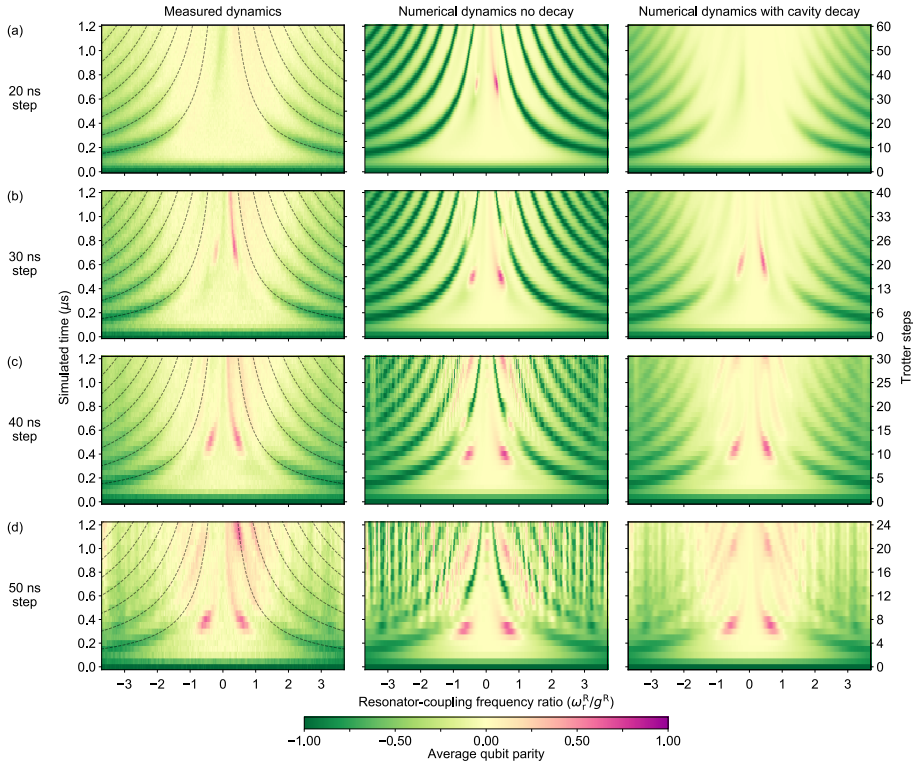
Figure 3.16: Comparison of simulation performance for various Trotter step sizes, showing measurements (left), numerical simulations with no decay (middle) and numerical simulations with the measured T_{1,r} = 3.5\mu\text{s} : (a) 20 ns steps (60 Trotter steps), (b) 30 ns steps (40 Trotter steps), (c) 40 ns steps (30 Trotter steps) and (d) 50 ns steps (24 Trotter steps).
