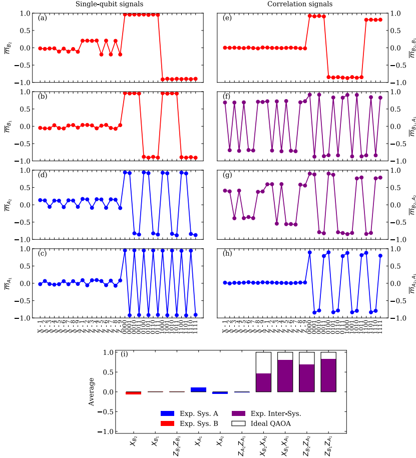
Figure 5.15: Example raw data for evaluating the cost function with variational angles (\vec{\alpha}, \vec{\gamma}) = 0 . Experimental average (from 4096 shots) of single-qubit and correlation measurements for the 18 measurement bases in Table 5.1 and for calibration of the measurement operators (following preparation of the 16 computational states of the four transmons). Panels show the experimental averages of (a-d) single-transmon measurements, (e,h) intra-system correlations and (f,g) inter-system correlations. (i) Bar graph of the experimental estimate of the expected values of all terms in \mathcal{C} , obtained by linear inversion on the measurement averages. For comparison, we also show are the expected values of all the terms for an ideal processor.
