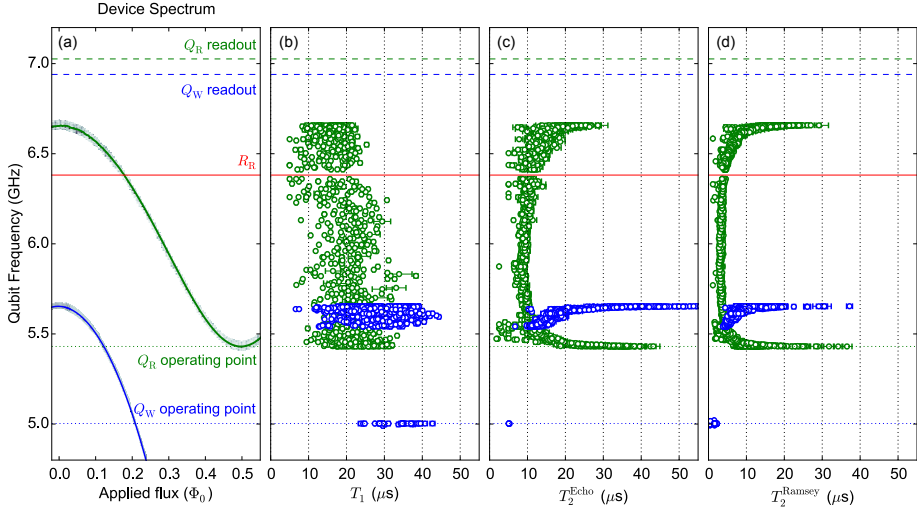
Figure 3.9: Schematic showing measured spectral arrangement for the digital Rabi quantum simulator device and the qubit coherence times. (a) Measured data for the 0–1 transition of the Rabi qubit Q_R (green curve) and the Wigner qubit Q_W (blue curve) are plotted as a function of applied flux in units of \Phi_0 . Also shown are the frequencies of the Rabi resonator R_R (red: \omega_r = 6.381\text{GHz} ) and the readout resonators for Q_R (green dashed: \sim 7.03\text{GHz} ) and Q_W (blue dashed: \sim 6.94\text{GHz} ). The operating points of the qubits for the Trotter simulation are given by the green and blue dotted lines for Q_R and Q_W , respectively. (b, c, d) Time constants measured for Q_R (green) and Q_W (blue) for (b) T_1 , (c) T_2^{\text{echo}} and (d) T_2^* . Note that, at the sweet spots, measured qubit T_2^* times here are limited by slow frequency-switching processes in the qubits such as quasiparticle tunnelling [15].
