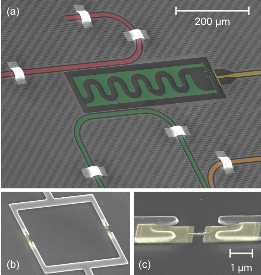
Figure 3.8: SEM images of a sister device with added false colour. (a) Rabi qubit ( Q_R ) with coupling to the Rabi resonator ( R_R , above) and readout resonator (below), showing the centred flux-bias line and displaced SQUID loop. Q_R is coupled to R_R near its shorted end in order to achieve the required small coupling g . (b, c) Josephson junctions are contacted to the NbTiN SQUID loop fingers using small bays to achieve better contact. In (b), it is possible to see the large asymmetry in junction size, with a zoom on the small junction in (c).
