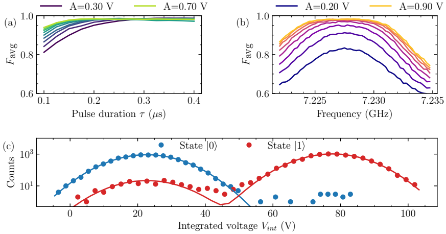
Figure 2.2: Readout control (a) Average assignment fidelity \mathcal{F}_a as a function of readout pulse duration \tau for different readout pulse amplitudes A . \mathcal{F}_a increases monotonically as amplitude or pulse improve, until a point of maximal fidelity where \mathcal{F}_a starts worsening with increasing \tau (see yellow curve) (b) Average assignment fidelity \mathcal{F}_a as a function of readout pulse frequency for different readout pulse amplitudes A . \mathcal{F}_a is maximal around a specific frequency. (c) Histograms for the signal V_{int} integrated after preparing the qubit in the states |0\rangle and |1\rangle . Solid lines correspond to gaussians fit centered at voltage V_0 and V_1 for each state.
