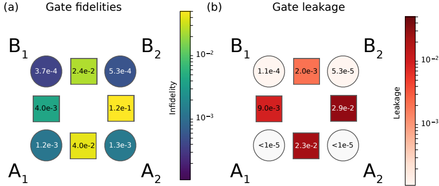
Figure 5.12: Single- and two-qubit gate performance. (a) Infidelity and (b) leakage of single-qubit gates (circles) and CZ gates (squares), extracted by randomized benchmarking.
