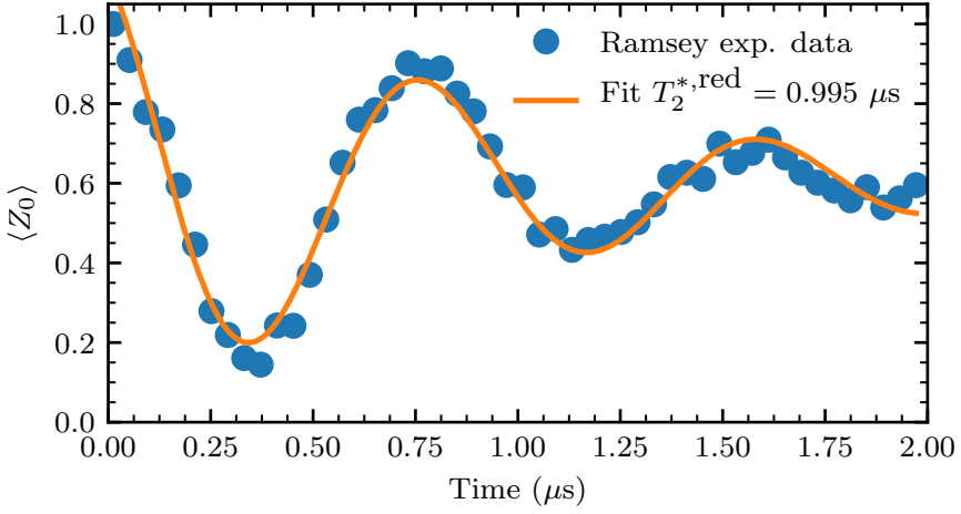
Figure 4.6: Ramsey experiment with qubit Q_0 DC-flux biased to the frequency of the resonant exchange interaction (5.1468 GHz, the Q_1 sweetspot frequency), but with qubit Q_1 biased away to a lower frequency. The best fit value T_2^{*,\text{red}} = 0.995 \mu\text{s} is used for modelling the increased dephasing of Q_0 during the exchange gate.
