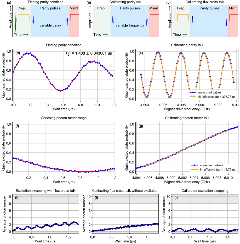
Figure 3.11: Calibration of the photon meter. (a–c) Measurement sequences used for calibrating the parity meter, specifically: (a) the dispersive shift of R_R on Q_W , (b) the effective delay time \tau corresponding to a particular pulse separation, and (c) high-frequency flux cross-talk between flux pulses on Q_R and the flux offset of Q_W . (d) Calibrating the parity condition, identified as the first crossing point of a Ramsey experiment with one photon in the resonator, giving a pulse separation of 383 ns. (e) Calibrating the effective delay time \tau for a particular pulse separation. Using parity pulses separated by 383 ns, we calibrated the effective separation \tau to be 398 ns, corresponding to a dispersive shift 2\chi/2\pi = -1.26 MHz. (f) Configuring an average photon number meter for a specific dynamic range of 0–8 photons. Driving at the midpoint of the 0–8 photon frequency range, the Ramsey pulse separation is chosen to lie on the edge of the linear region. For 0–8 photons, we chose to use a separation of 4 ns. (g) Calibrating the photon meter effective \tau . Repeating the measurement described in (e), the effective pulse delay for a 4 ns separation was \sim 19 ns. Comparing the oscillation period of the curves in (e) and (g) highlights the different sensitivity of the two photon meters. (h–j) Calibrating high-frequency flux cross-talk. The flux cross-talk is calibrated by measuring the photon meter without loading excitations into the resonator and corrected by adjusting the phase of the second photon meter pulse.
