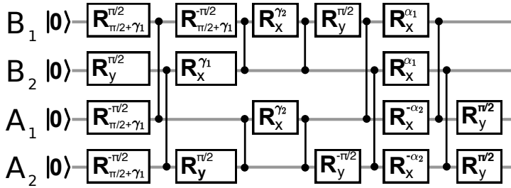
Figure 5.9: Compilation step 4. Depth-11 circuit obtained by propagating all R_Z gates in Figure 5.8 to the beginning of the circuit and then eliminating them.
