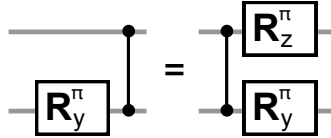
Figure 5.7: Commutation of R_Y(180^\circ) and CZ gates.
