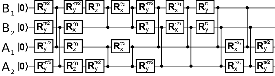
Figure 5.6: Compilation step 2. Depth-16 circuit obtained by replacing every CNOT in Figure 5.4 with the circuit of Figure 5.5 and using simple identities.
