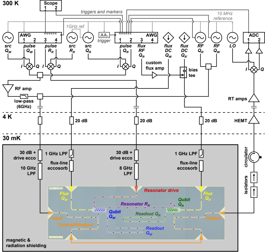
Figure 3.7: Experimental schematic showing the connectivity of microwave electronics and components in and outside the dilution refrigerator. The sample mounted below the mixing chamber typically remained at around 30 mK. Qubit and resonator drive lines and flux-bias lines were thermalised and attenuated at the 4 – K and 30 – mK stages and were low-pass filtered before arriving at the sample. The qubits and resonator drive pulses were generated by AWGs and IQ mixers. Home-built low-noise current sources provided DC bias currents for qubit frequency tuning, which were combined with fast frequency-tuning bias pulses using reactive bias tees. AWG markers provided the gating for pulse-modulated measurement pulses.
