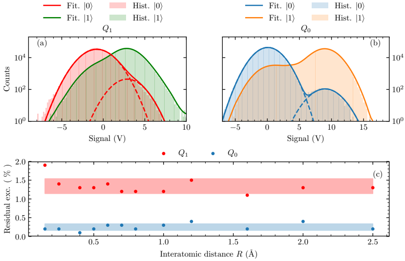
Figure 4.7: Residual qubit excitations. Single-shot readout histograms for (a) Q_1 and (b) Q_0 nominally prepared in |0\rangle and |1\rangle . We extract a residual qubit excitation from the best-fit double gaussian on the ground-state histogram (solid curves). (c) Residual excitations extracted from calibration data in the final, post-VQE-convergence in the dataset of Figs. 2 and 3 at each value of R . The average (standard deviation) of the residual excitation is 0.25% (0.09%) for Q_0 and 1.34% (0.20%) for Q_1 .
