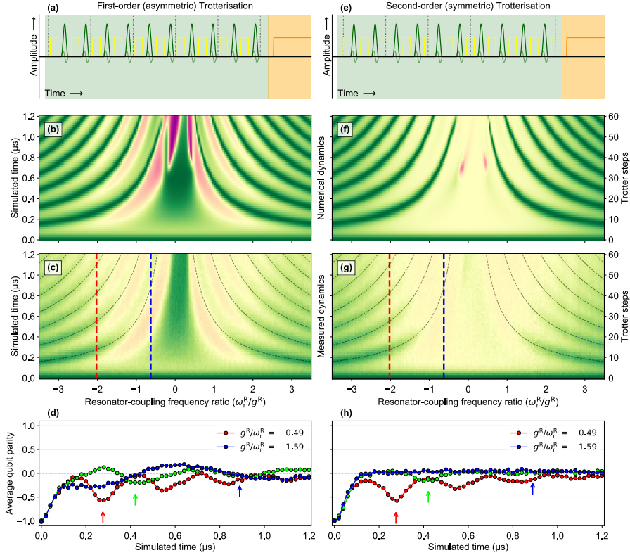
Figure 3.15: Comparison of simulation performance for asymmetric, first-order (a–d) and symmetric, second-order (e–h) Trotterisation. (a, e) Pulse sequences for the first-order (a) and second-order (e) Trotterisation. (b, f) Numerical simulations of the Trotterised Rabi model for the ideal case with no decay. Note that the sharp features in the centre of the plots (deep in the ultrastrong coupling regime) are not artifacts of the numerics, but Trotter error related to the 20 ns step size (these features disappear for 10 ns pulses). (c, g) Experimental quantum simulations for first-order (c) and second-order (g) Trotterisation, showing very good agreement with the numerical results in (b, f). (d, h) Vertical line slices are plotted for evenly spaced resonator frequencies between the red and blue dashed lines in plots (c) and (g).
