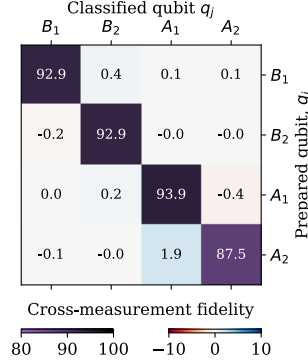
Figure 5.14: Measured readout cross-fidelity matrix.
