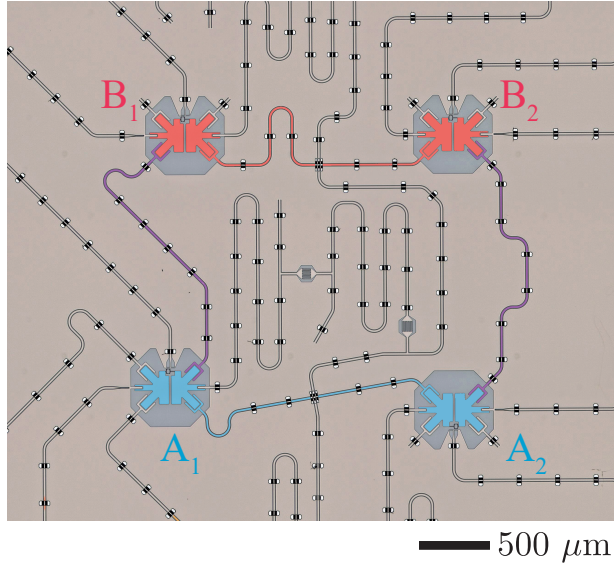
Figure 5.10: Optical image of the device, zoomed in to the four transmons used in the experiment. Added false color highlights the transmon pair of system A (blue, A 1 , A 2 ) the transmon pair of system B (red, B 1 , B 2 ), and the dedicated bus resonators used to achieve intra-system (read and blue) and inter-system coupling (purple).
