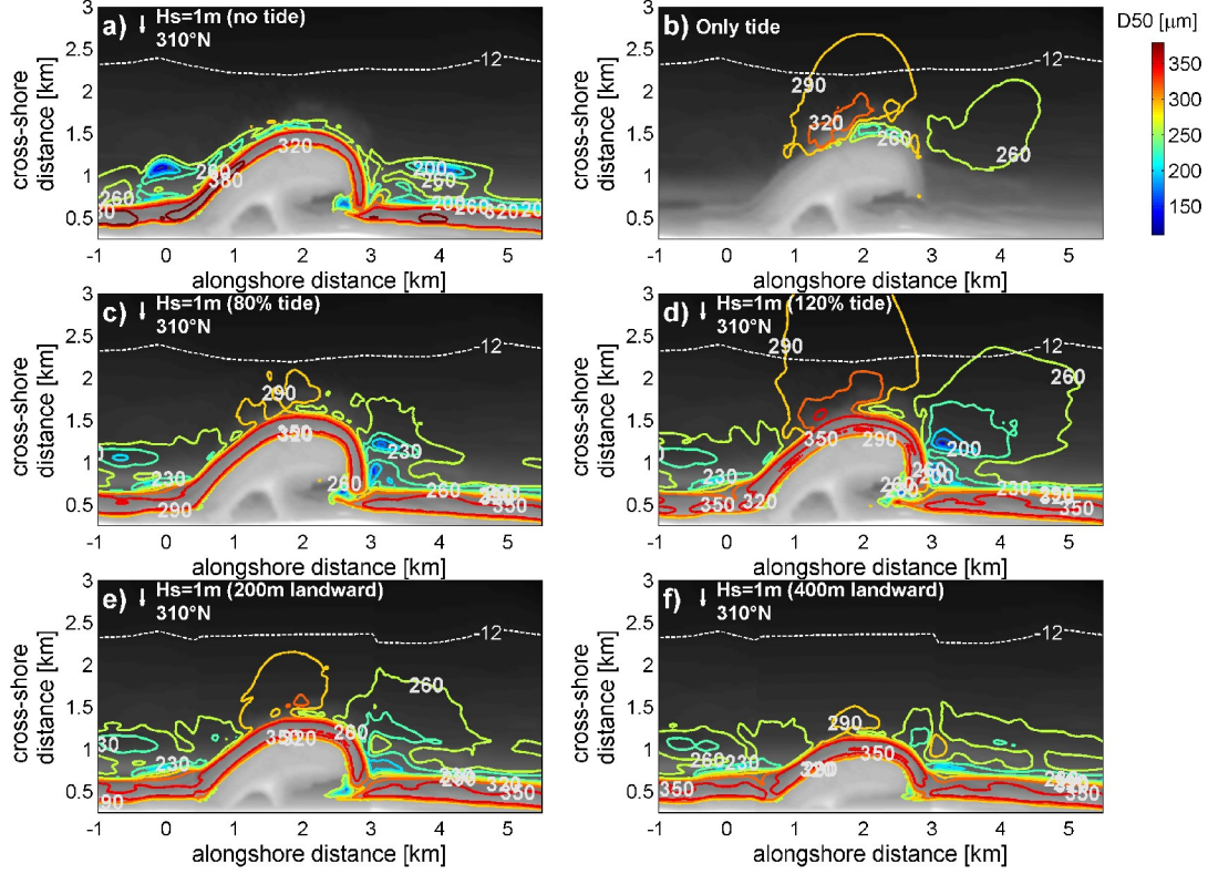
Figure 15: Modelled spatial pattern of D_{50} as a result of wave conditions ( H_{m0}=1\text{m} ), tide ( \Delta H \approx 1.5\text{m} and \bar{U} \approx 1\text{m/s} ) or adjustments of the bathymetry (affecting the tide and waves). a) Run C1 with only waves; b) Run C2 with only tide; c) Run C3 with 80% tidal velocities and moderate waves ( H_{m0}=1\text{m} ); d) Run C4 with 120% tidal velocities and moderate waves ( H_{m0}=1\text{m} ); e) Run B1 with 400 m landward shift of bathymetry ( H_{m0}=1\text{m} and 100% tide); f) Run B2 with 200 m landward shift ( H_{m0}=1\text{m} and 100% tide).
