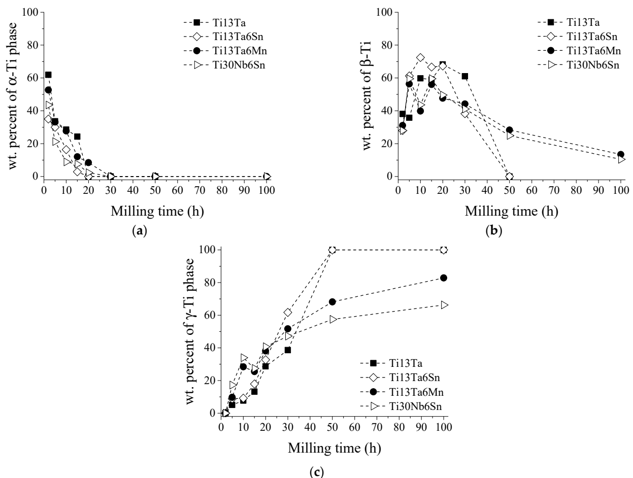
Figure 7. Phase evolution as a function of the milling time, (a) \alpha -Ti, (b) \beta -Ti, and (c) \gamma -Ti phase.
